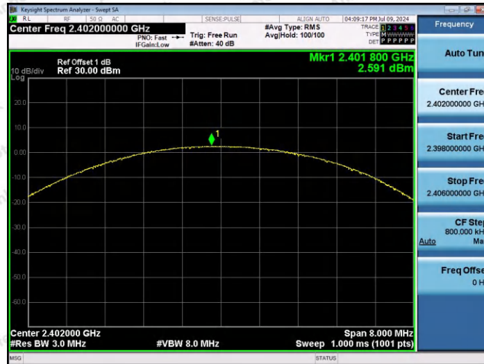
3DH5-Ant1-2402-PASS
