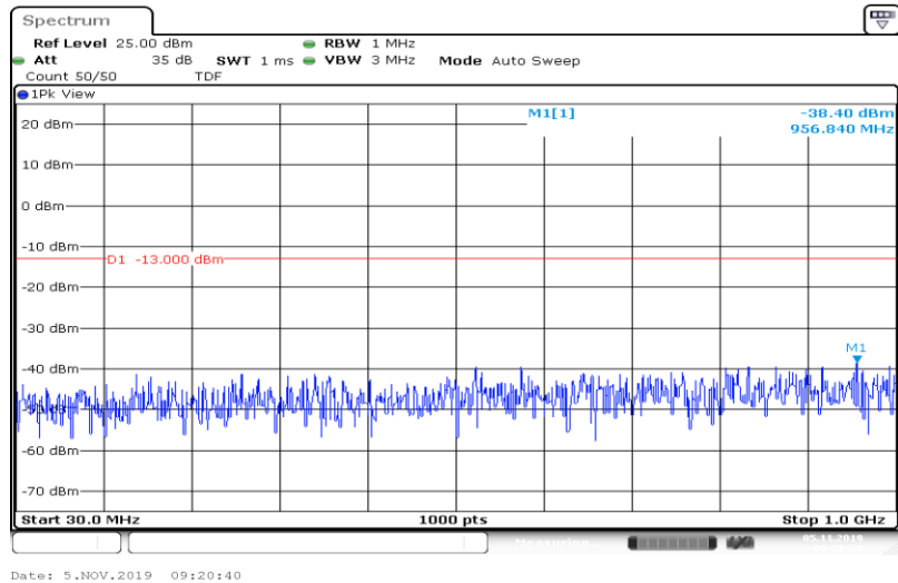
Band4-5MHz-16QAM-19975-25RB#0-Range4:1000~2000MHz
