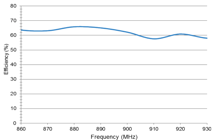
ISM Efficiency
