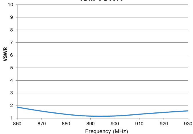
ISM VSWR
