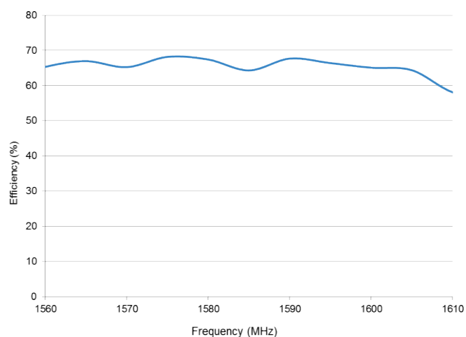
GPS Efficiency
