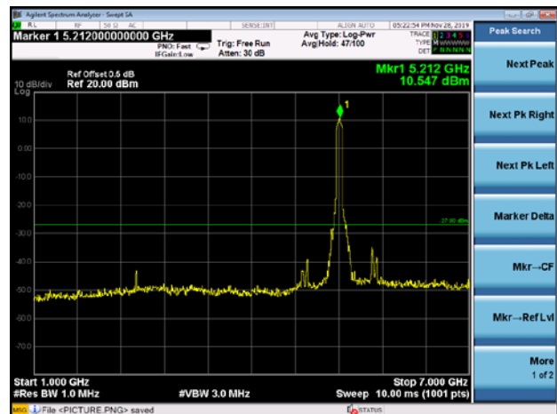
802.11 ac80 on channel 42
