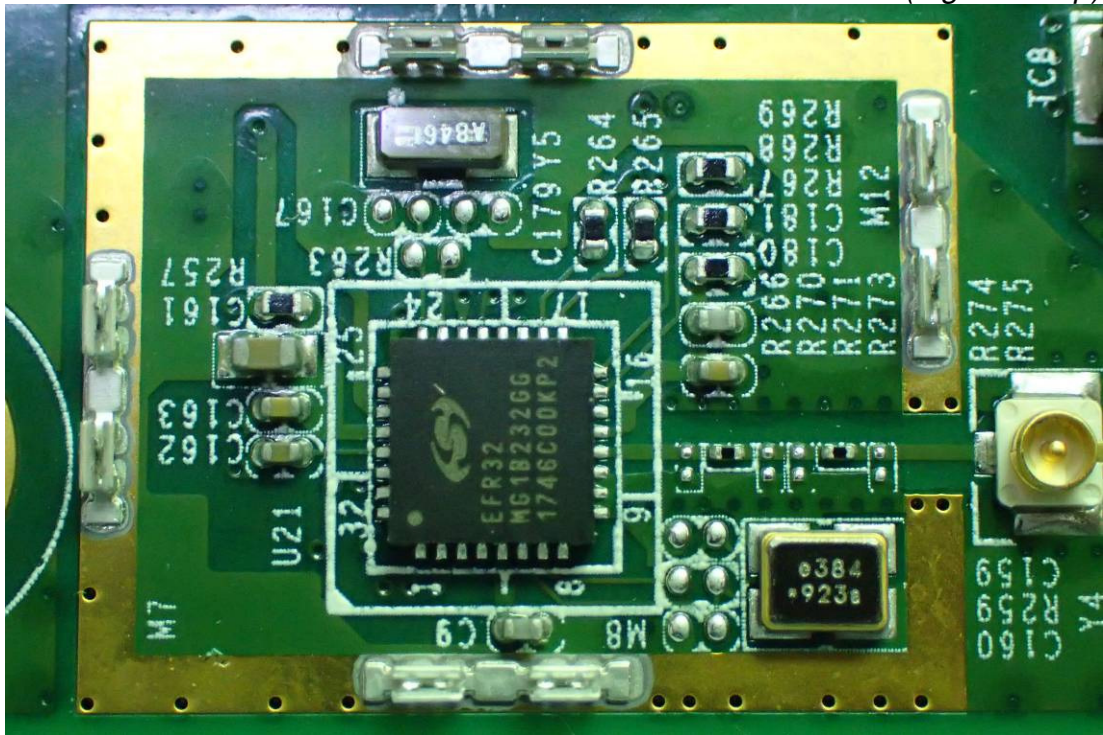
Figure 21 Internal View (ZigBee Chip)
