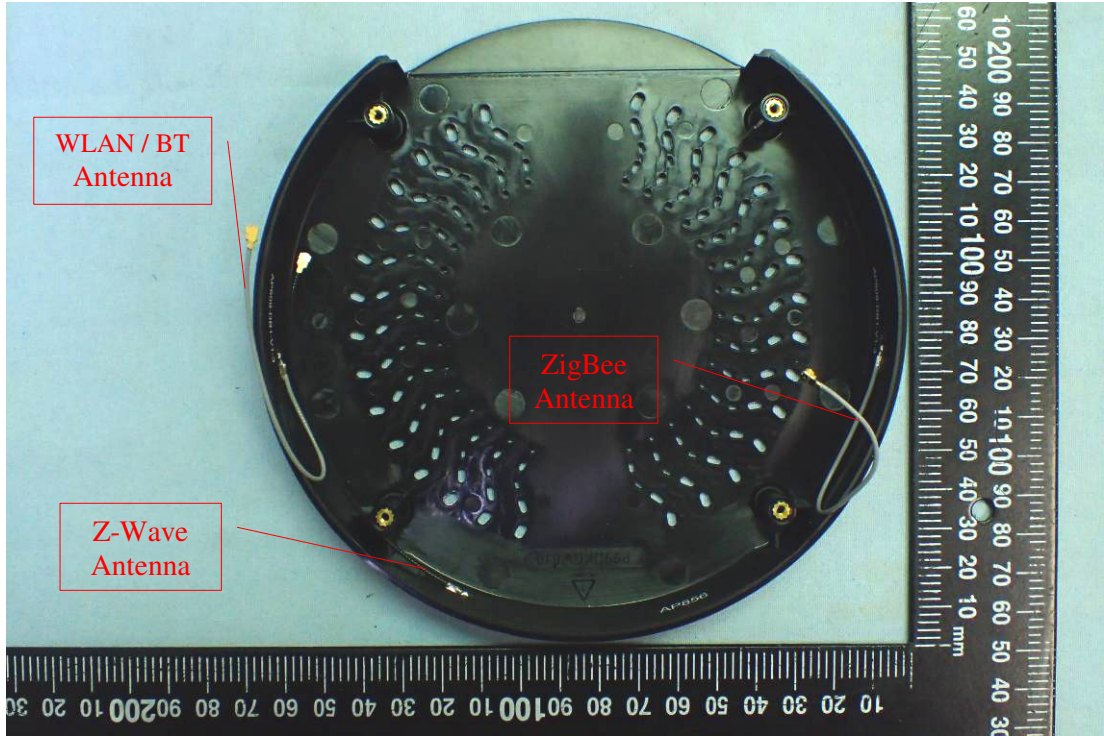
Figure 9 Internal View
