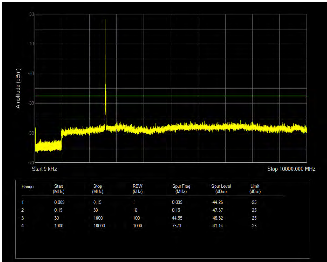
Band41 QPSK BW=15MHz Channel=40815 RB Size=75 Position=#0
