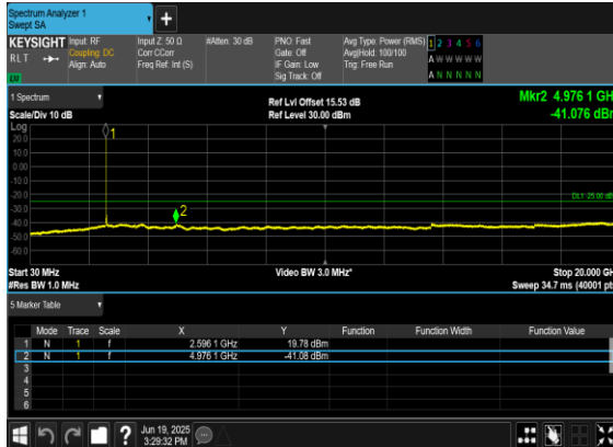
N38(25M)_DFT-s- OFDM_QPSK_Edge_1RB_Left_High_CH
