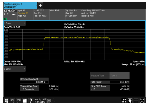
B7_N5(20M)_CP-OFDM_256 QAM_Outer_Full_Mid_CH
