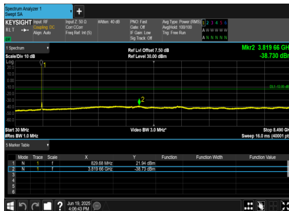
B7_N5(20M)_DFT-s- OFDM_QPSK_Edge_1RB_Left_High_CH
