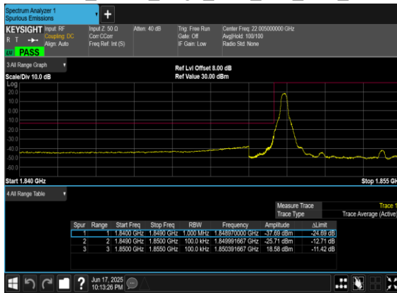
N2(10M)_DFT-s- OFDM_QPSK_Edge_1RB_Left_Low_CH
