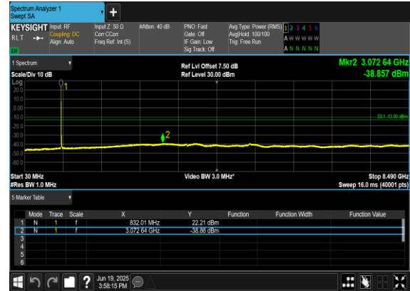
B7_N5(10M)_DFT-s- OFDM_QPSK_Edge_1RB_Left_Mid_CH
