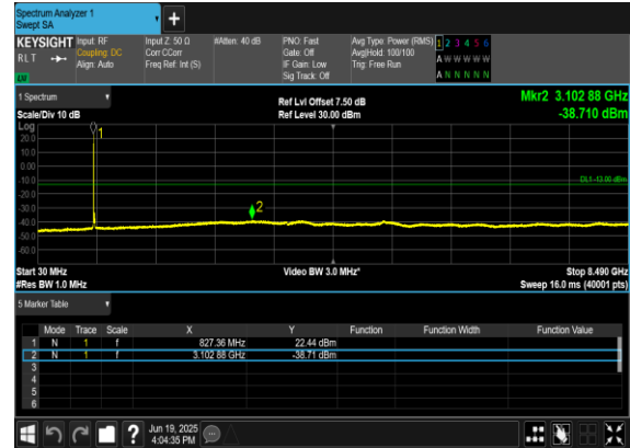
B7_N5(20M)_DFT-s- OFDM_QPSK_Edge_1RB_Left_Mid_CH
