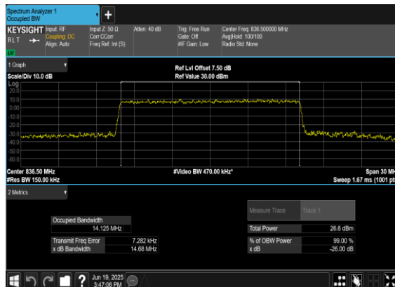
B7_N5(15M)_CP-OFDM_64 QAM_Outer_Full_Mid_CH
