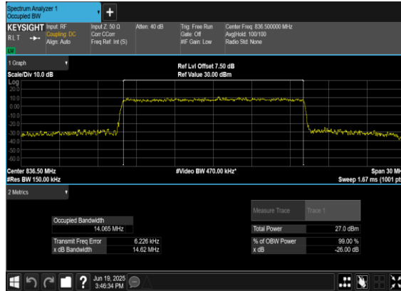
B7_N5(15M)_CP- OFDM_QPSK_Outer_Full_Mid_CH
