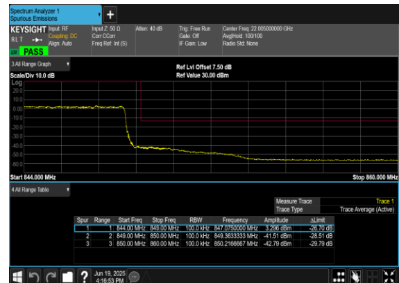
B7_N5(10M)_DFT-s- OFDM_QPSK_Outer_Full_High_CH
