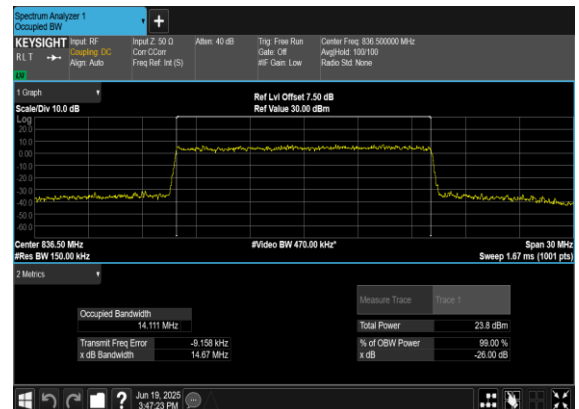
B7_N5(15M)_CP-OFDM_256 QAM_Outer_Full_Mid_CH
