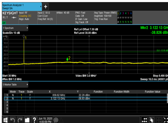
B7_N5(10M)_DFT-s- OFDM_QPSK_Edge_1RB_Left_High_CH
