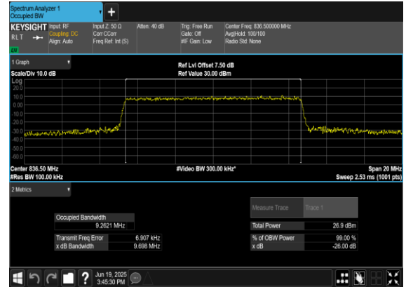
B7_N5(10M)_CP-OFDM_16 QAM_Outer_Full_Mid_CH
