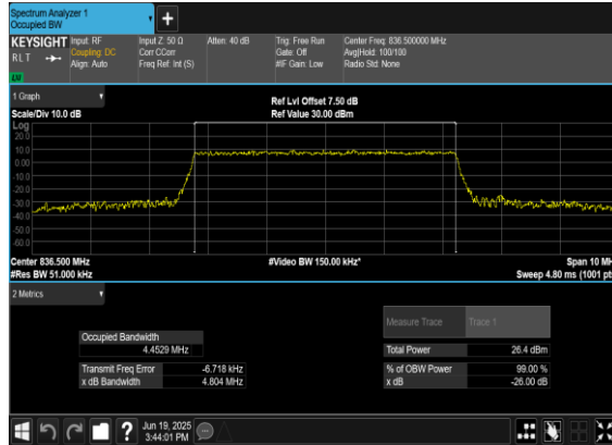
B7_N5(5M)_CP- OFDM_QPSK_Outer_Full_Mid_CH
