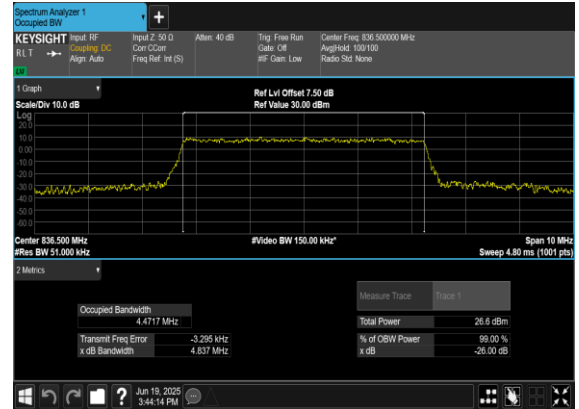
B7_N5(5M)_CP-OFDM_16 QAM_Outer_Full_Mid_CH
