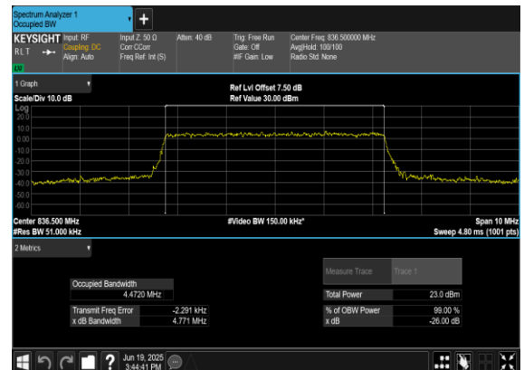
B7_N5(5M)_CP-OFDM_256 QAM_Outer_Full_Mid_CH
