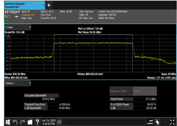
B7_N5(20M)_CP-OFDM_16 QAM_Outer_Full_Mid_CH
