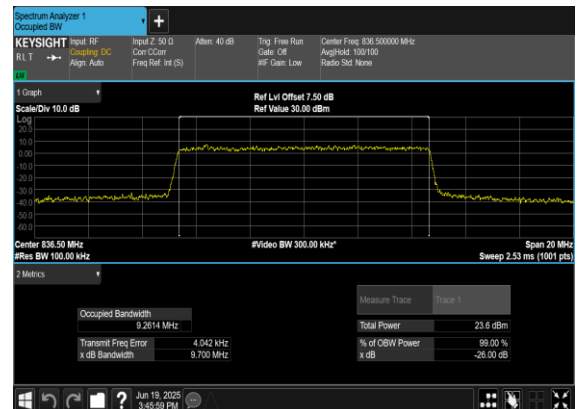
B7_N5(10M)_CP-OFDM_256 QAM_Outer_Full_Mid_CH
