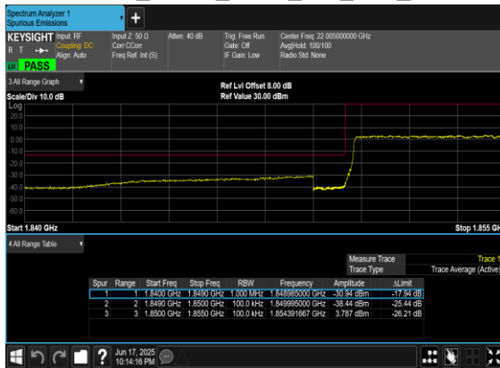
N2(10M)_DFT-s- OFDM_QPSK_Outer_Full_Low_CH
