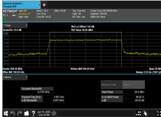
B7_N5(10M)_CP- OFDM_QPSK_Outer_Full_Mid_CH
