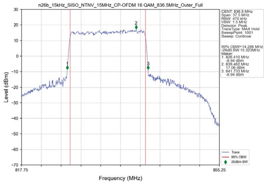
n26b 15kHz SISO NTN 15MHz CP-OFDM 16 QAM 836.5MHz Outer Full Ant0
