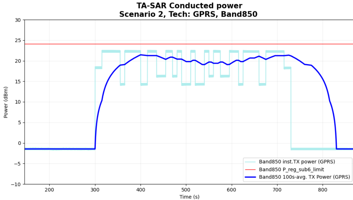
Figure 5-37 Time-averaged conducted TX power over time for case 10 (2G GPRS 850 2TX)
