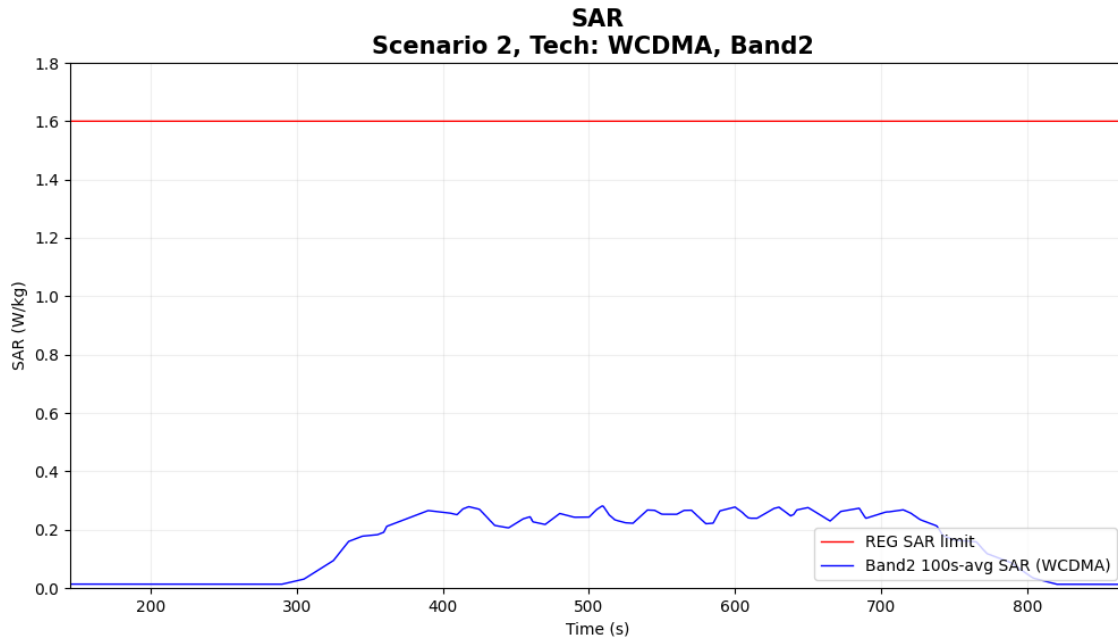
Figure 6-13 Time-averaged SAR for case 13 in table 6-1 (WCDMA B2)
