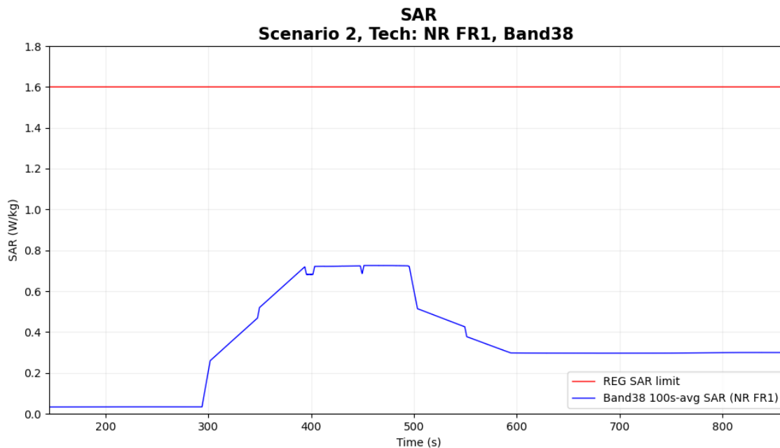
Figure 6-3 Time-averaged SAR for case 9 in table 6-1 (sub6 NR n38)
