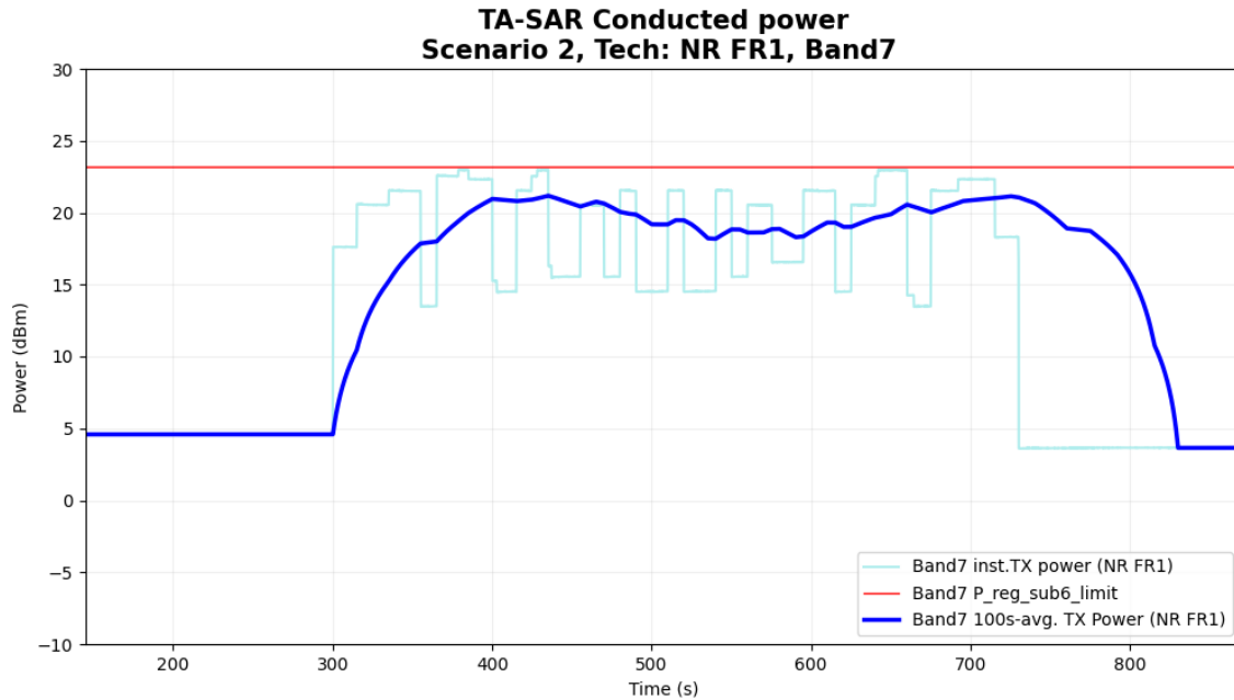
Figure 5-13 Time-averaged conducted TX power over time for case 16 (sub6 NR n7)
