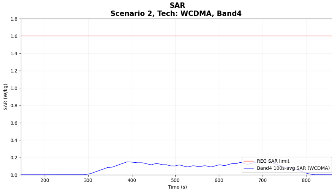
Figure 6-12 Time-averaged SAR for case 12 in table 6-1 (WCDMA B4)
