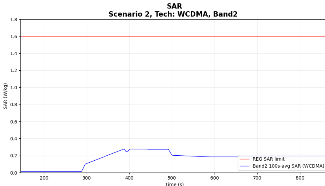
Figure 6-11 Time-averaged SAR for case 5 in table 6-1 (WCDMA B2)
