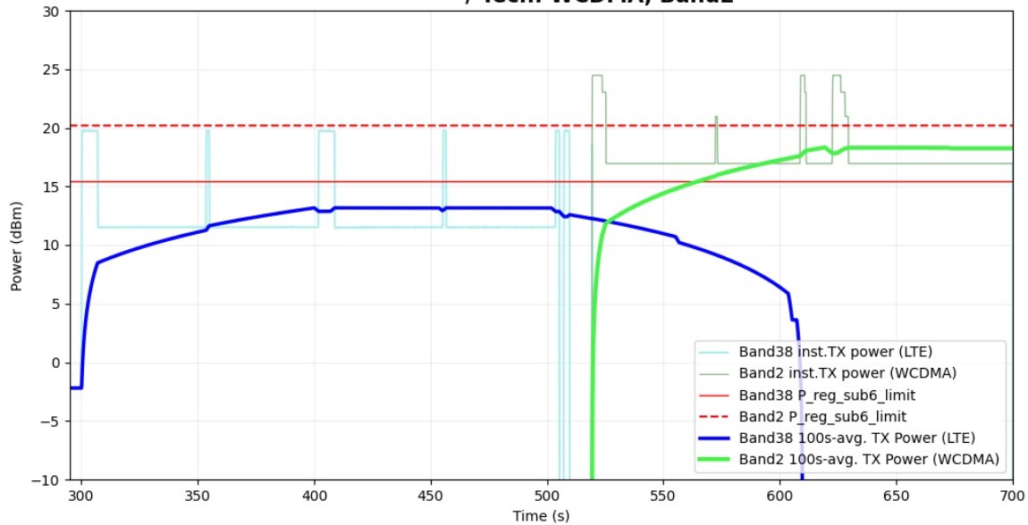
Figure 5-43 Time-averaged conducted TX power over time for case 19 (LTE B38, WCDMA B2)
