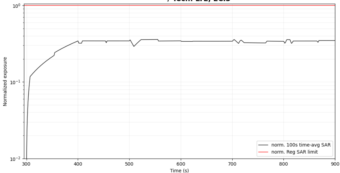
Figure 5-46 Normalized time-averaged SAR for case 20 (LTE ECI2, ECI3)
