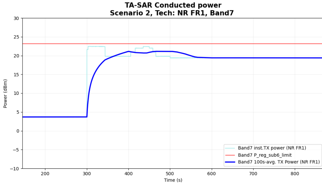
Figure 5-9 Time-averaged conducted TX power over time for case 8 (sub6 NR n7)
