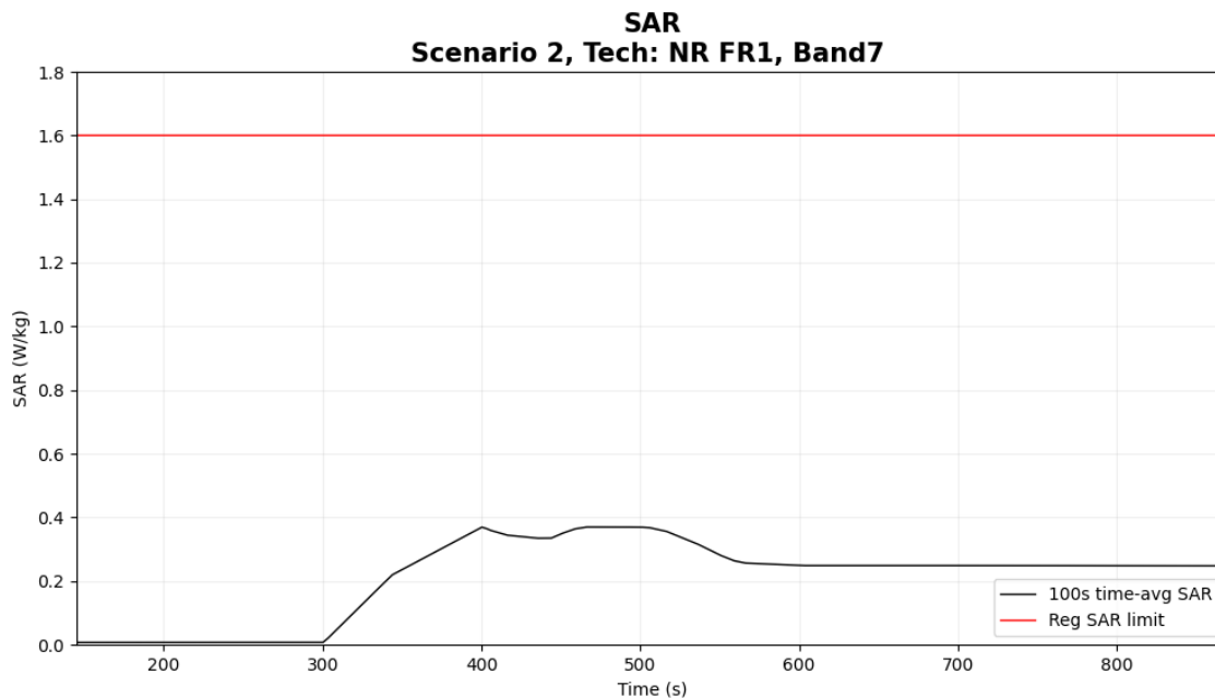
Figure 5-10 Time-averaged SAR for case 8 (sub6 NR n7)
