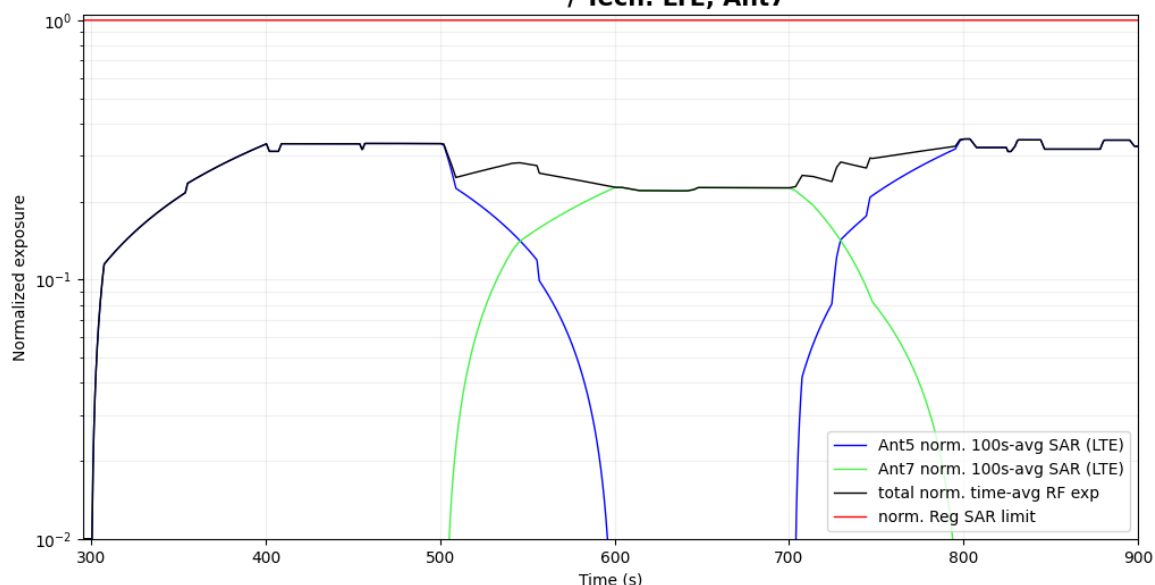
Figure 5-48 Normalized time-averaged SAR for case 21 (LTE Ant5, Ant7)
