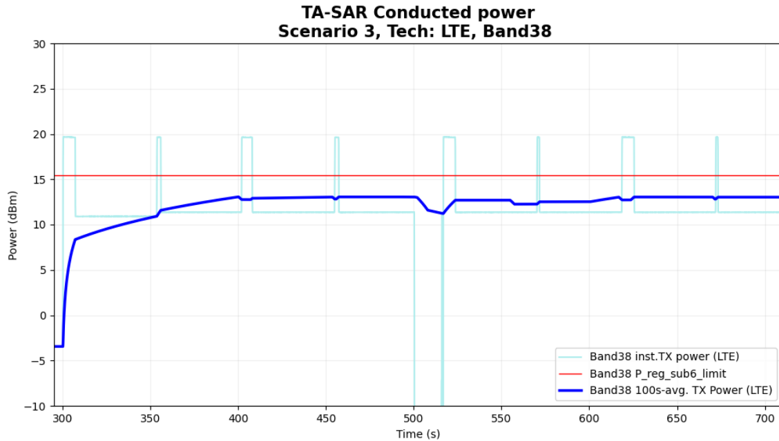
Figure 5-41 Time-averaged conducted TX power over time for case 18 (LTE B38)
