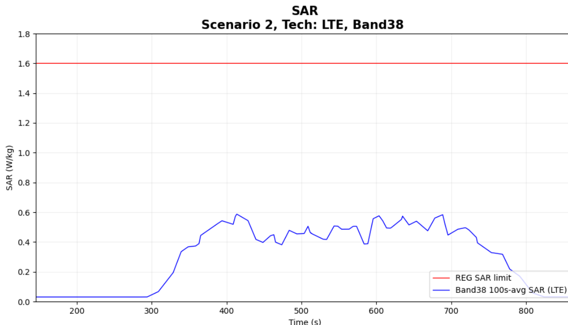
Figure 6-9 Time-averaged SAR for case 15 in table 6-1 (LTE B38)
