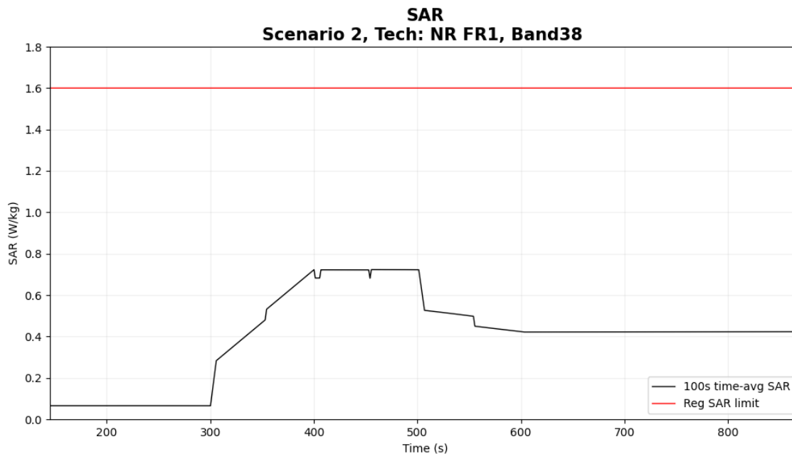
Figure 5-12 Time-averaged SAR for case 9 (sub6 NR n38)
