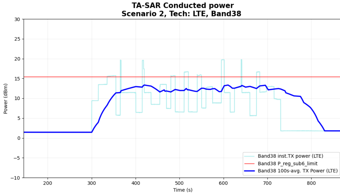
Figure 5-23 Time-averaged conducted TX power over time for case 15 (LTE B38)
