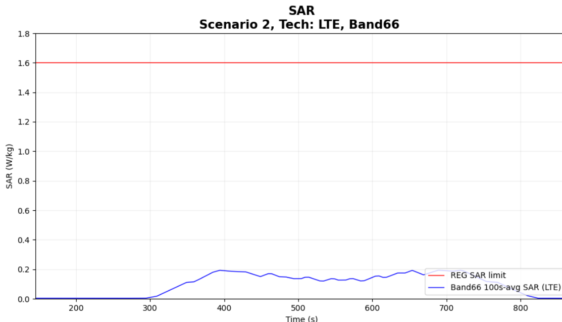
Figure 6-8 Time-averaged SAR for case 14 in table 6-1 (LTE B66)
