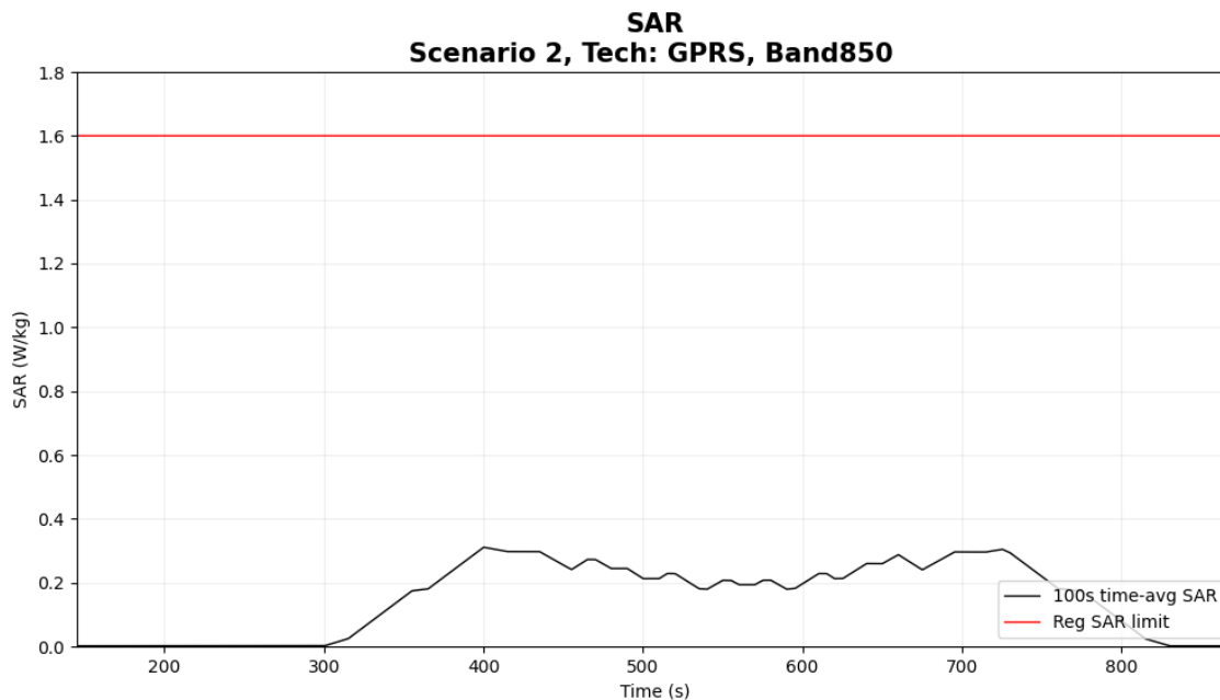
Figure 5-38 Time-averaged SAR for case 10 (2G GPRS 850 2TX)
