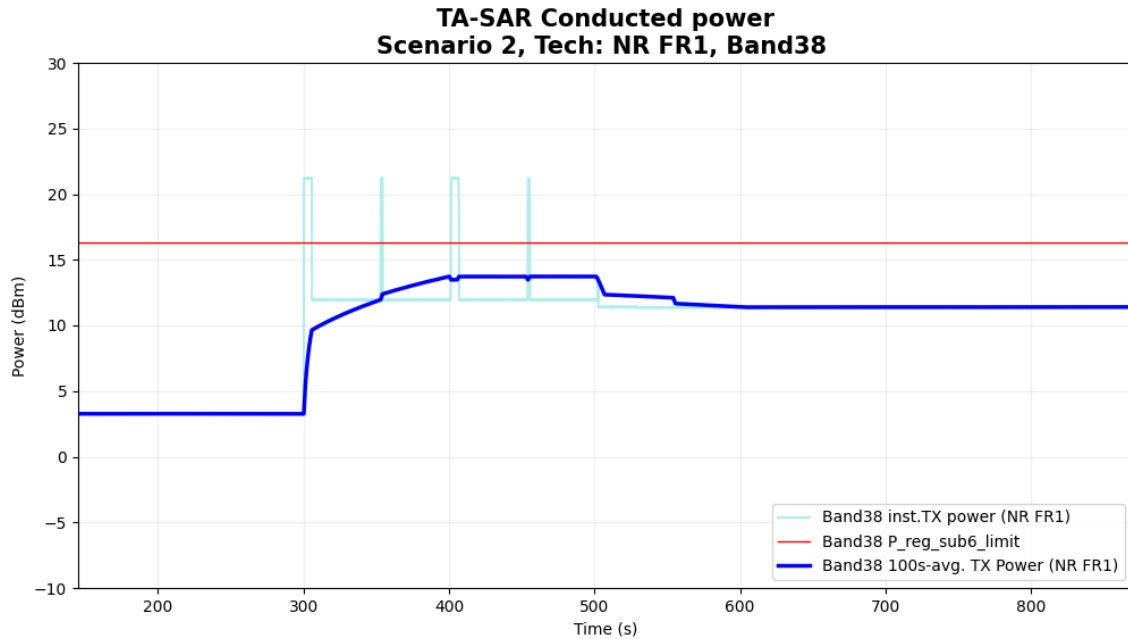
Figure 5-11 Time-averaged conducted TX power over time for case 9 (sub6 NR n38)
