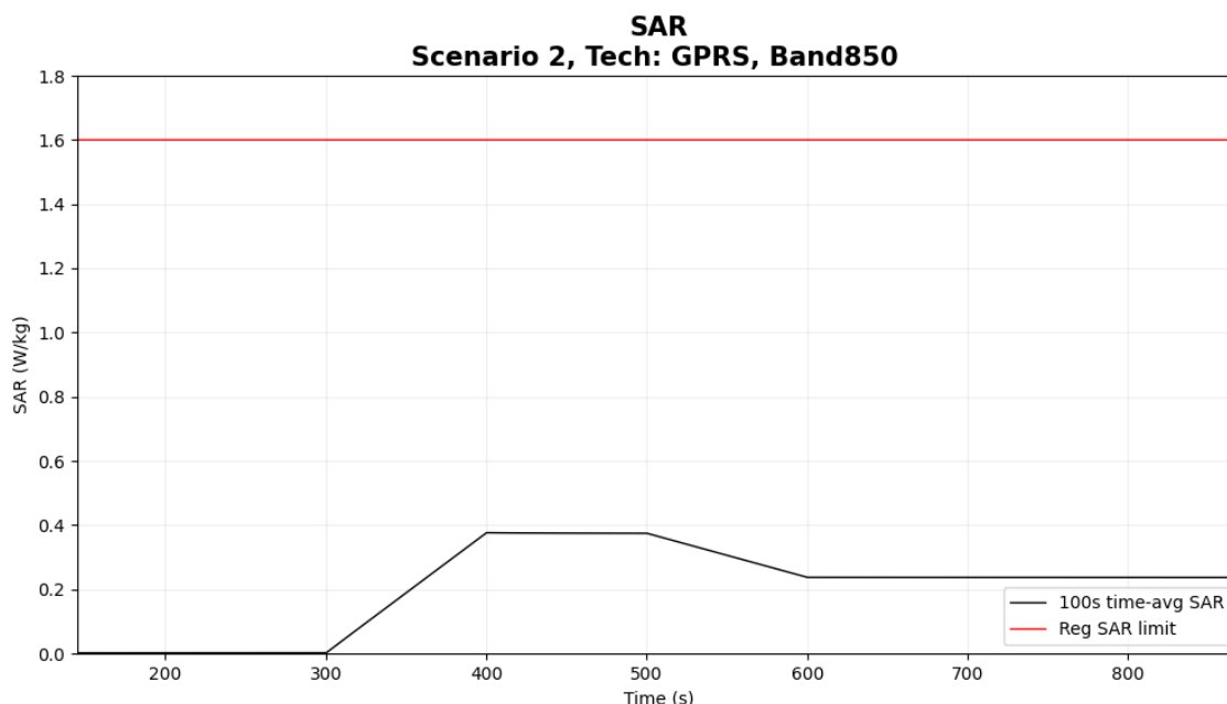
Figure 5-34 Time-averaged SAR for case 2 (2G GPRS 850 2TX)
