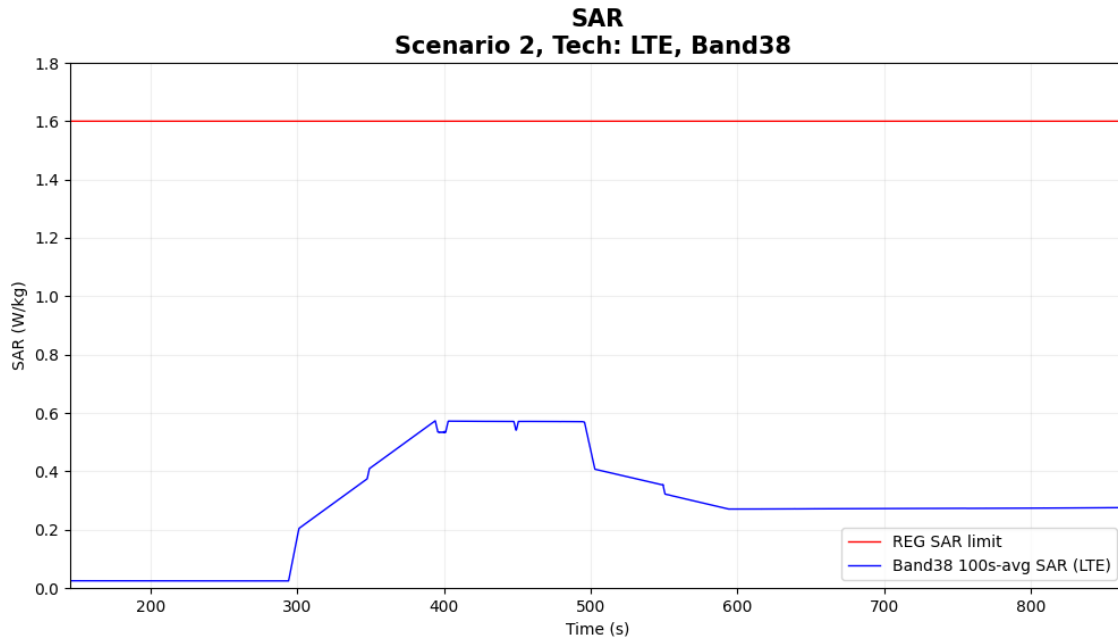
Figure 6-7 Time-averaged SAR for case 7 in table 6-1 (LTE B38)
