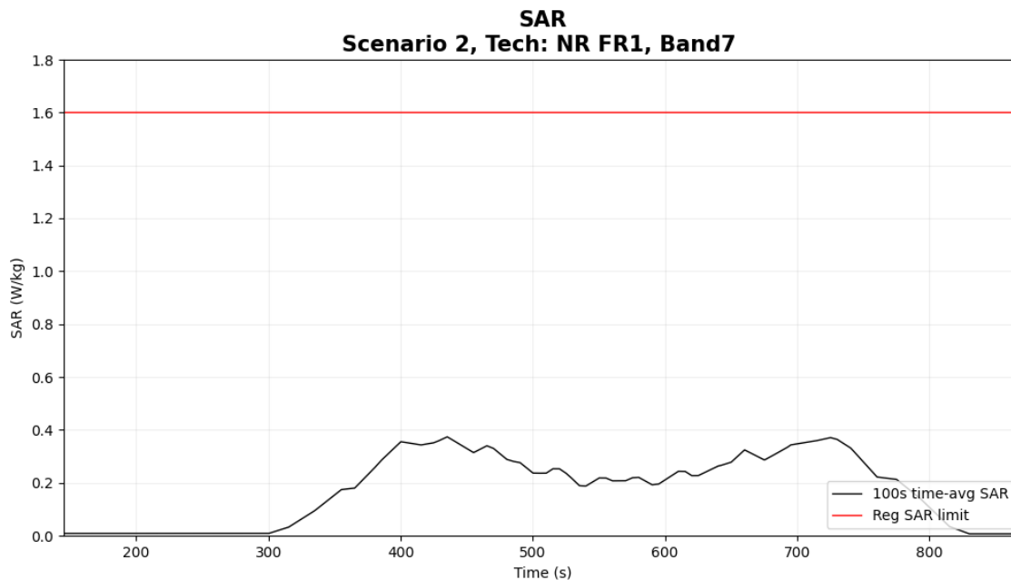
Figure 5-14 Time-averaged SAR for case 16 (sub6 NR n7)
