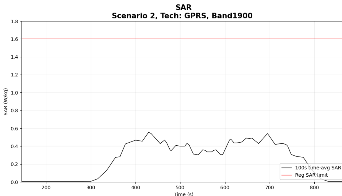
Figure 5-40 Time-averaged SAR for case 11 (2G GPRS 1900 2Tx)
