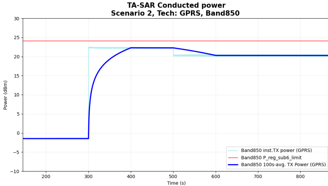
Figure 5-33 Time-averaged conducted TX power over time for case 2 (2G GPRS 850 2TX)
