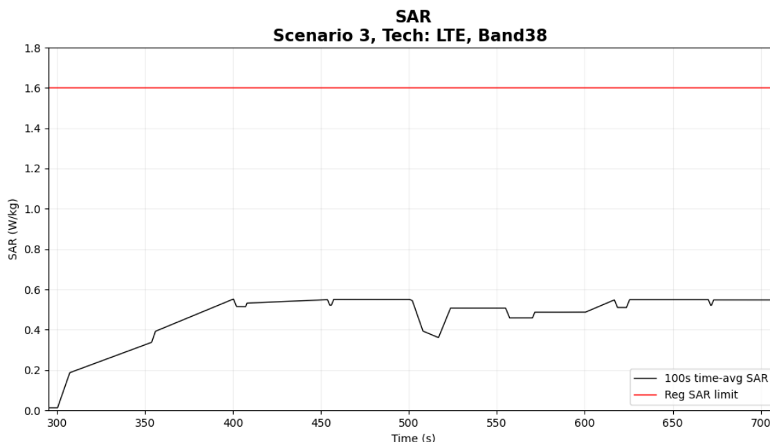
Figure 5-42 Time-averaged SAR for case 18 (LTE B38)
