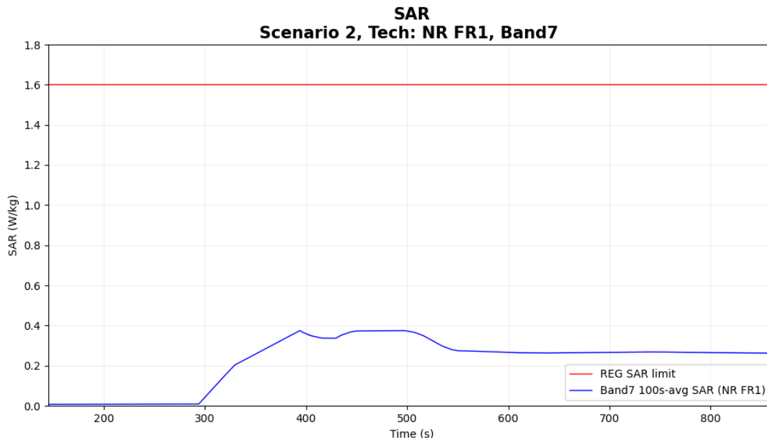
Figure 6-2 Time-averaged SAR for case 8 in table 6-1 (sub6 NR n7)
