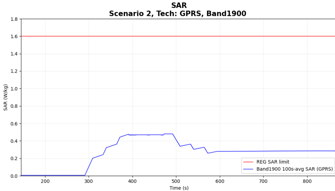
Figure 6-15 Time-averaged SAR for case 3 in table 6-1 (2G GPRS 1900)
