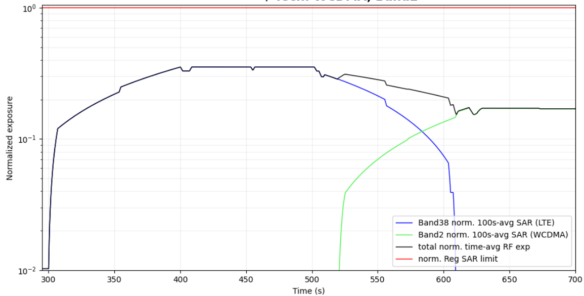
Figure 5-44 Normalized time-averaged SAR for case 19 (LTE B38, WCDMA B2)
