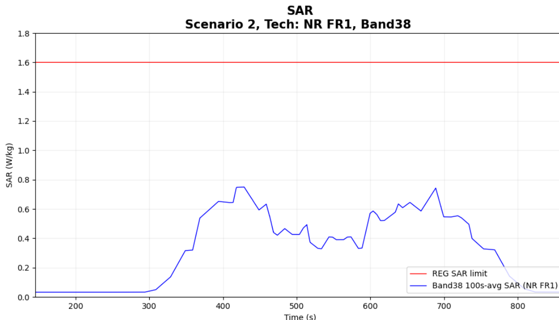
Figure 6-5 Time-averaged SAR for case 17 in table 6-1 (sub6 NR n38)
