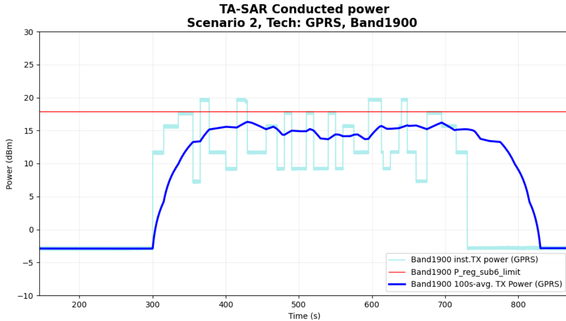
Figure 5-39 Time-averaged conducted TX power over time for case 11 (2G GPRS 1900 2Tx)
