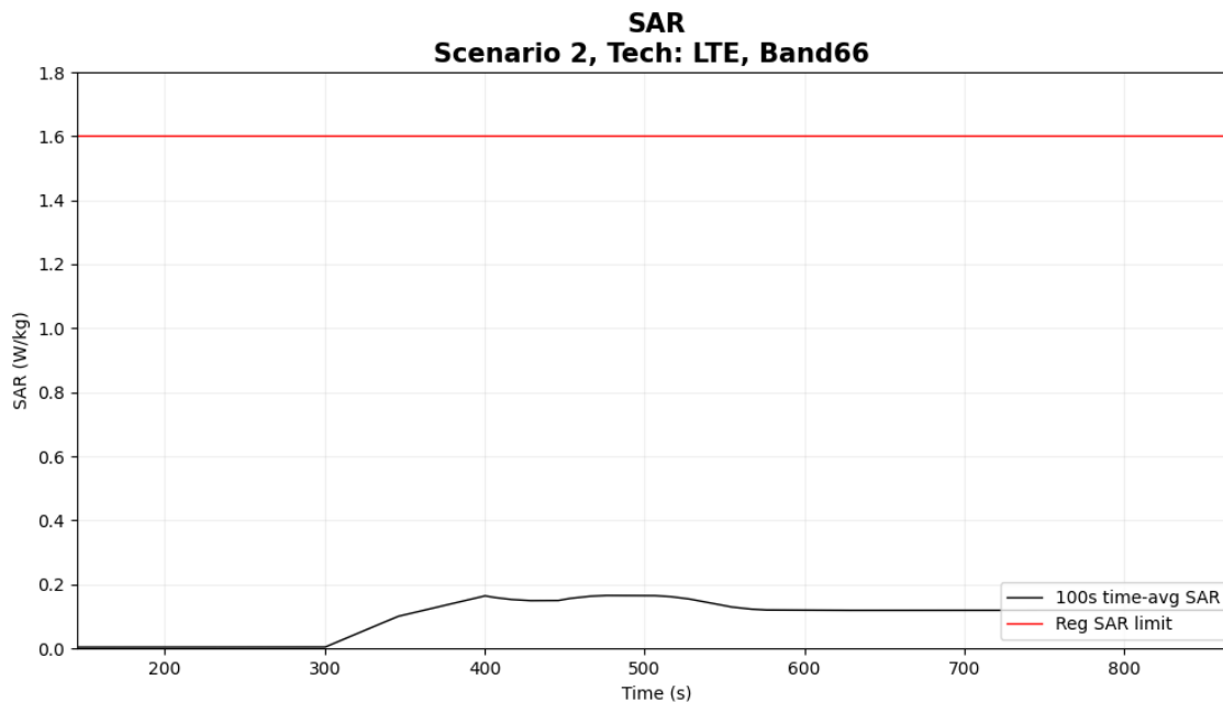
Figure 5-18 Time-averaged SAR for case 6 (LTE B66)
