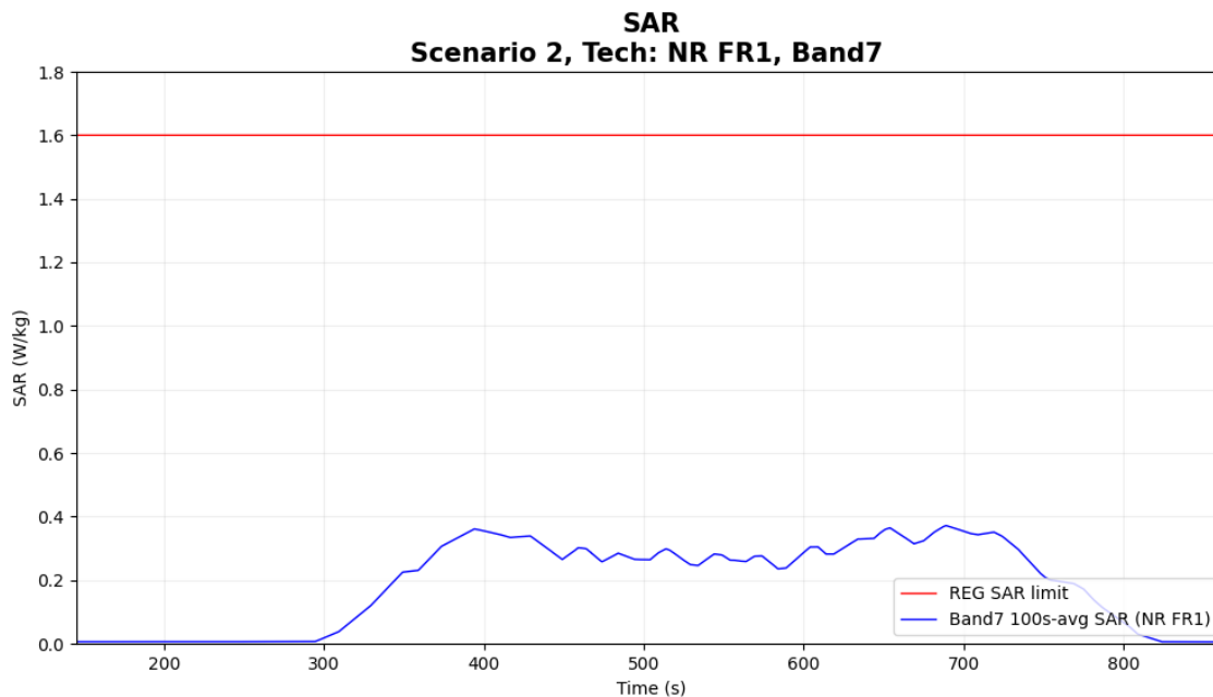
Figure 6-4 Time-averaged SAR for case 16 in table 6-1 (sub6 NR n7)
