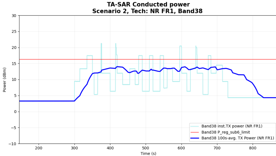
Figure 5-15 Time-averaged conducted TX power over time for case 17 (sub6 NR n38)
