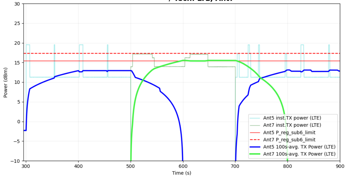
Figure 5-47 Time-averaged conducted TX power over time for case 21 (LTE Ant5, Ant7)
