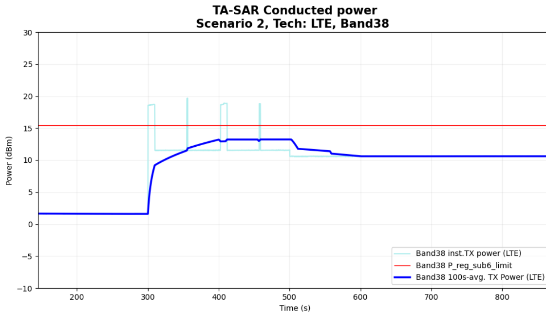
Figure 5-19 Time-averaged conducted TX power over time for case 7 (LTE B38)
