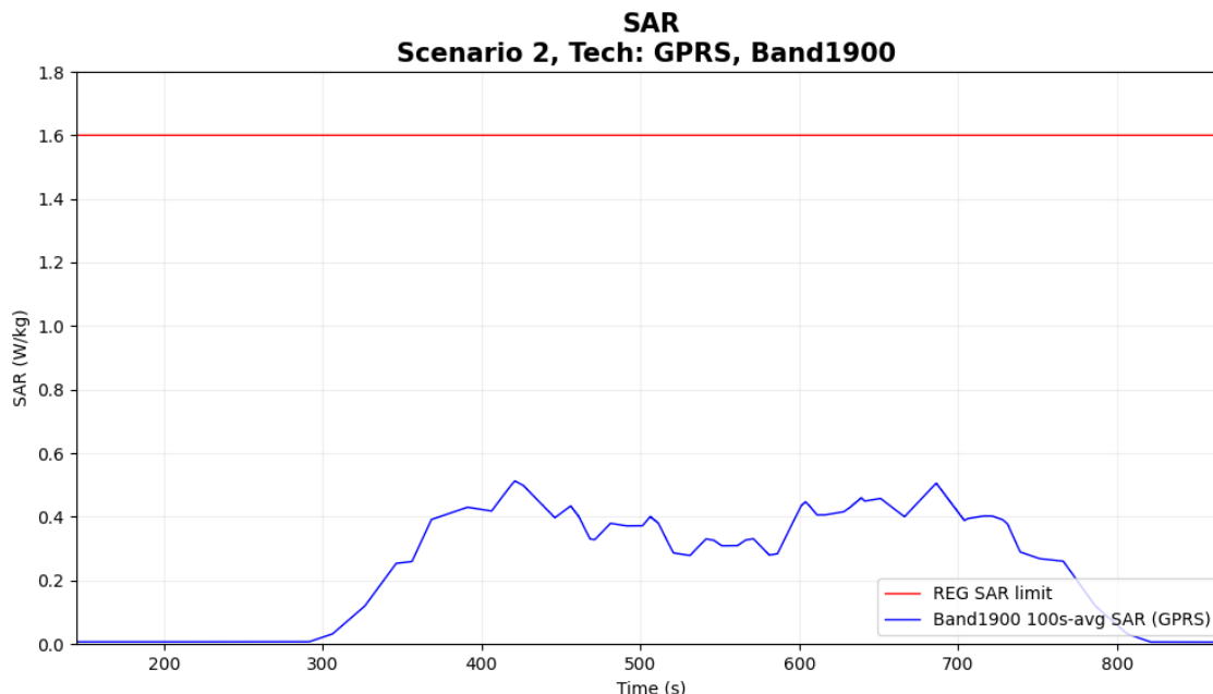
Figure 6-17 Time-averaged SAR for case 11 in table 6-1 (2G GPRS 1900)
