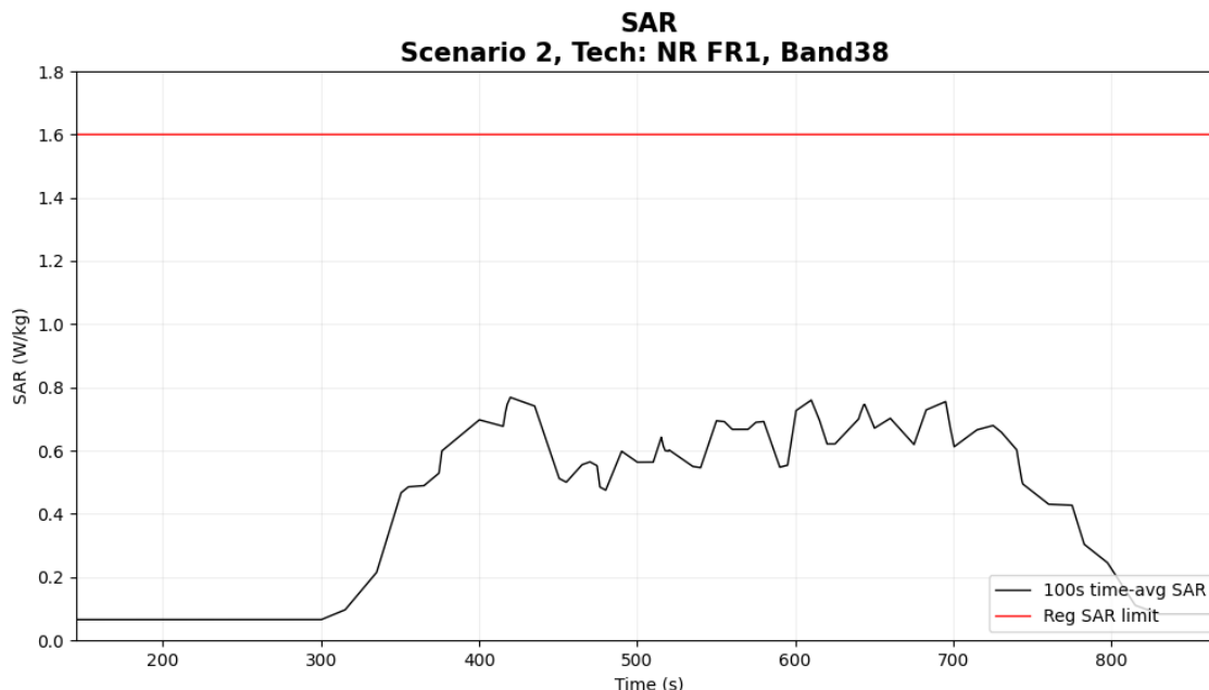
Figure 5-16 Time-averaged SAR for case 17 (sub6 NR n38)
