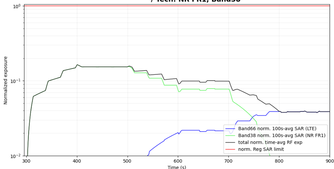
Figure 5-50 Normalized time-averaged SAR for case 22 (LTE B66, sub6 NR n38)
