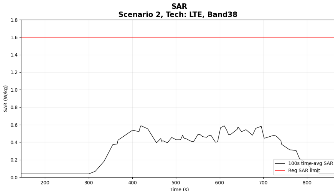
Figure 5-24 Time-averaged SAR for case 15 (LTE B38)
