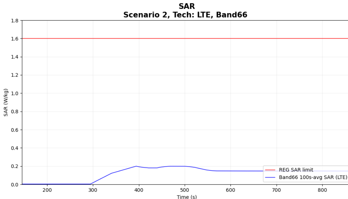
Figure 6-6 Time-averaged SAR for case 6 in table 6-1 (LTE B66)
