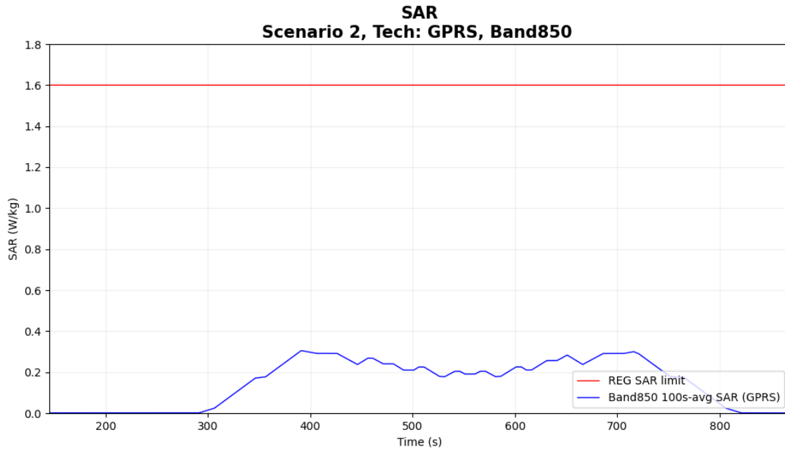
Figure 6-16 Time-averaged SAR for case 10 in table 6-1 (2G GPRS 850)
