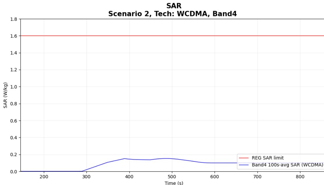
Figure 6-10 Time-averaged SAR for case 4 in table 6-1 (WCDMA B4)
