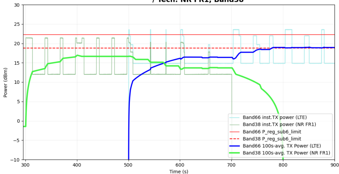
Figure 5-49 Time-averaged conducted TX power over time for case 22 (LTE B66, sub6 NR n38)
