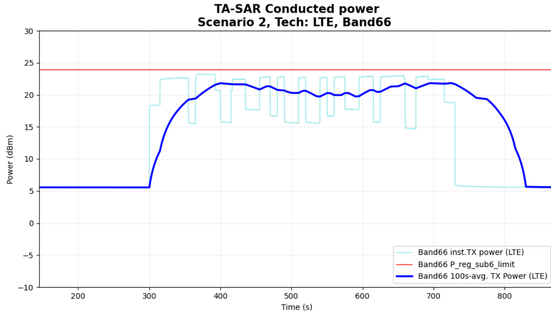
Figure 5-21 Time-averaged conducted TX power over time for case 14 (LTE B66)
