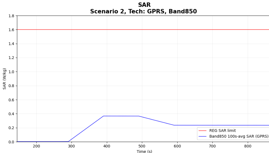
Figure 6-14 Time-averaged SAR for case 2 in table 6-1 (2G GPRS 850)
