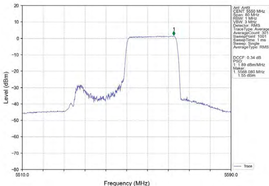
802.11ax(HEW40)_MCH_5550MHz_RU242_Right_Ant9_NTNV
