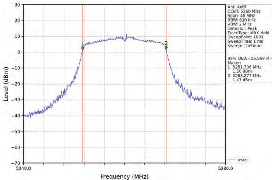
802.11a_LCH_5260MHz_Ant9_NTNV
