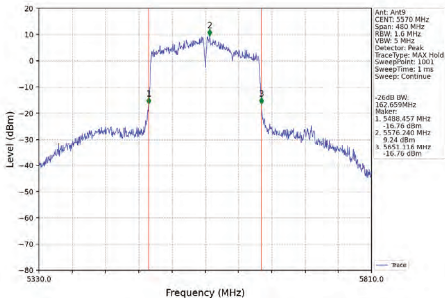
802.11ac(VHT160)_MCH_5570MHz_Ant9_NTNV
