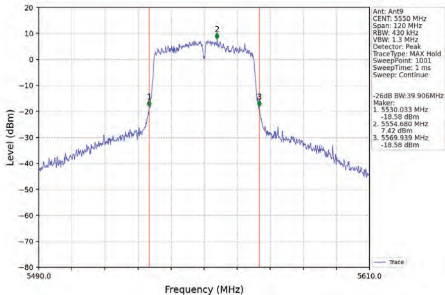
802.11ac(VHT40)_MCH_5550MHz_Ant9_NTNV
