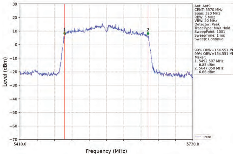
802.11ac(VHT160)_MCH_5570MHz_Ant9_NTNV
