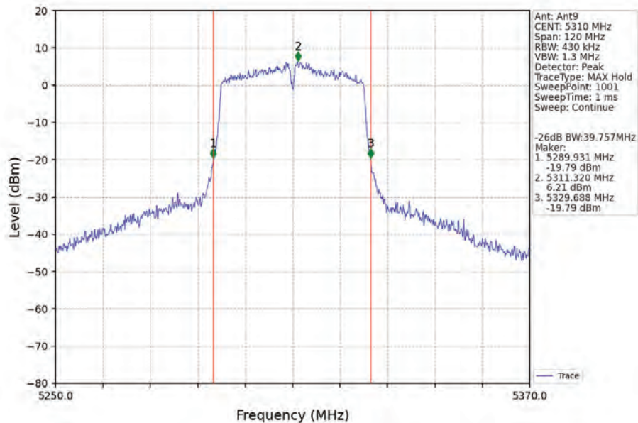
802.11ac(VHT40)_HCH_5310MHz_Ant9_NTNV
