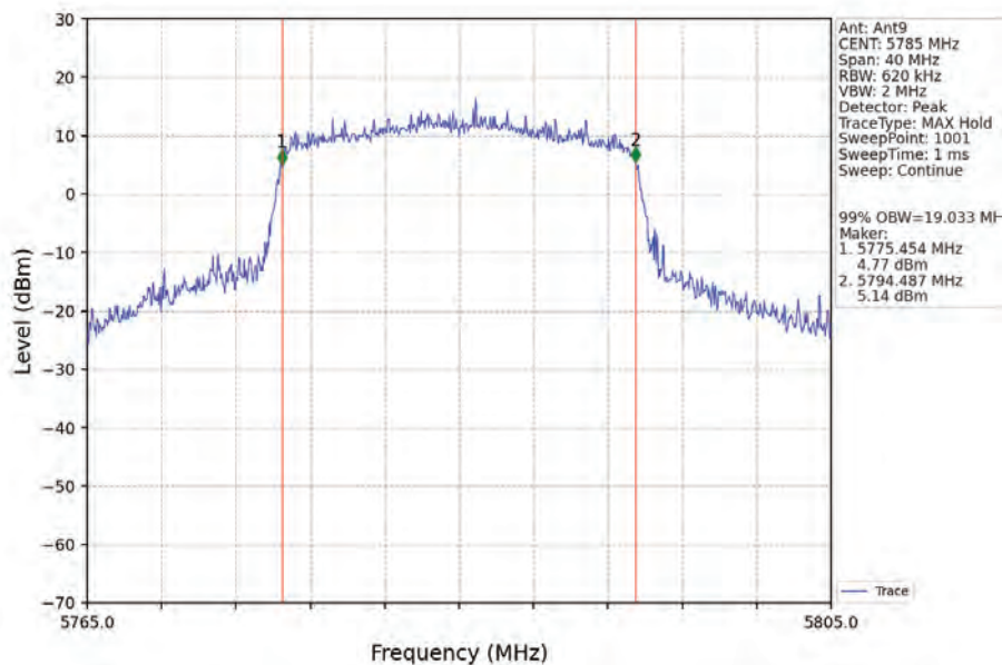
802.11ax(HEW20)_MCH_5785MHz_RU242_Left_Ant9_NTNV
