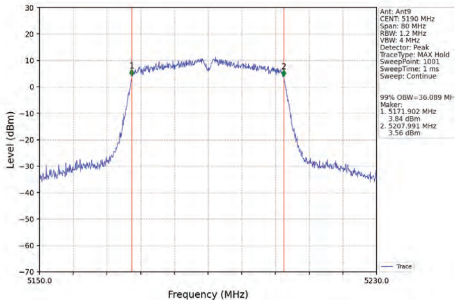
802.11ac(VHT40)_LCH_5190MHz_Ant9_NTNV
