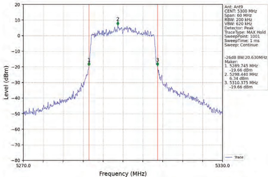
802.11ax(HEW20)_MCH_5300MHz_RU242_Left_Ant9_NTNV
