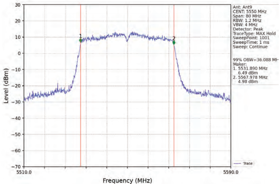
802.11n(HT40)_MCH_5550MHz_Ant9_NTNV
