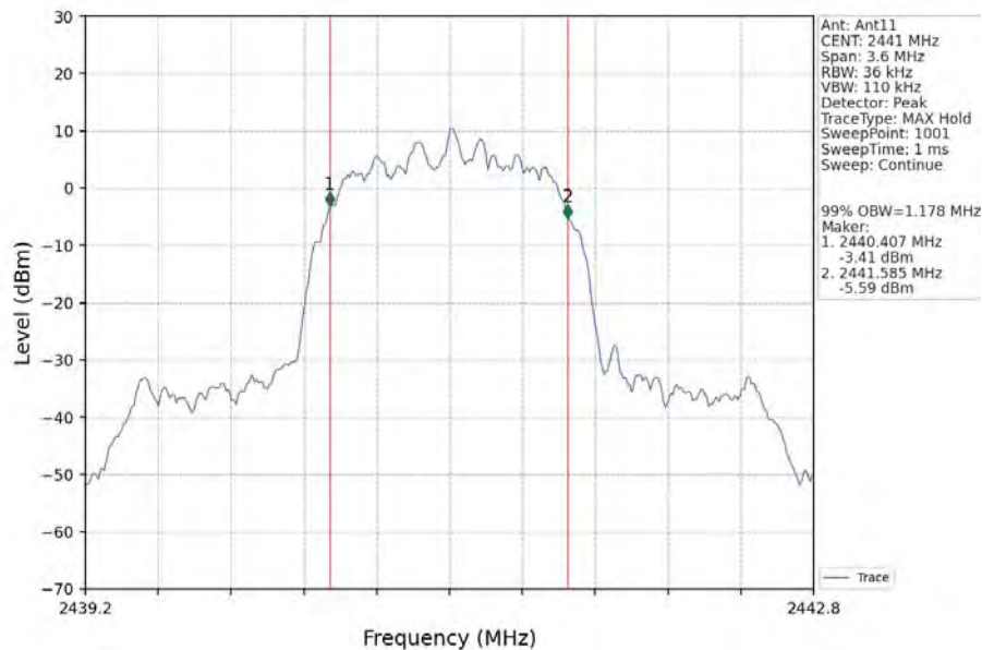
Pi/4DQPSK_2DH5_MCH_2441MHz_Ant11_NTNV
