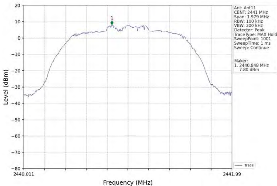
Pi/4DQPSK_2DH5_MCH_2441MHz_Ant11_NTNV
