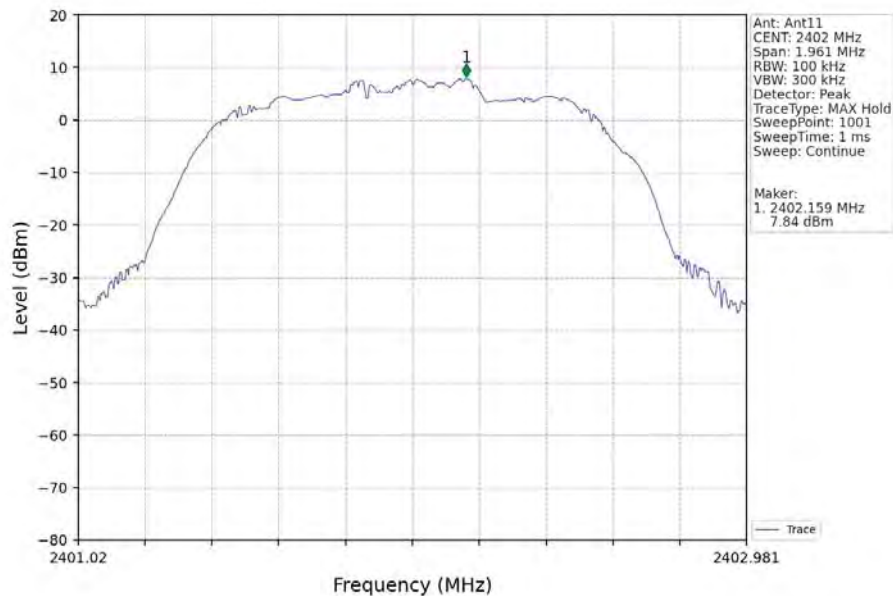
8DPSK_3DH5_LCH_2402MHz_Ant11_NTNV
