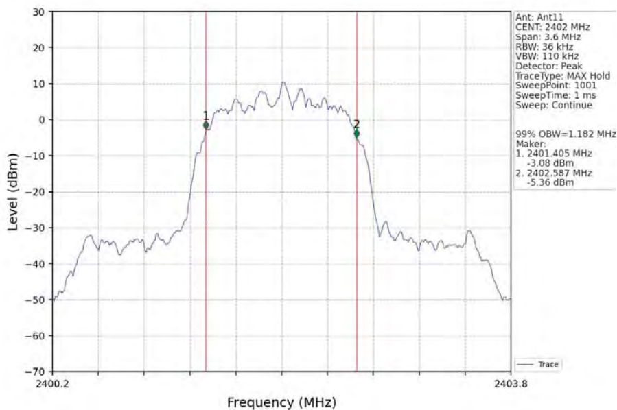
Pi/4DQPSK_2DH5_LCH_2402MHz_Ant11_NTNV
