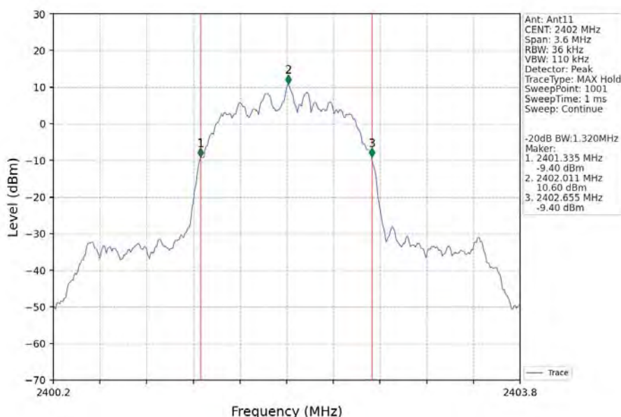
Pi/4DQPSK_2DH5_LCH_2402MHz_Ant11_NTNV
