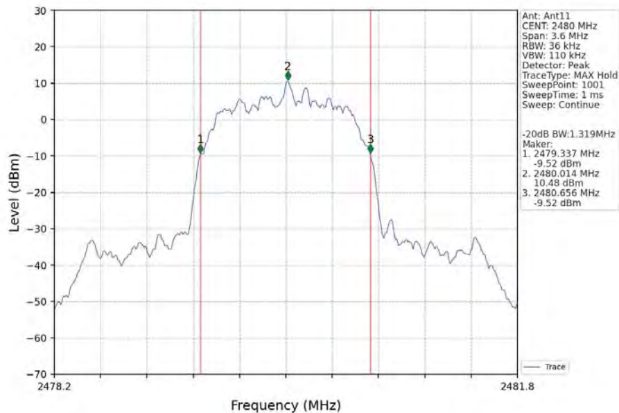
Pi/4DQPSK_2DH5_HCH_2480MHz_Ant11_NTNV
