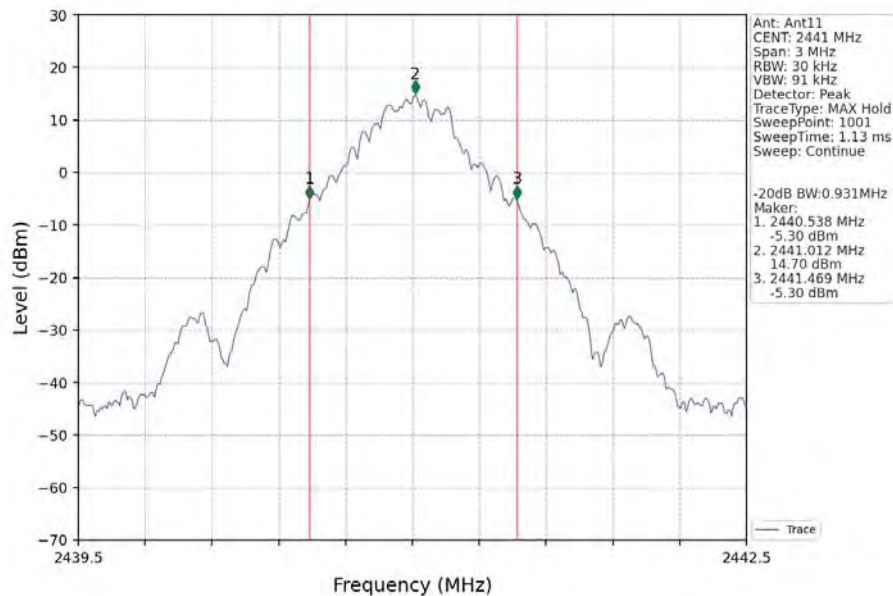
GFSK_DH5_MCH_2441MHz_Ant11_NTNV
