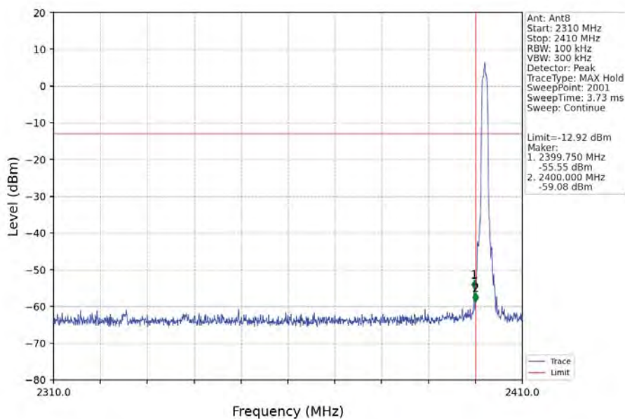
Pi/4DQPSK_2DH5_LCH_2402MHz_Ant8_NTNV
