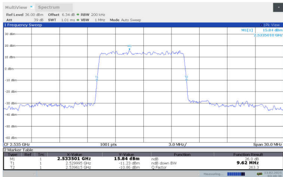
n7,10MHz Bandwidth,DFT-s-16QAM (-26dBc OBW)
