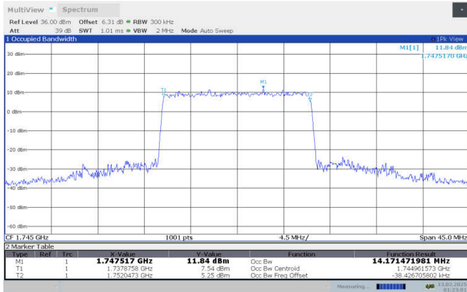
n66,15MHz Bandwidth,CP-256QAM (99% OBW)
