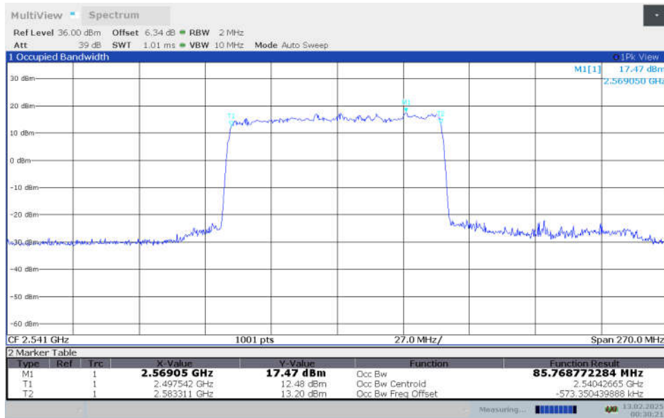
n41,90MHz Bandwidth,CP-QPSK (99% OBW)
