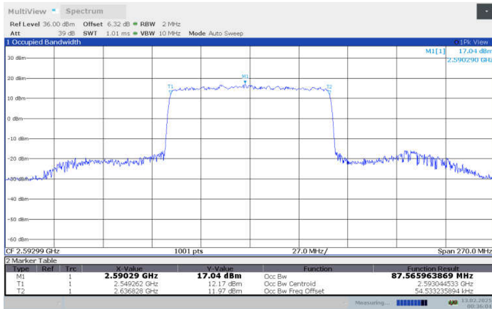
n41,90MHz Bandwidth,CP-256QAM (99% OBW)
