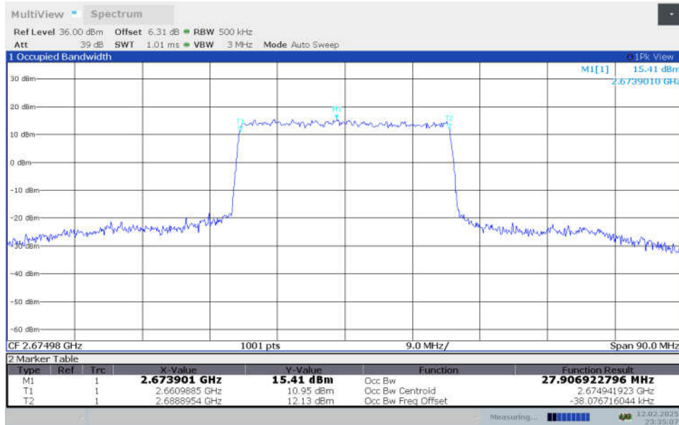
n41,30MHz Bandwidth,CP-QPSK (99% OBW)
