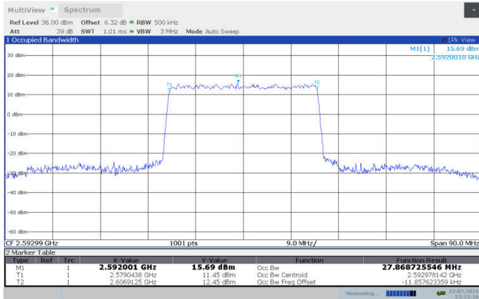
n41,30MHz Bandwidth,CP-16QAM (99% OBW)
