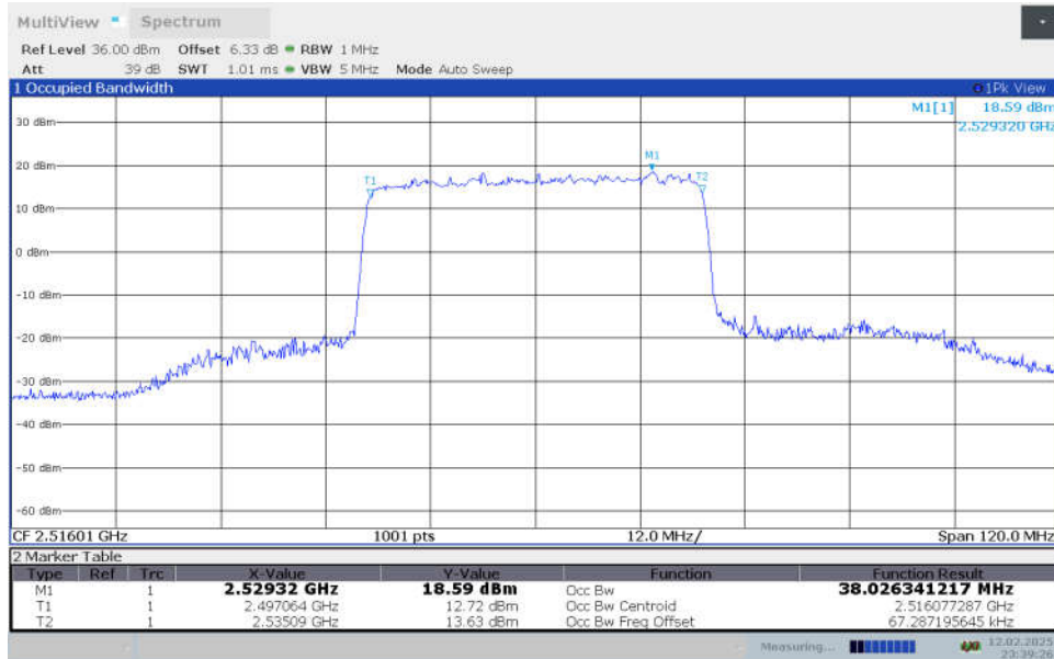
n41,40MHz Bandwidth,CP-QPSK (99% OBW)
