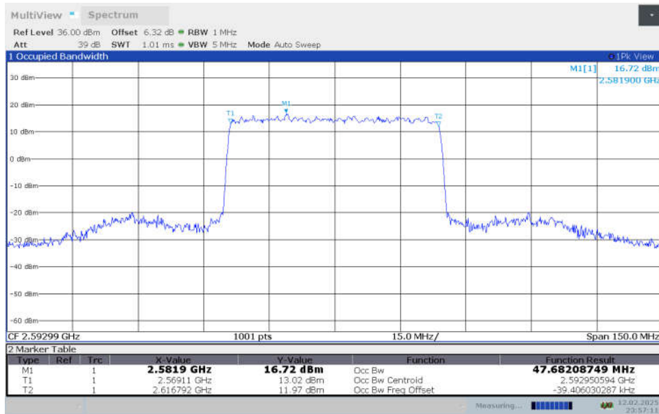
n41,50MHz Bandwidth,CP-256QAM (99% OBW)
