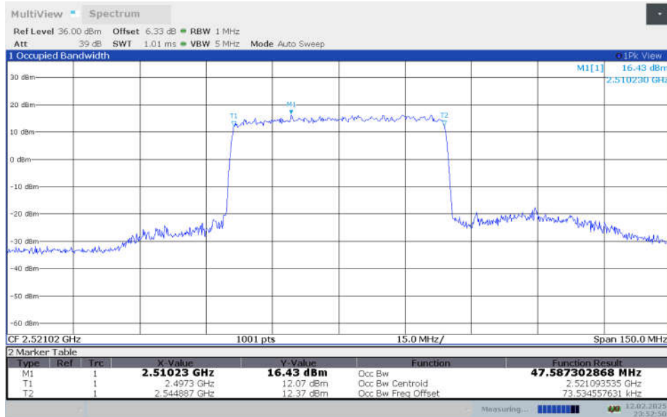
n41,50MHz Bandwidth,CP-64QAM (99% OBW)
