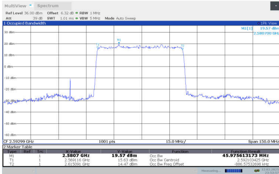
n41,50MHz Bandwidth,DFT-s-pi/2 BPSK (99% OBW)
