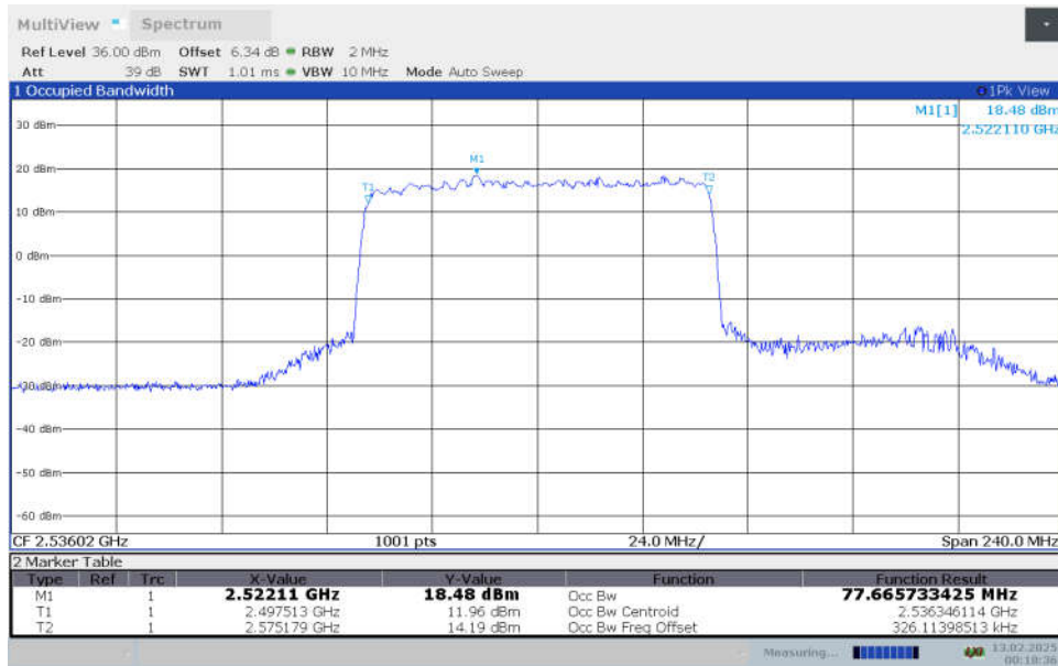
n41,80MHz Bandwidth,CP-64QAM (99% OBW)
