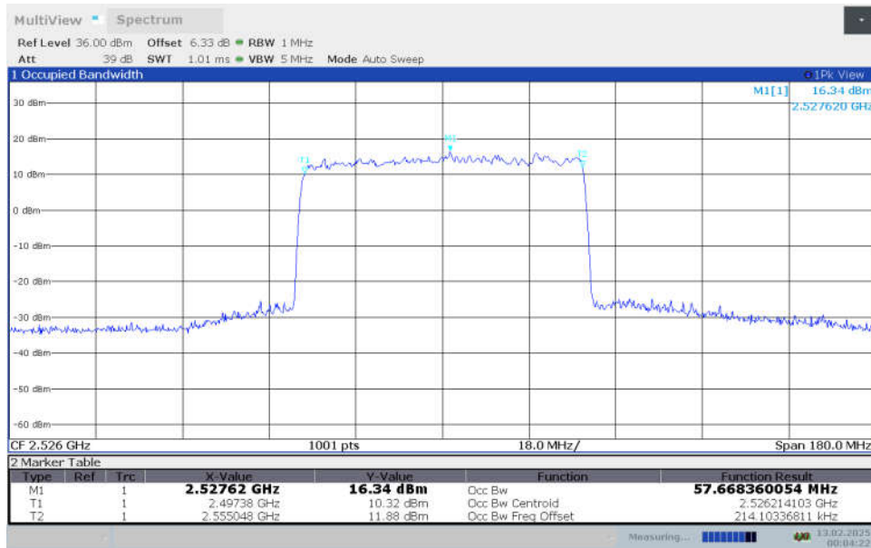
n41,60MHz Bandwidth,CP-QPSK (99% OBW)
