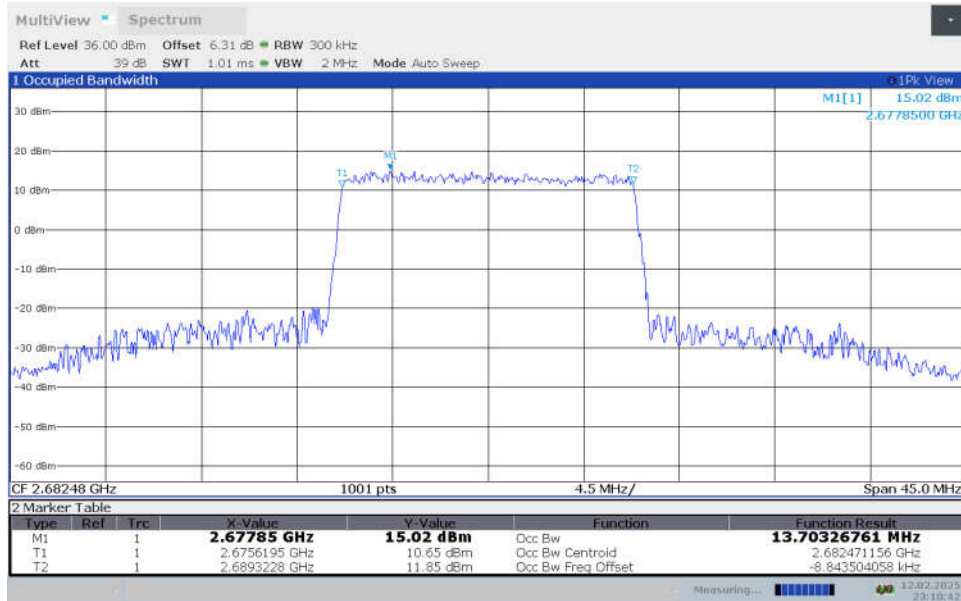
n41,15MHz Bandwidth,CP-64QAM (99% OBW)
