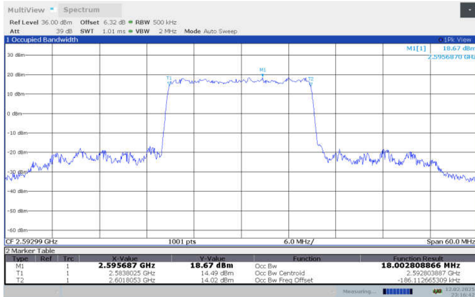
n41,20MHz Bandwidth,DFT-s-16QAM (99% OBW)
