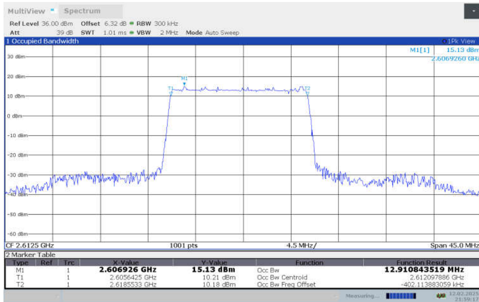
n38,15MHz Bandwidth,DFT-s-64QAM (99% OBW)
