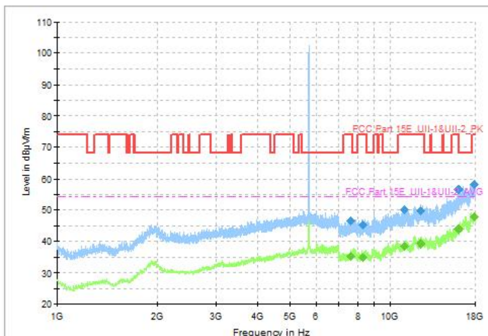
Fig. 54 Transmitter Spurious Emission (802.11ax-HE20, CH140 5700MHz, 1GHz-18GHz), MIMO
