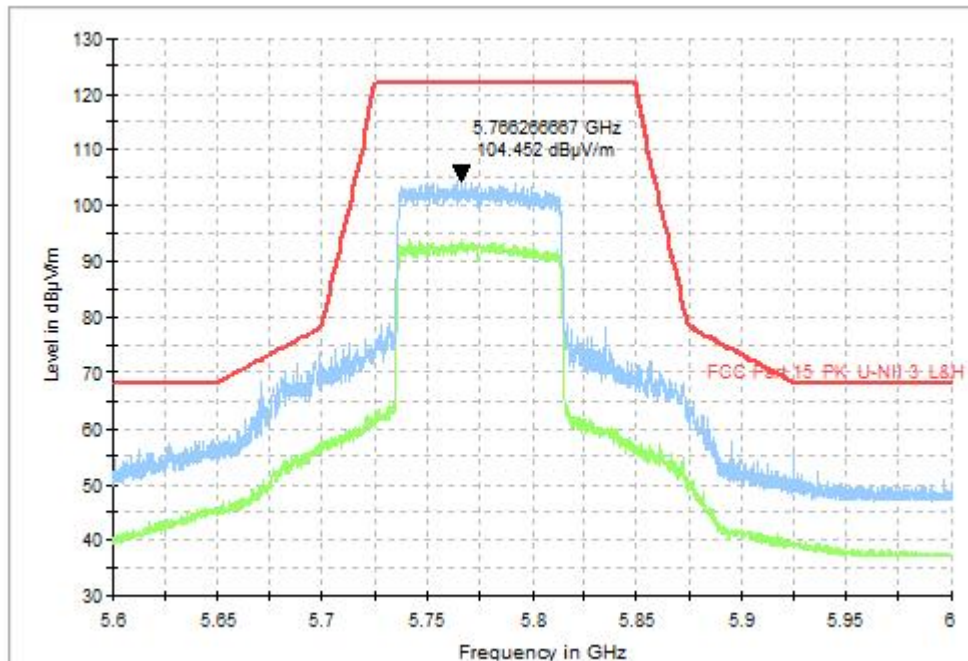
Fig. 43 Band Edges, CH155 5775MHz, MIMO
