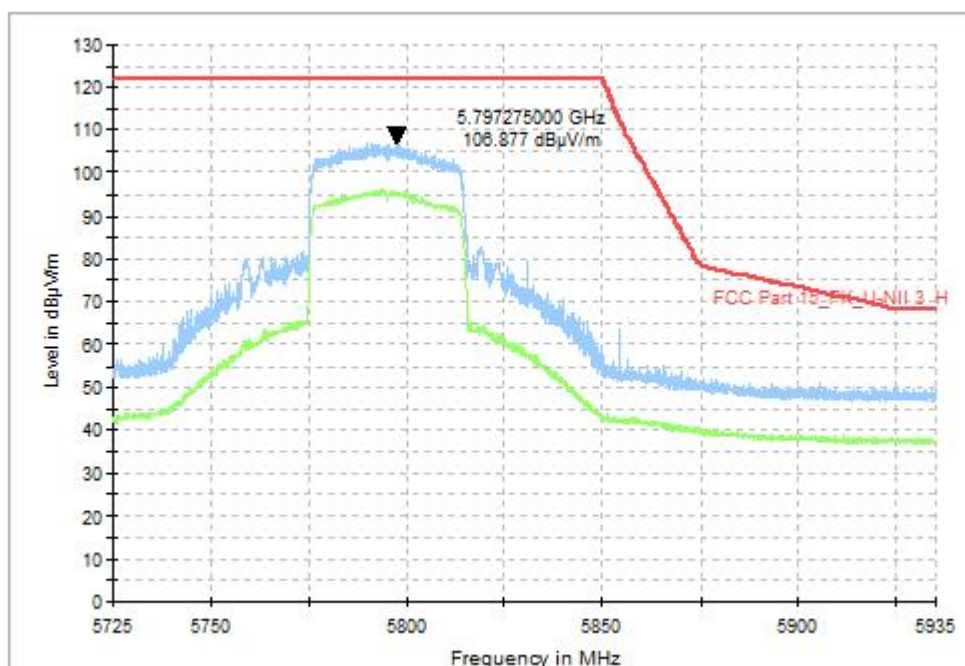
Fig. 38 Band Edges, CH159 5795MHz, MIMO
