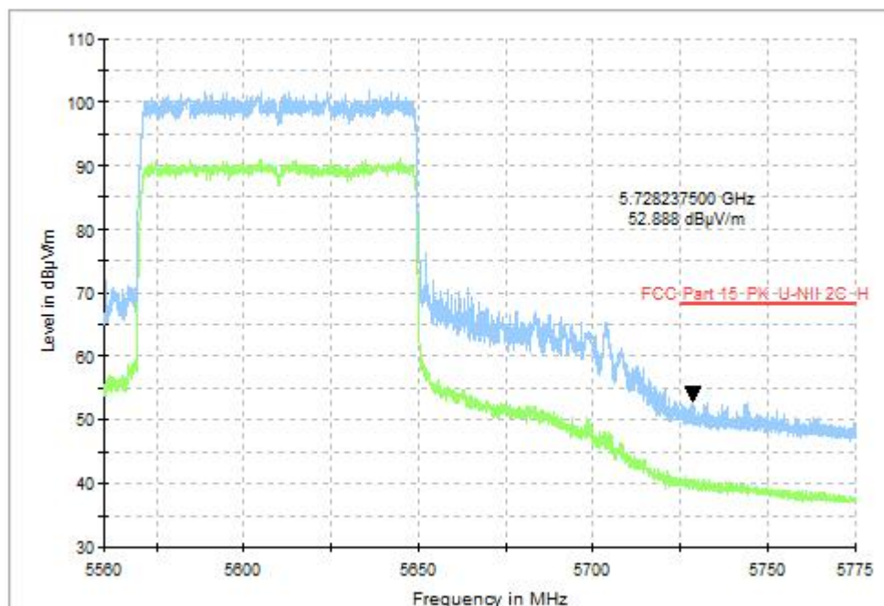
Fig. 42 Band Edges, CH122 5610MHz, MIMO
