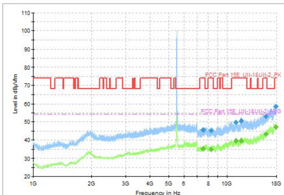
Fig. 62 Transmitter Spurious Emission (802.11ax-HE40, CH102 5510MHz, 1GHz-18GHz), MIMO
