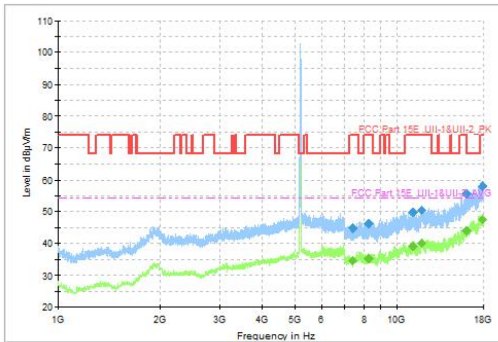
Fig. 47 Transmitter Spurious Emission (802.11ax-HE20, CH40 5200MHz, 1GHz-18GHz), MIMO
