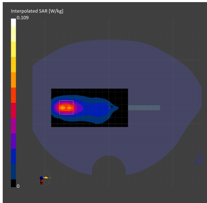
Fig.40 Bluetooth Body
