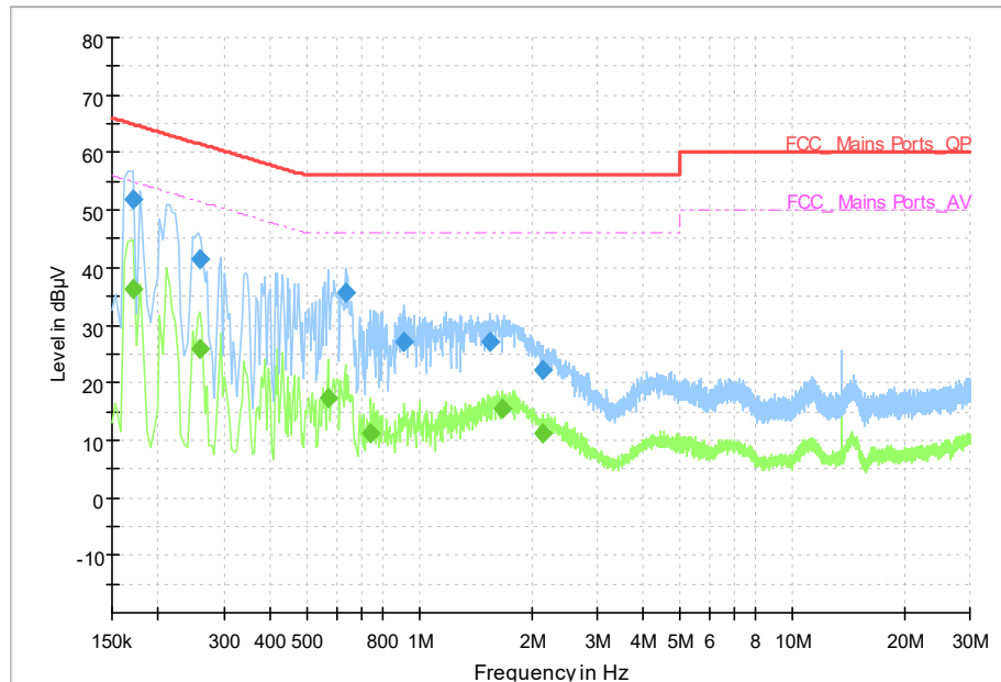
Figure A-6 Conducted Emission (Idle)
