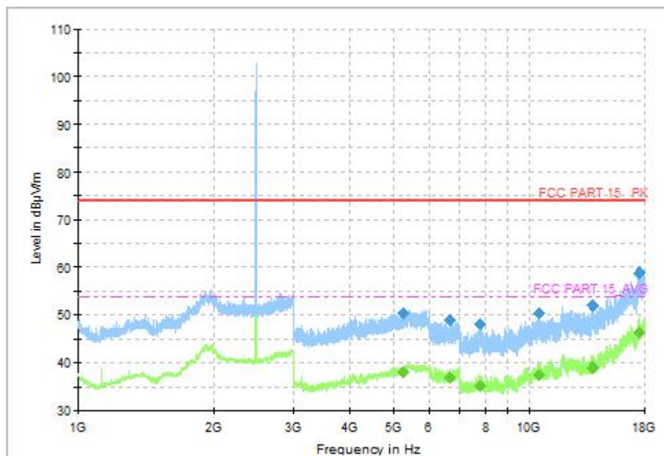
Fig.31 Radiated Spurious Emission (CH38, 1GHz ~18GHz), LE 2M
