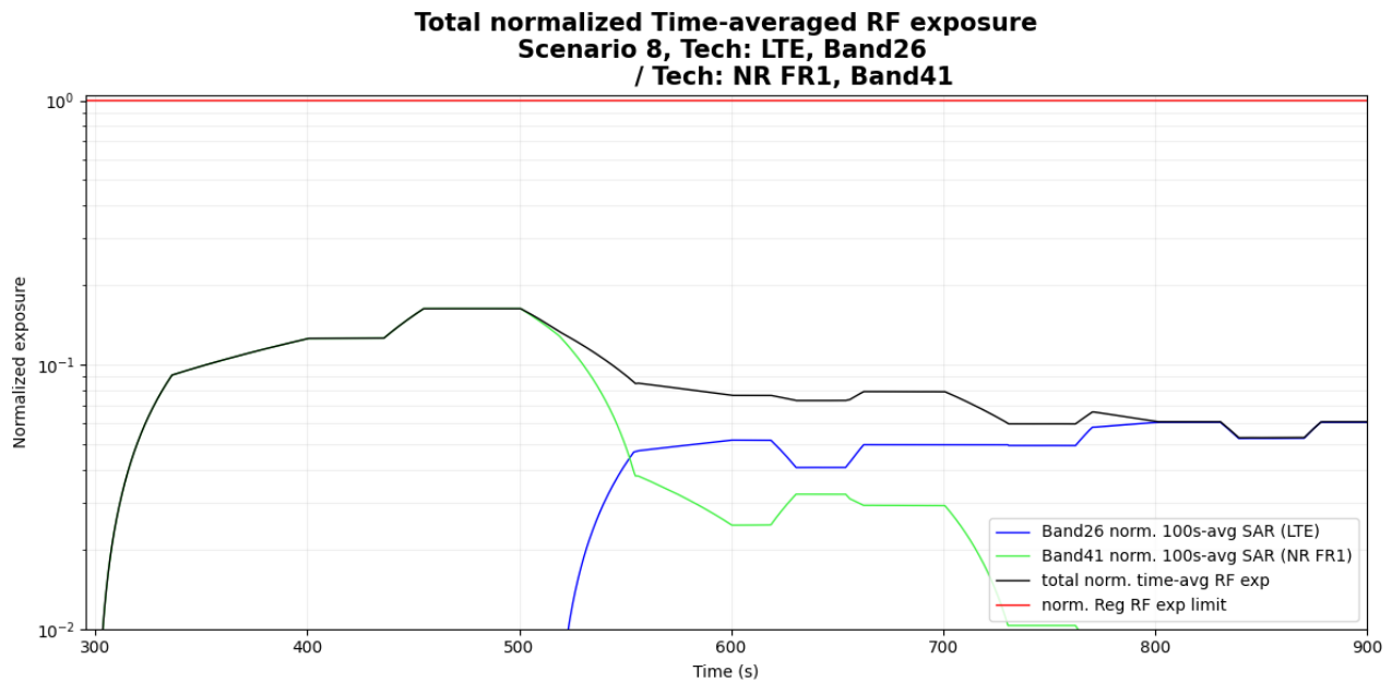
Figure 6- 46 Normalized time-averaged SAR
