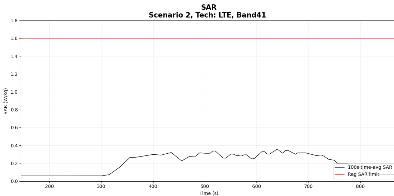
Figure 6- 30 Time-averaged SAR
