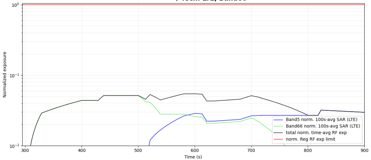
Figure 6- 48 Normalized time-averaged SAR
