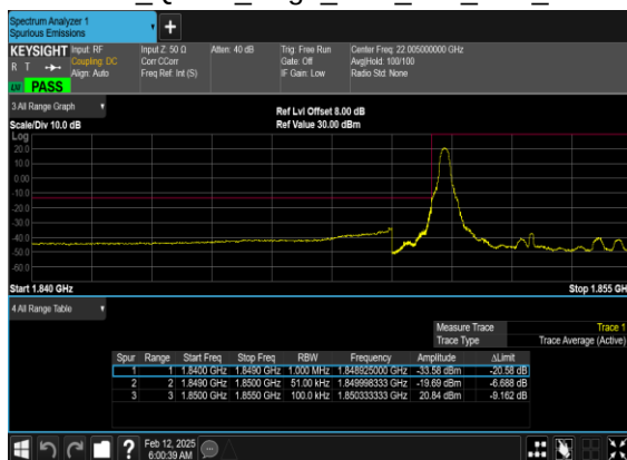
N2(5M)_DFT-s- OFDM_QPSK_Edge_1RB_Left_Low_CH
