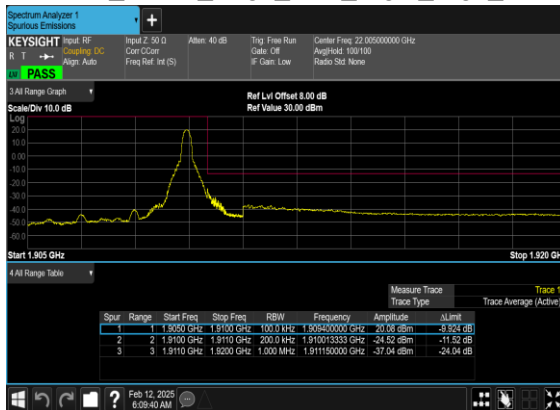
N2(20M)_DFT-s- OFDM_QPSK_Edge_1RB_Right_High_CH
