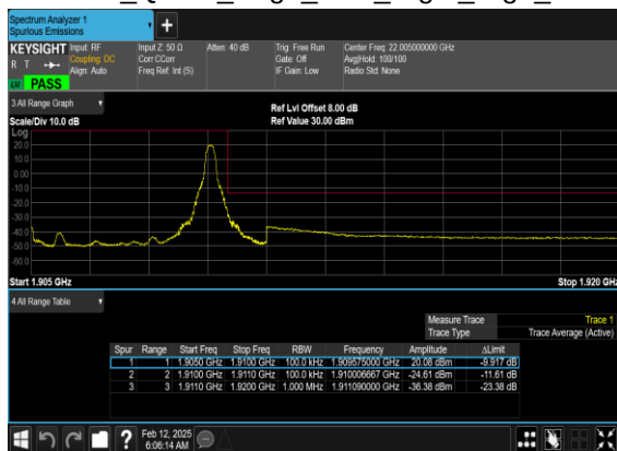
N2(10M)_DFT-s- OFDM_QPSK_Edge_1RB_Right_High_CH
