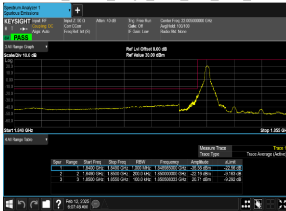
N2(20M)_DFT-s- OFDM_QPSK_Edge_1RB_Left_Low_CH
