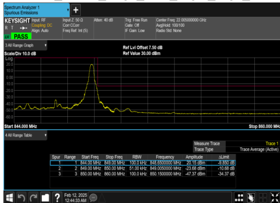
B7_N5(5M)_DFT-s- OFDM_QPSK_Edge_1RB_Right_High_CH
