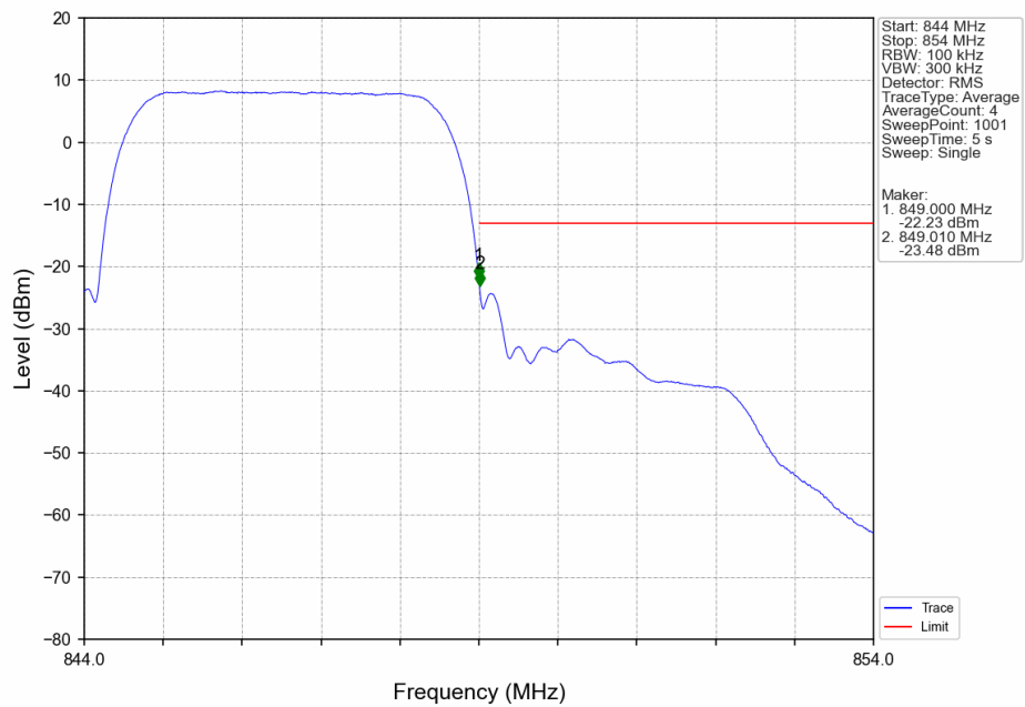
BandV_RMC_HCH_846.6MHz_12.2kbps RMC_NTNV
