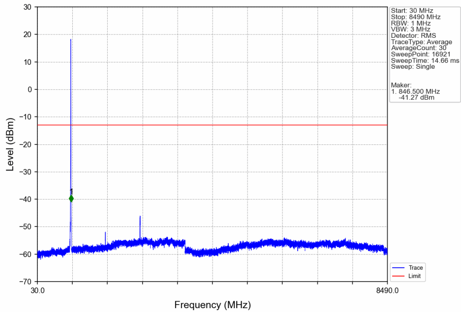
BandV_RMC_HCH_846.6MHz_12.2kbps RMC_NTNV
