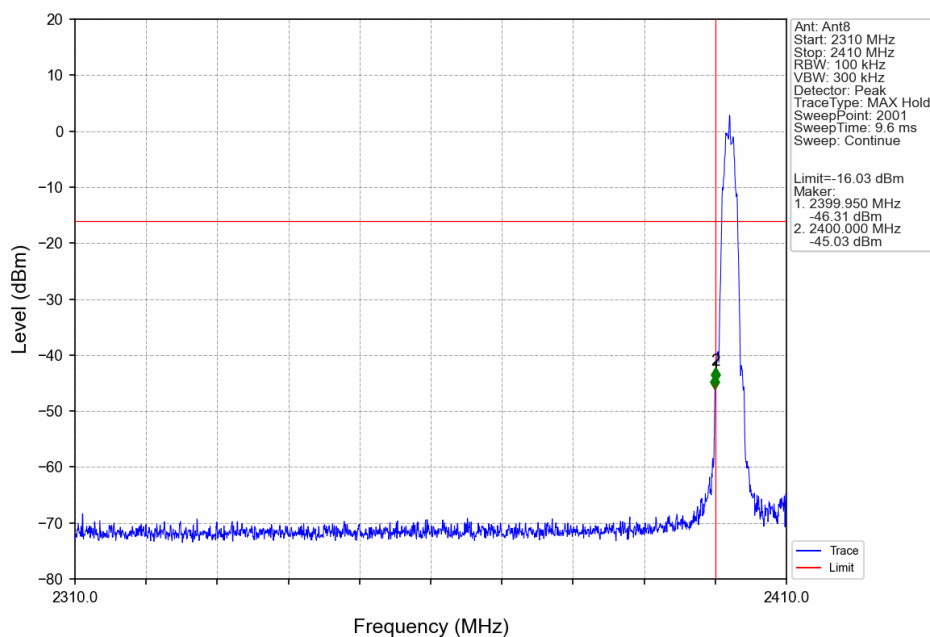
2M_LCH_2402MHz_Ant8_NTNV
