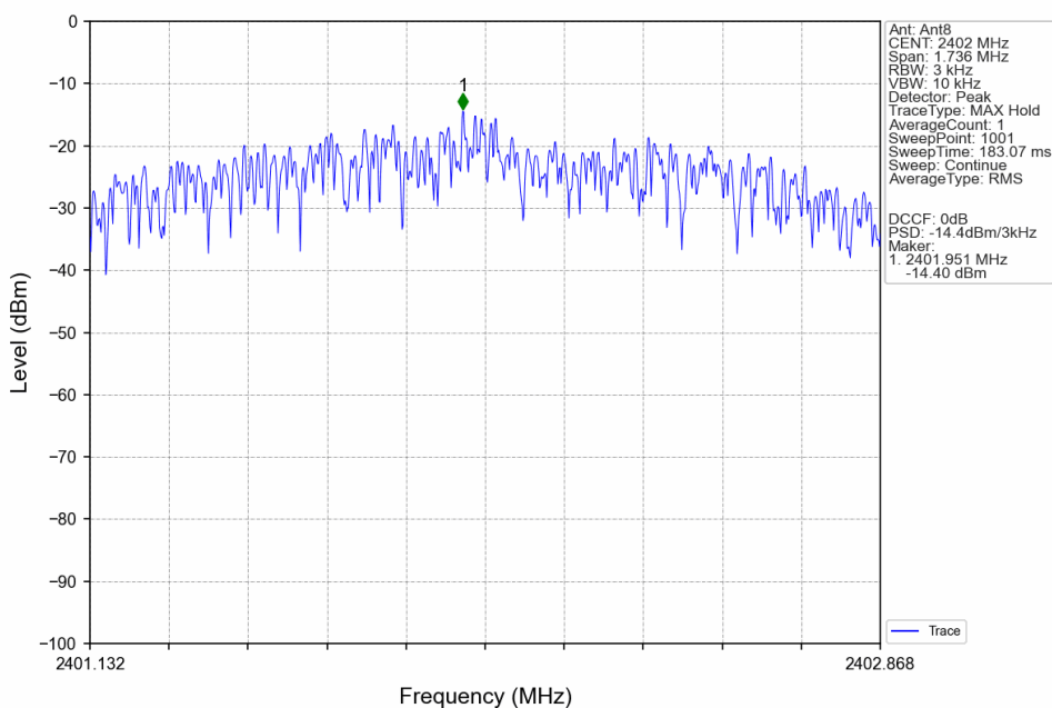
2M_LCH_2402MHz_Ant8_NTNV
