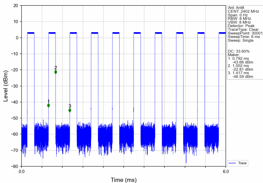
2M_LCH_2402MHz_Ant8_NTNV
