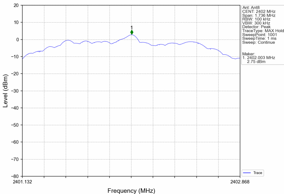
2M_LCH_2402MHz_Ant8_NTNV
