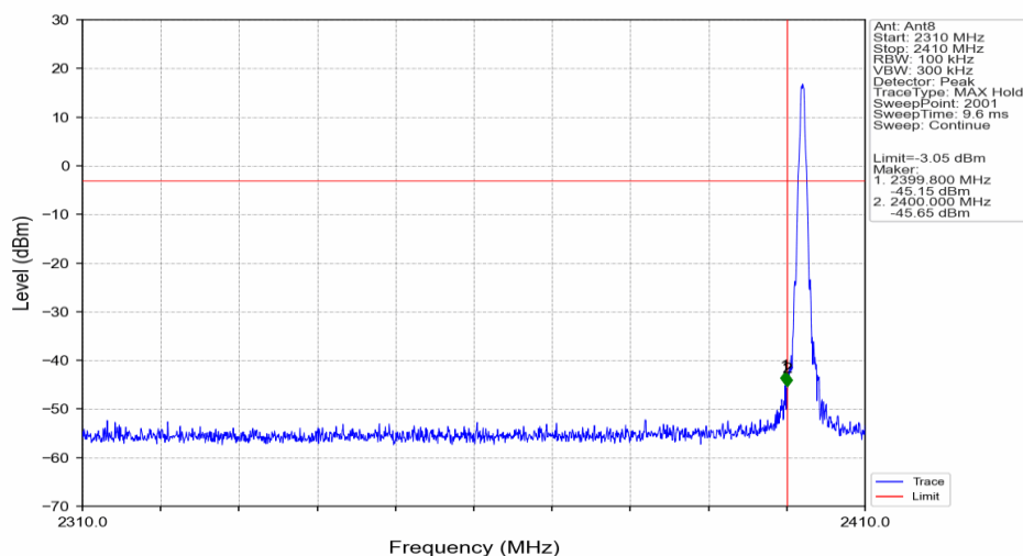
GFSK_DH5_LCH_2402MHz_Ant8_NTNV
