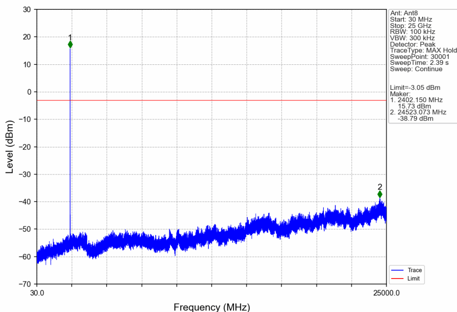
GFSK_DH5_LCH_2402MHz_Ant8_NTNV
