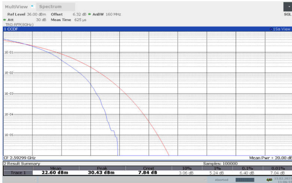
n41, DFT-s-pi/2 BPSK (PAPR)
