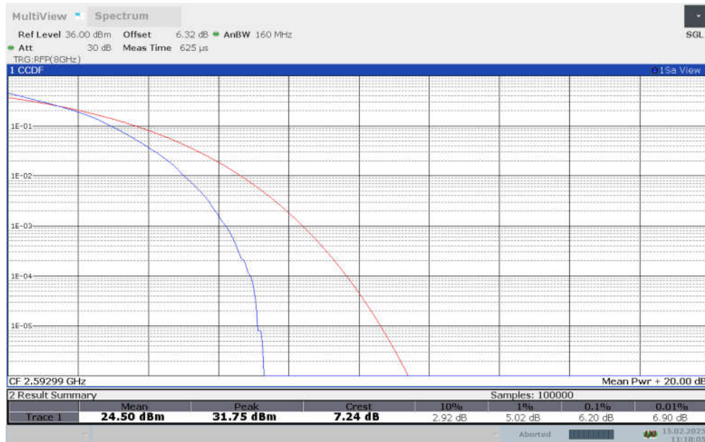
n41, DFT-s-64QAM (PAPR)
