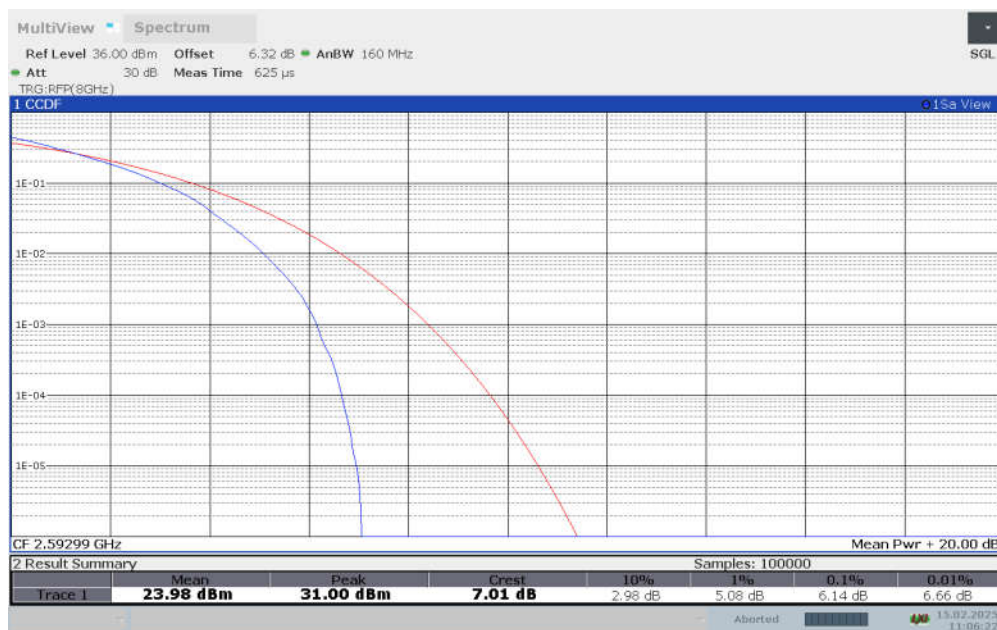
n41, DFT-s-256QAM (PAPR)
