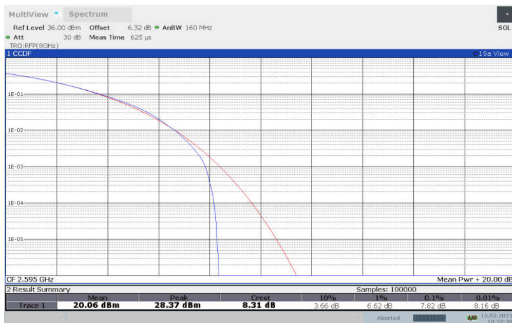
n38, DFT-s-16QAM (PAPR)
