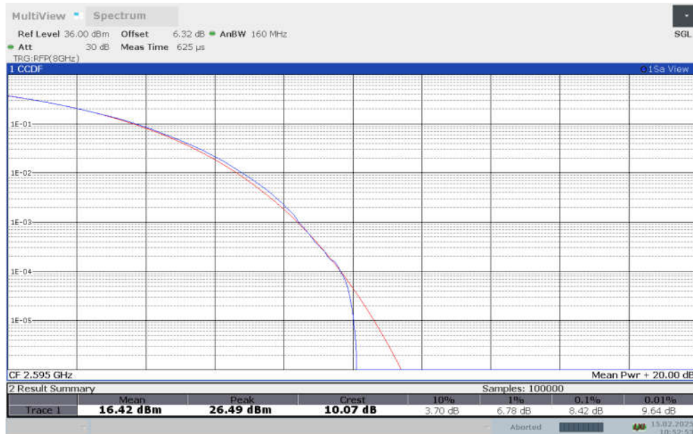
n38, CP-QPSK (PAPR)
