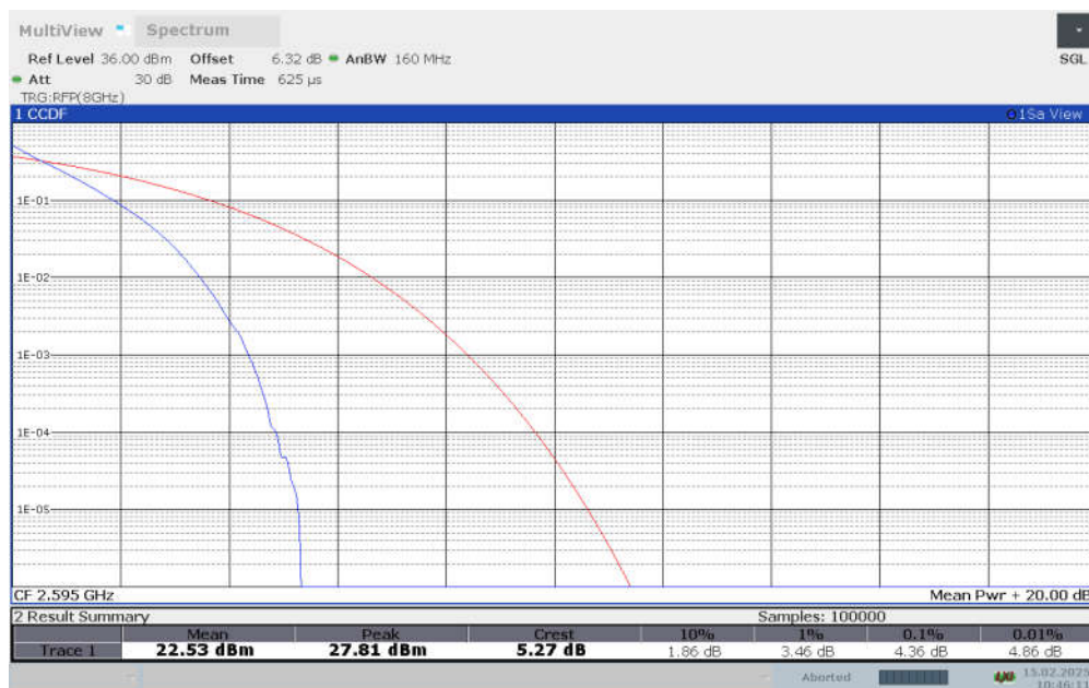
n38, DFT-s-QPSK (PAPR)
