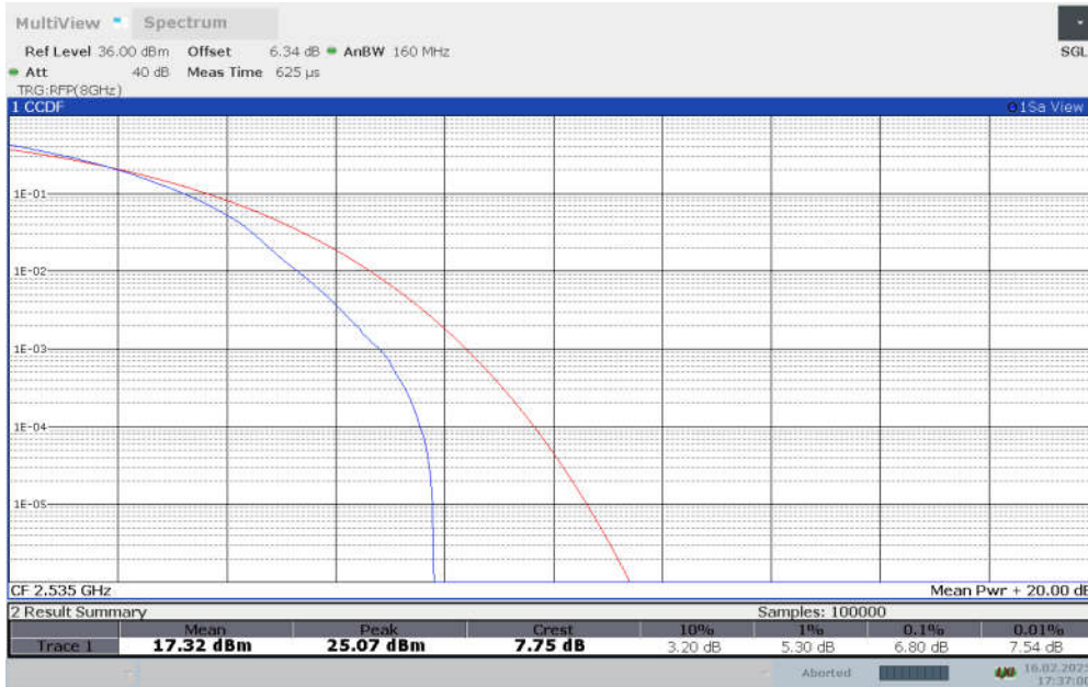
n7, DFT-s-pi/2 BPSK (PAPR)
