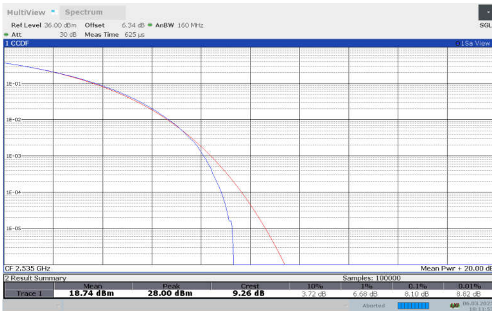
n7, CP-64QAM (PAPR)
