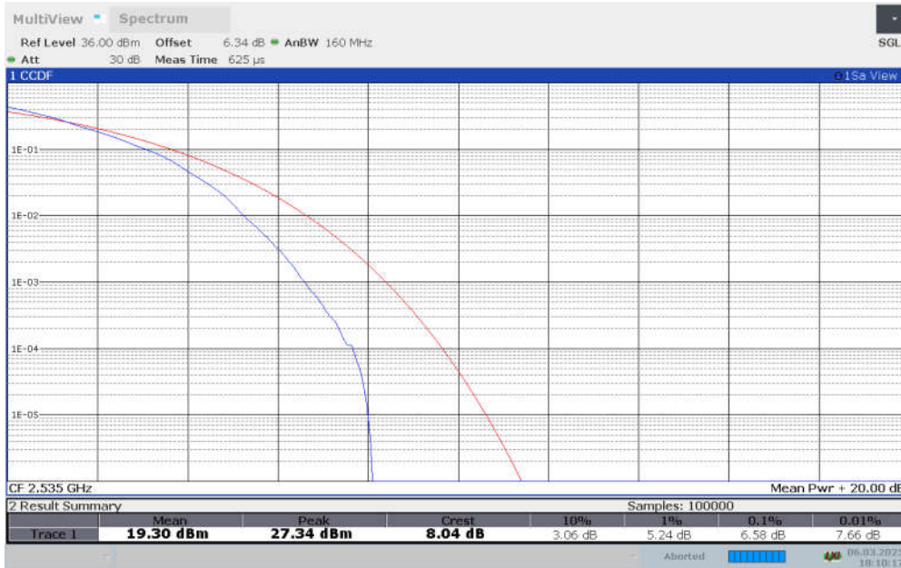
n7, DFT-s-256QAM (PAPR)
