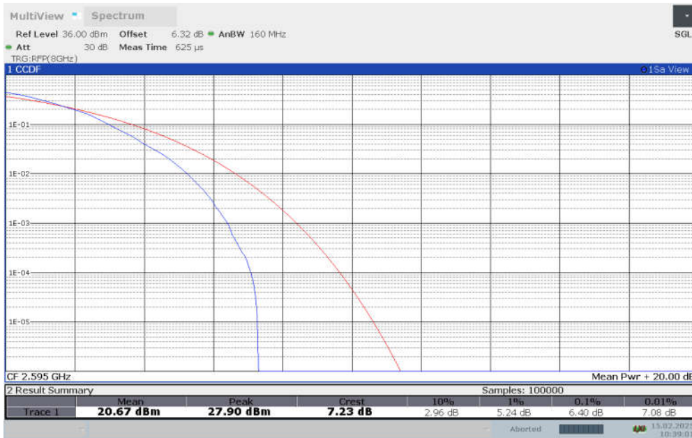
n38, DFT-s-256QAM (PAPR)
