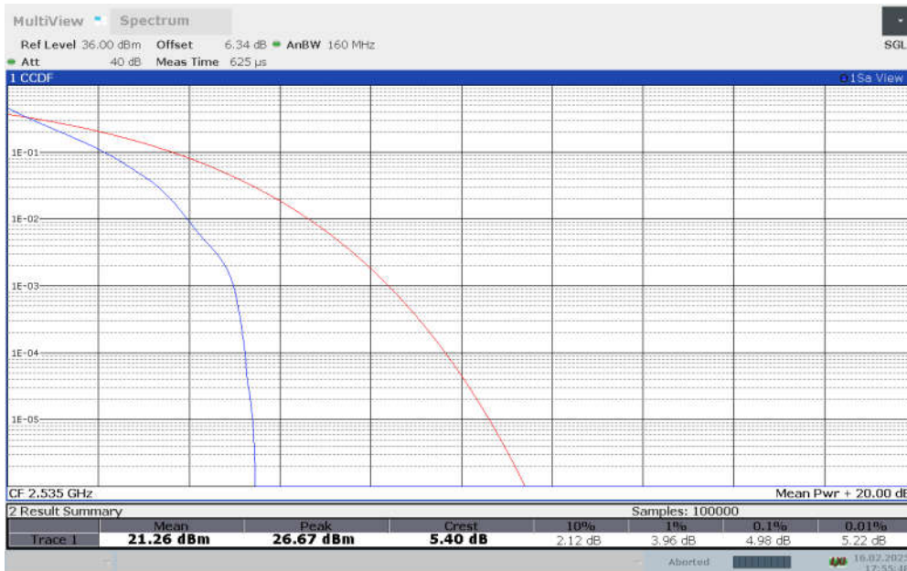
n7, DFT-s-QPSK (PAPR)
