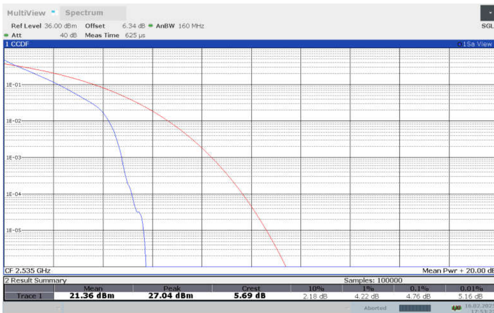
n7, DFT-s-QPSK (PAPR)
