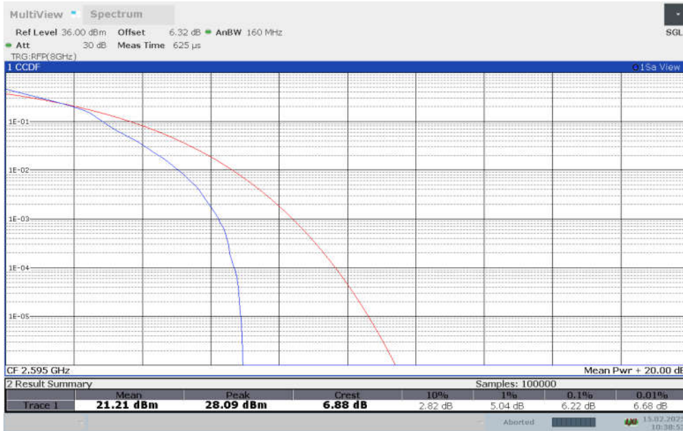
n38, DFT-s-64QAM (PAPR)
