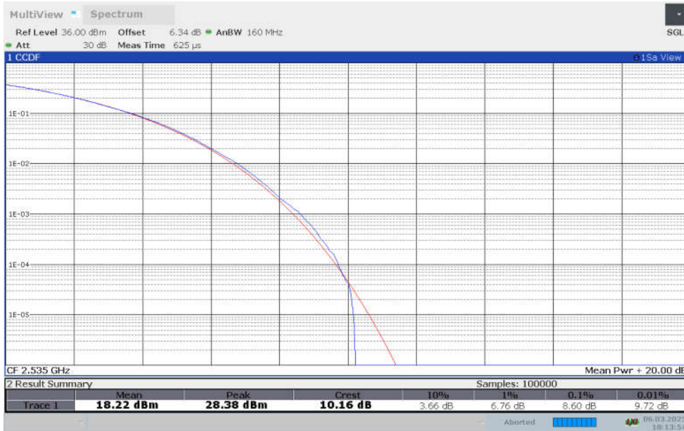
n7, CP-256QAM (PAPR)
