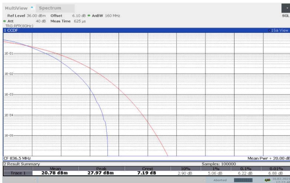
n5, DFT-s-256QAM (PAPR)
