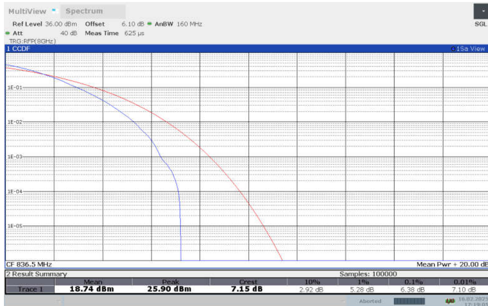
n5, DFT-s-pi/2 BPSK (PAPR)
