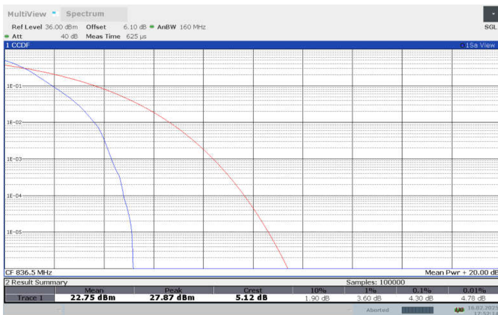
n5, DFT-s-QPSK (PAPR)
