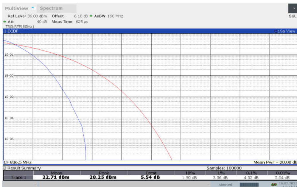
n5, DFT-s-QPSK (PAPR)
