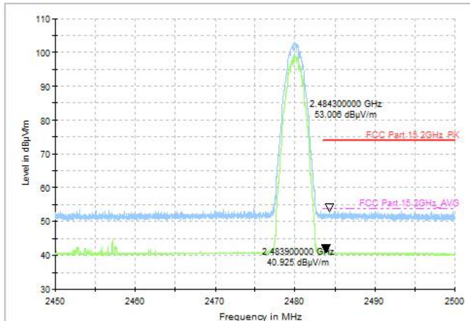
Fig. 37 Radiated Band Edges (8DPSK, CH78, 2.45GHz~2.50GHz)
