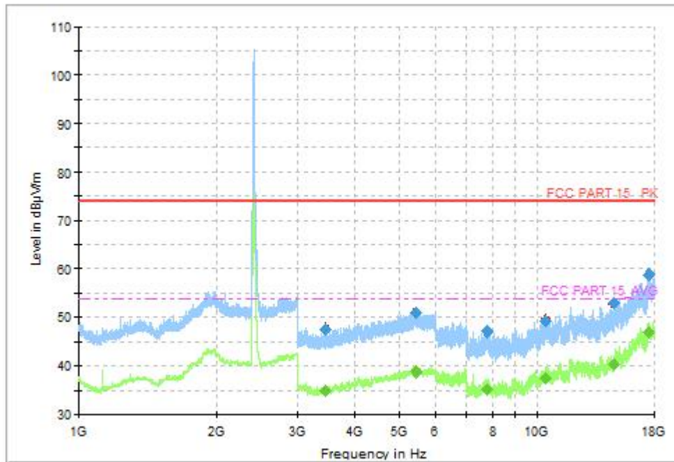
Fig.28 Radiated Spurious Emission (802.11n-HT20, CH1, 1GHz-18GHz, MIMO)
