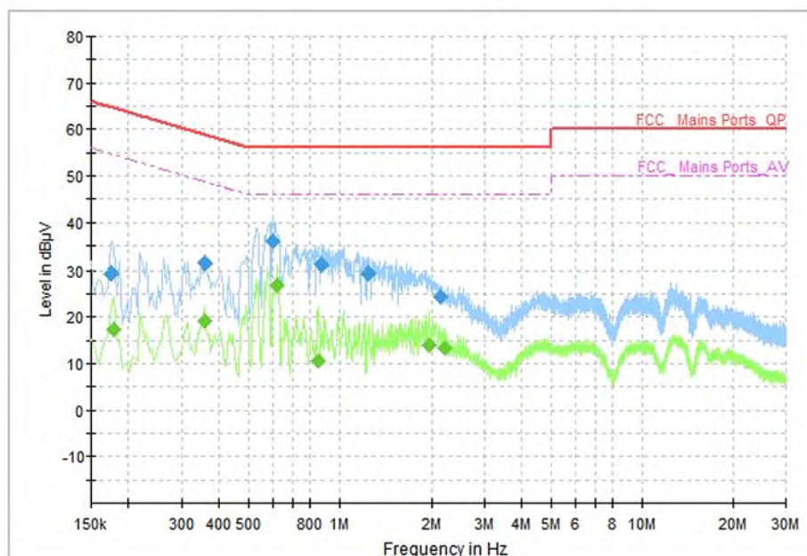
Fig.52 AC Power line Conducted Emission (Idle)
