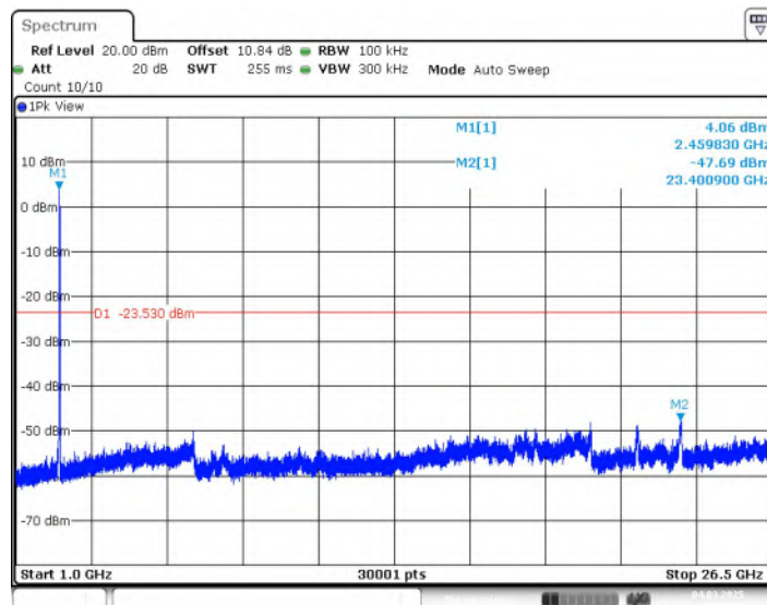
Fig.26 Conducted Spurious Emission (1GHz-26.5GHz, 802.11be-EHT20, CH11)
