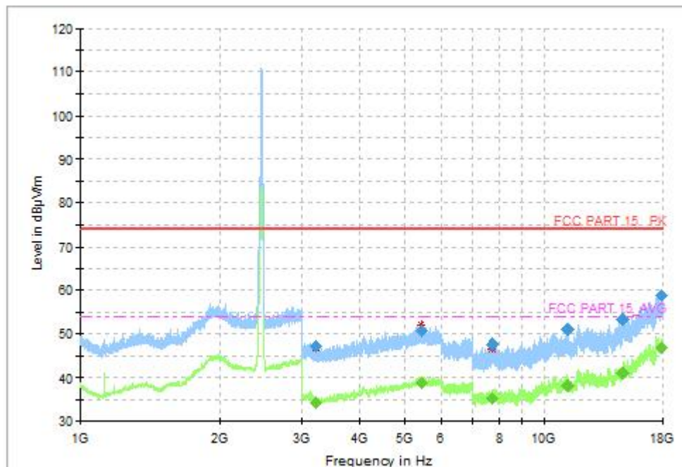
Fig.40 Radiated Spurious Emission (802.11ax-HE20, CH11, 1GHz-18GHz, MIMO)
