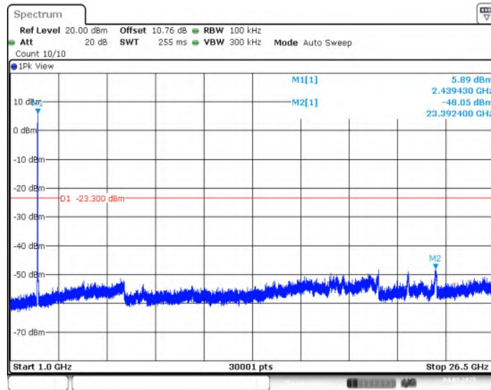
Fig.25 Conducted Spurious Emission (1GHz-26.5GHz, 802.11be-EHT20, CH6)
