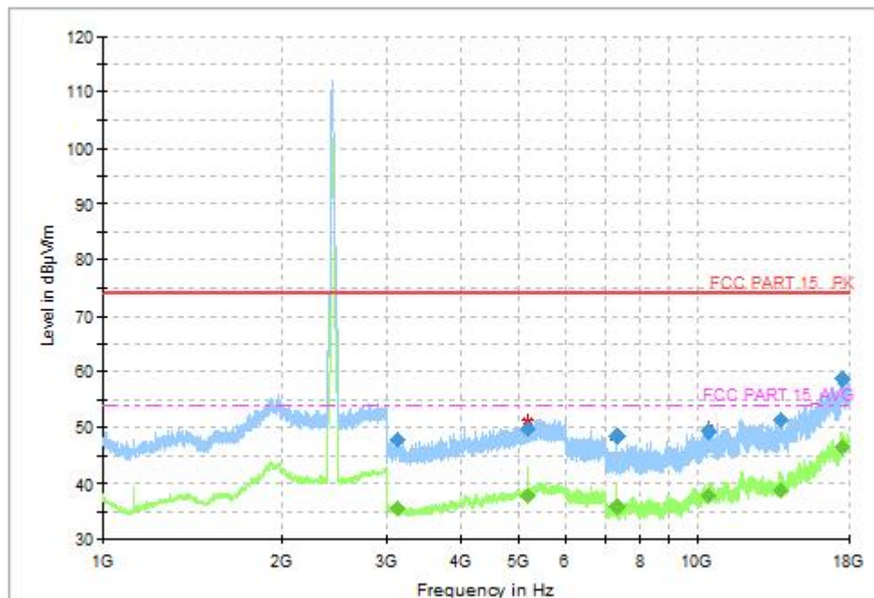
Fig.44 Radiated Spurious Emission (802.11be-EHT20, CH6, 1GHz-18GHz, MIMO)
