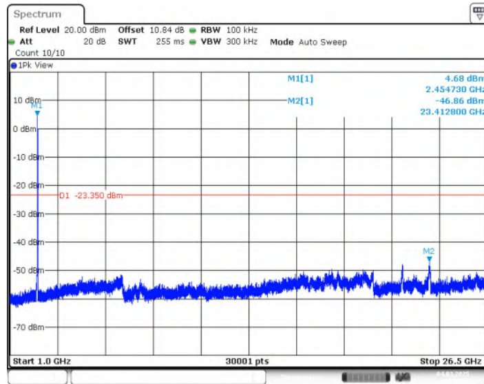
Fig.23 Conducted Spurious Emission (1GHz-26.5GHz, 802.11ax-HE20, CH11)
