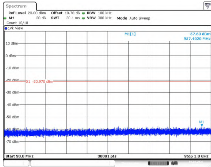
Fig.27 Conducted Spurious Emission (All Channels, 30MHz -1GHz)
