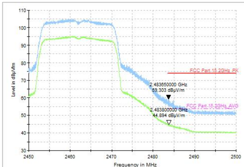
Fig.32 Radiated Restricted Band (802.11n-HT20, CH11, 2.45GHz~2.50GHz, MIMO)
