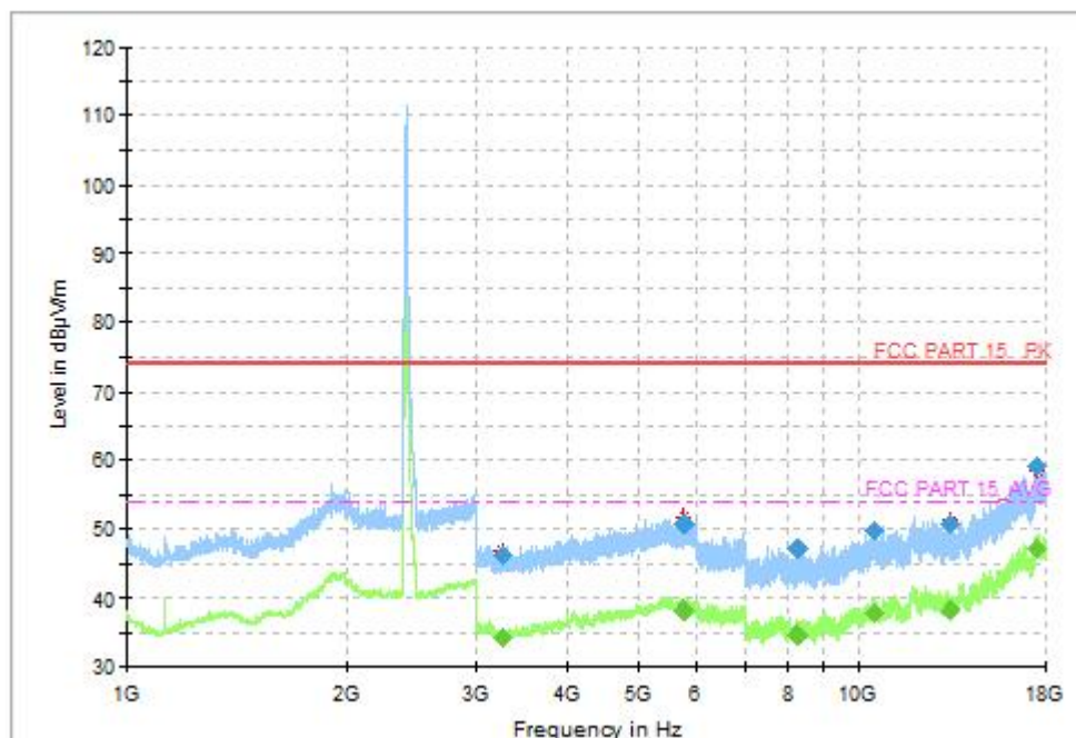
Fig.39 Radiated Spurious Emission (802.11ax-HE20, CH6, 1GHz-18GHz, MIMO)
