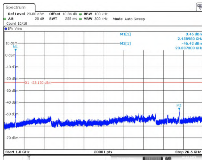
Fig.14 Conducted Spurious Emission (1GHz-26.5GHz, 802.11g, CH11)
