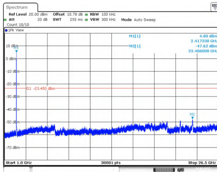
Fig.12 Conducted Spurious Emission (1GHz-26.5GHz, 802.11g, CH1)
