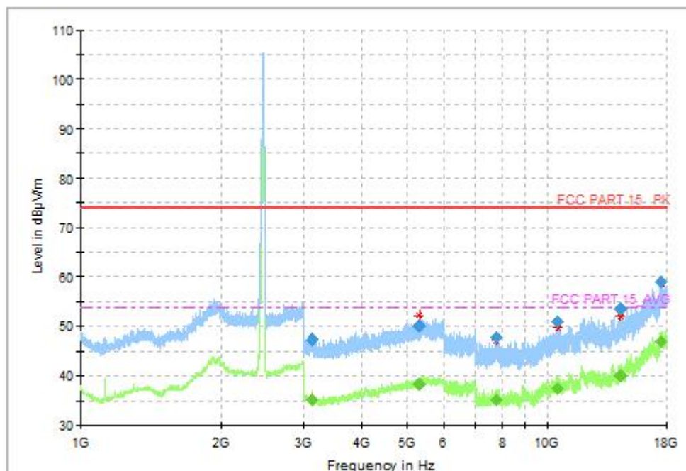
Fig.35 Radiated Spurious Emission (802.11-VHT20, CH11, 1GHz-18GHz, MIMO)
