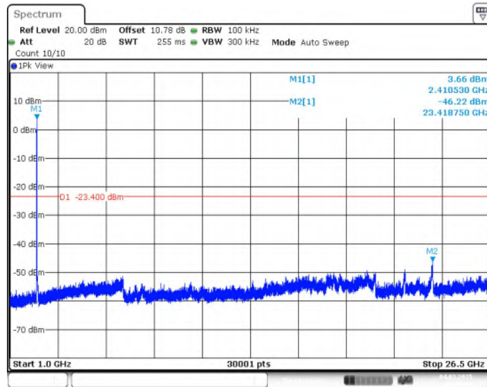
Fig.15 Conducted Spurious Emission (1GHz-26.5GHz, 802.11n-HT20, CH1)
