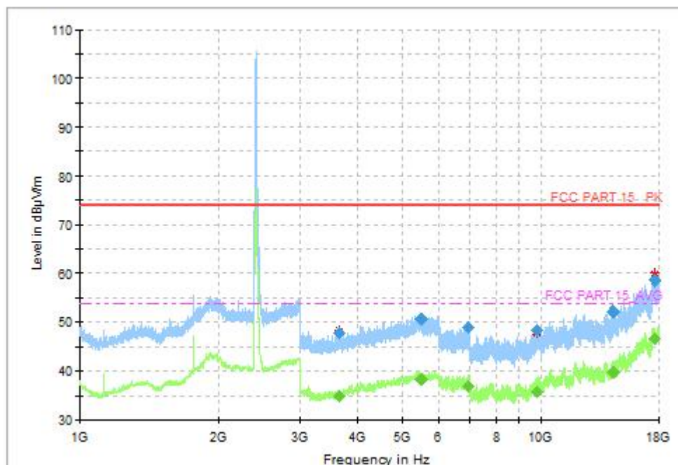
Fig.33 Radiated Spurious Emission (802.11-VHT20, CH1, 1GHz~18GHz, MIMO)
