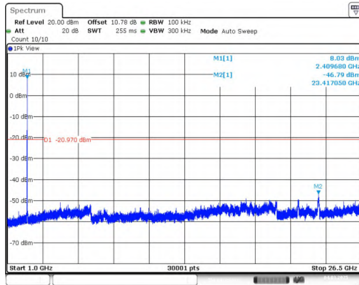
Fig.9 Conducted Spurious Emission (1GHz-26.5GHz, 802.11b, CH1)
