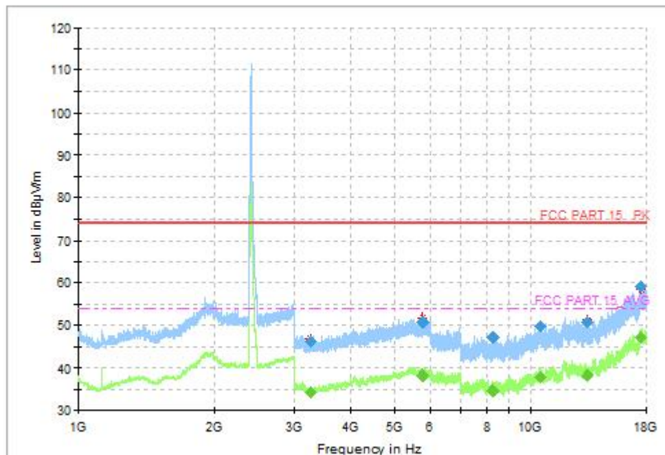
Fig.38 Radiated Spurious Emission (802.11ax-HE20, CH1, 1GHz-18GHz, MIMO)
