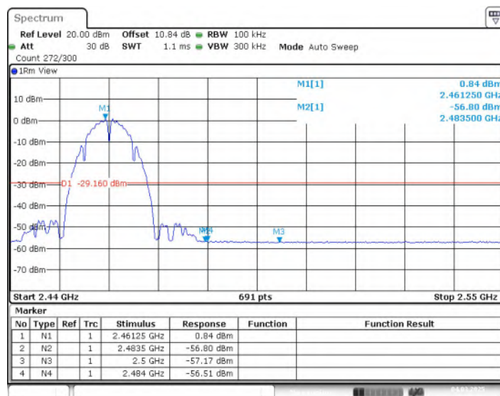
Fig.8 Band Edges (802.11b, CH11)
