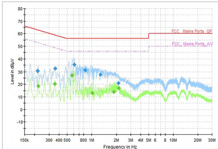
Fig.51 AC Power line Conducted Emission (Traffic)
