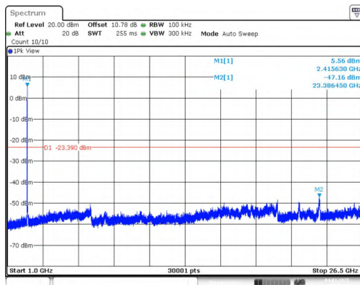
Fig.18 Conducted Spurious Emission (1GHz-26.5GHz, 802.11-VHT20, CH1)
