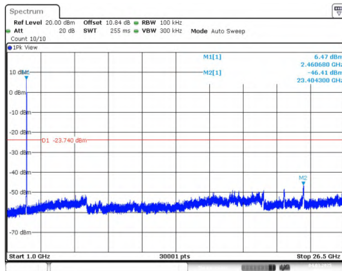
Fig.20 Conducted Spurious Emission (1GHz-26.5GHz, 802.11-VHT20, CH11)
