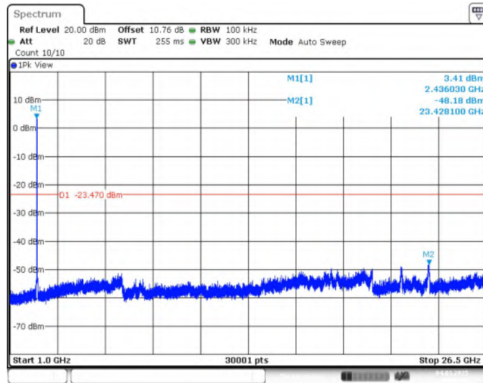
Fig.13 Conducted Spurious Emission (1GHz-26.5GHz, 802.11g, CH6)
