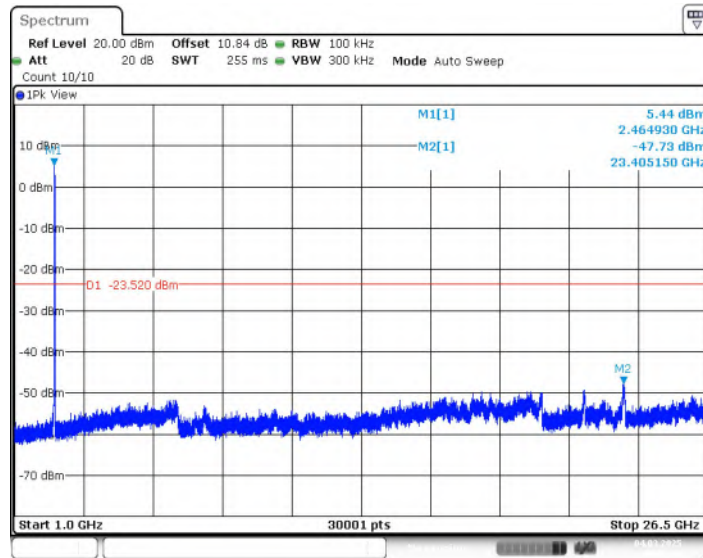
Fig.17 Conducted Spurious Emission (1GHz-26.5GHz, 802.11n-HT20, CH11)
