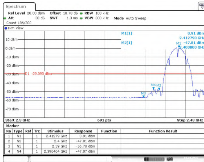
Fig.7 Band Edges (802.11b, CH1)
