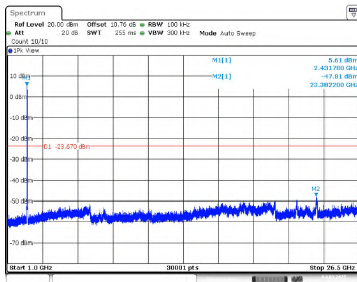
Fig.16 Conducted Spurious Emission (1GHz-26.5GHz, 802.11n-HT20, CH6)
