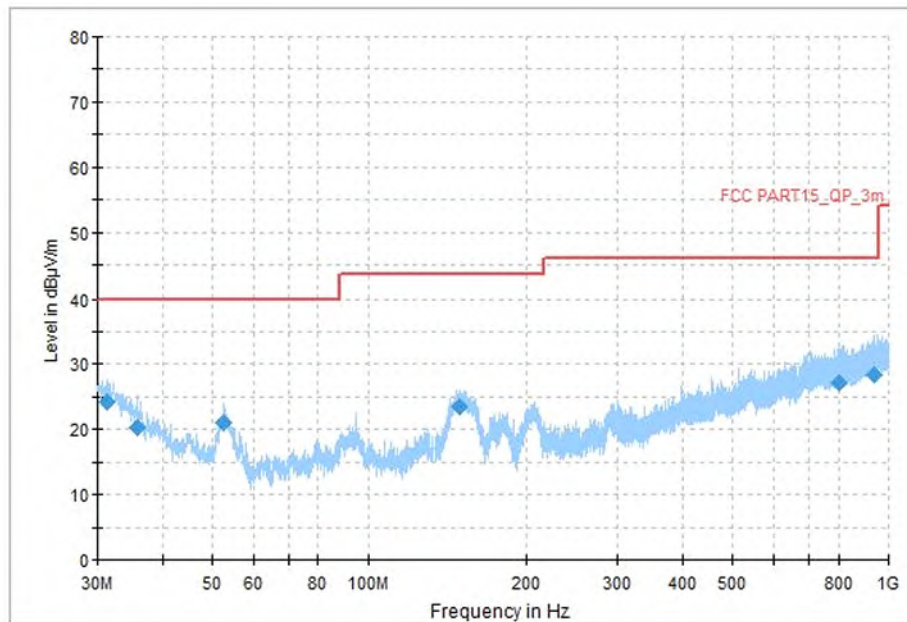
Fig.49 Radiated Spurious Emission (All Channels, 30MHz-1GHz, MIMO)
