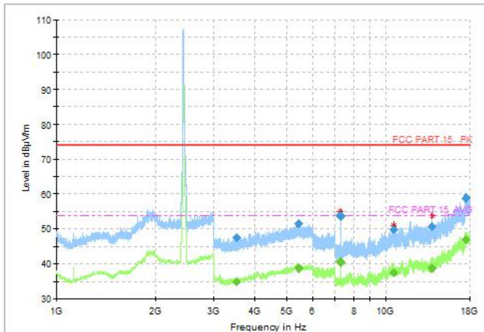
Fig.29 Radiated Spurious Emission (802.11n-HT20, CH6, 1GHz-18GHz, MIMO)
