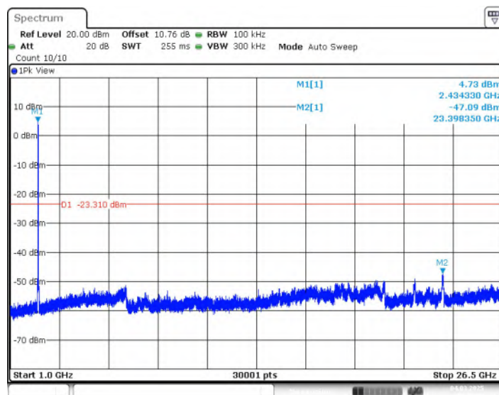
Fig.22 Conducted Spurious Emission (1GHz-26.5GHz, 802.11ax-HE20, CH6)
