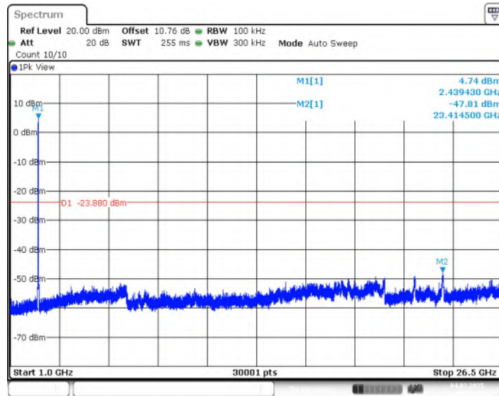
Fig.19 Conducted Spurious Emission (1GHz-26.5GHz, 802.11-VHT20, CH6)
