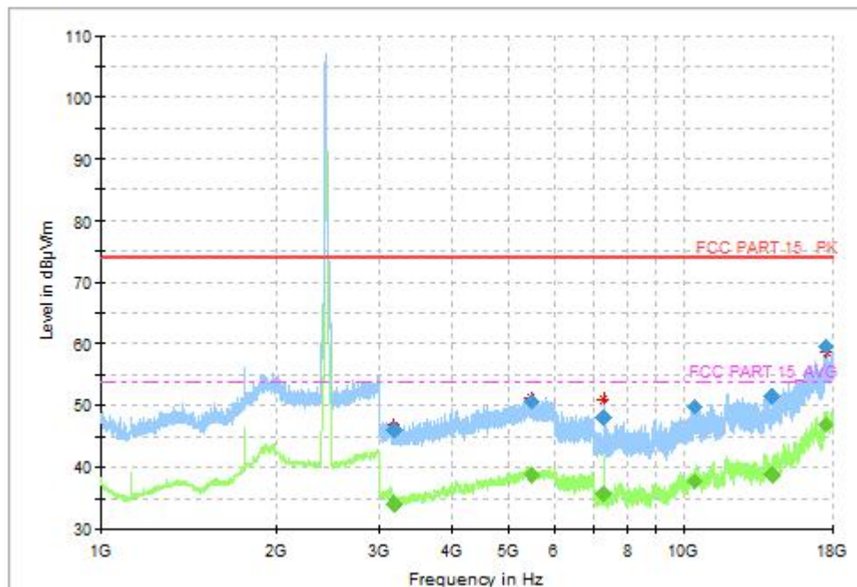
Fig.34 Radiated Spurious Emission (802.11-VHT20, CH6, 1GHz-18GHz, MIMO)
