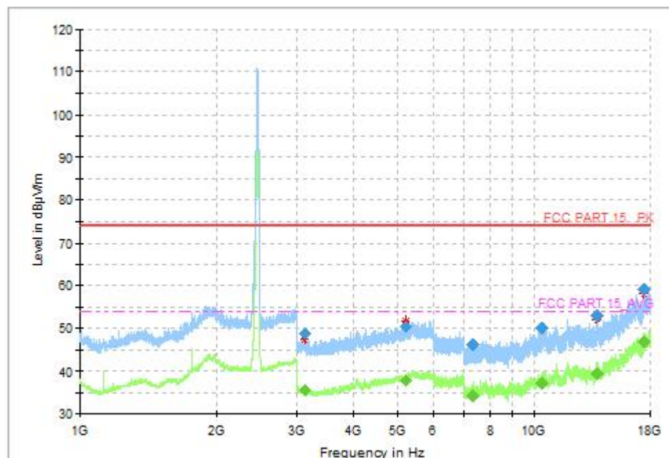
Fig.43 Radiated Spurious Emission (802.11be-EHT20, CH1, 1GHz-18GHz, MIMO)
