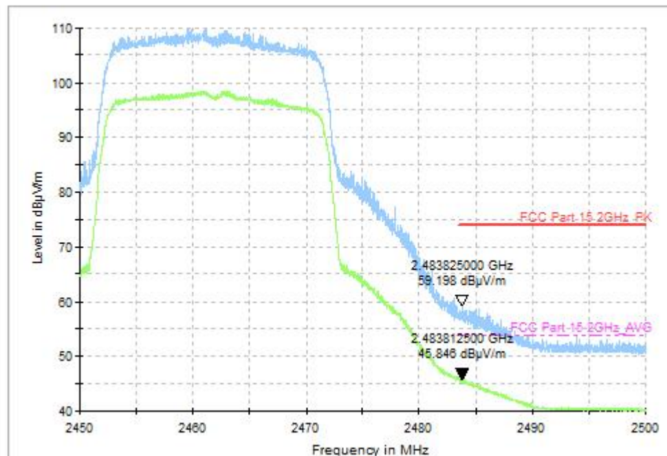
Fig.42 Radiated Restricted Band (802.11ax-HE20, CH11, 2.45GHz~2.50GHz, MIMO)
