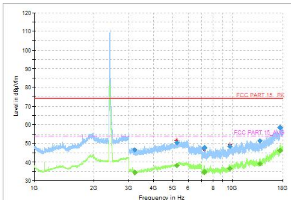
Fig.45 Radiated Spurious Emission (802.11be-EHT20, CH11, 1GHz-18GHz, MIMO)
