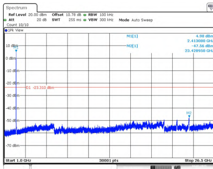
Fig.24 Conducted Spurious Emission (1GHz-26.5GHz, 802.11be-EHT20, CH1)
