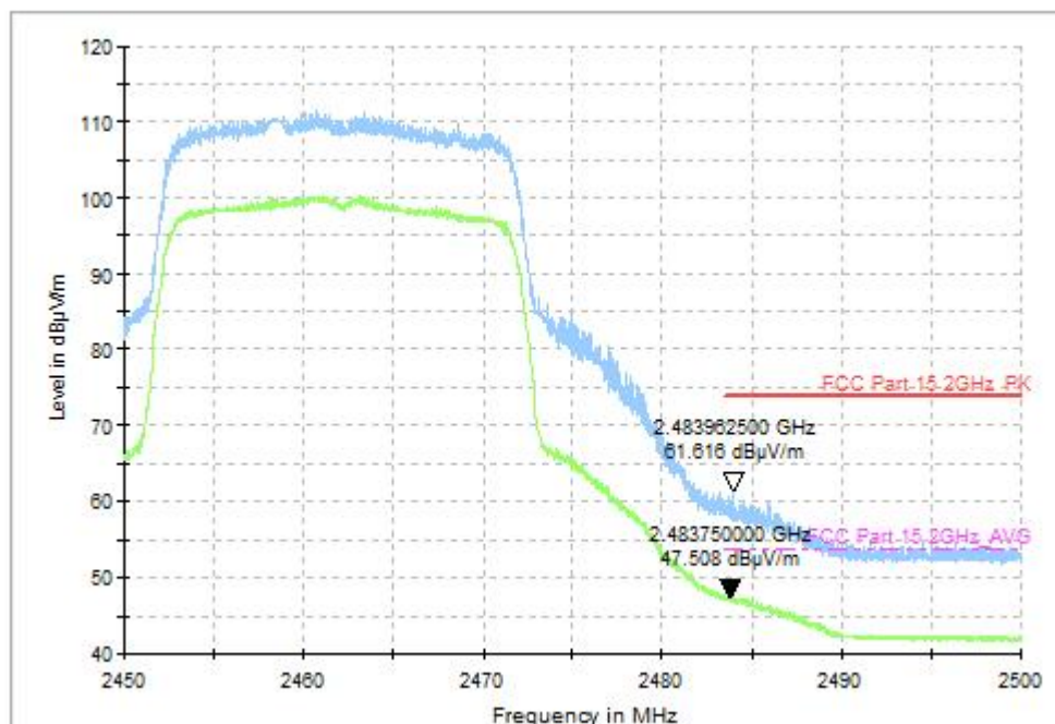
Fig.47 Radiated Restricted Band (802.11be-EHT20, CH11, 2.45GHz~2.50GHz, MIMO)
