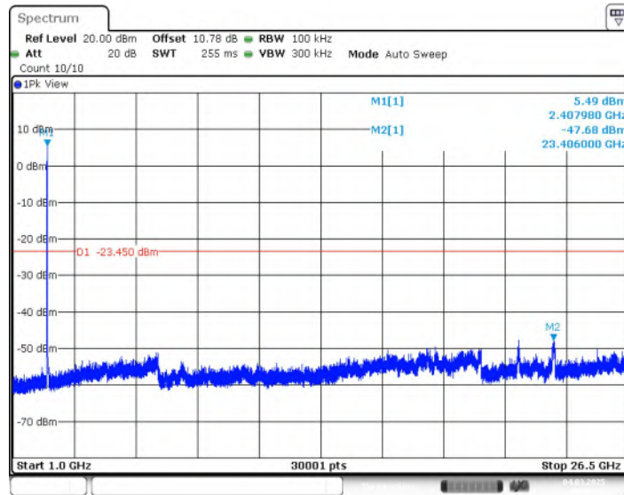
Fig.21 Conducted Spurious Emission (1GHz-26.5GHz, 802.11ax-HE20, CH1)
