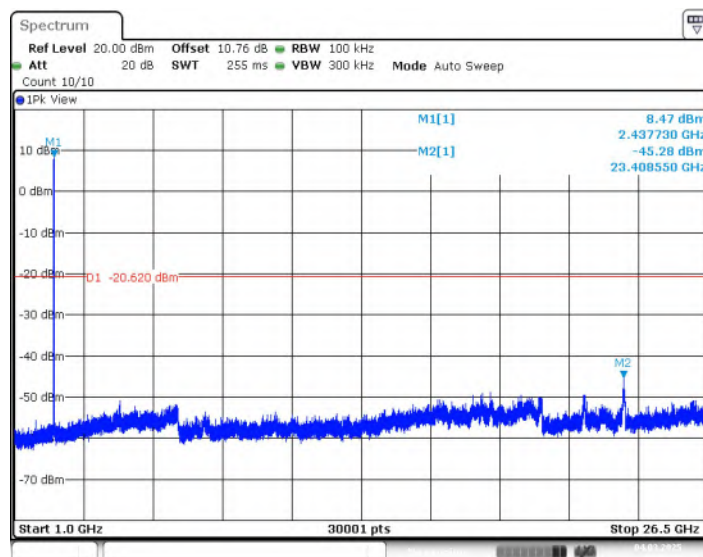
Fig.10 Conducted Spurious Emission (1GHz-26.5GHz, 802.11b, CH6)
