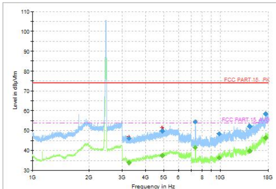
Fig.30 Radiated Spurious Emission (802.11n-HT20, CH11, 1GHz-18GHz, MIMO)
