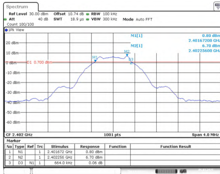
Fig.7 6dB Bandwidth (CH0), LE 1M
