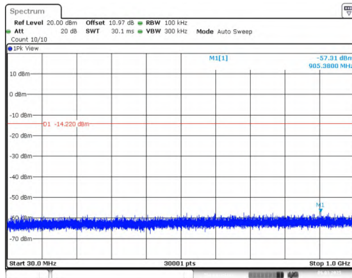
Fig.23 Conducted Spurious Emission (All Channels, 30MHz -1GHz)
