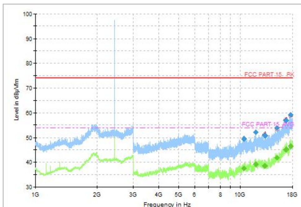
Fig.25 Radiated Spurious Emission (CH19, 1GHz ~18GHz), LE 1M
