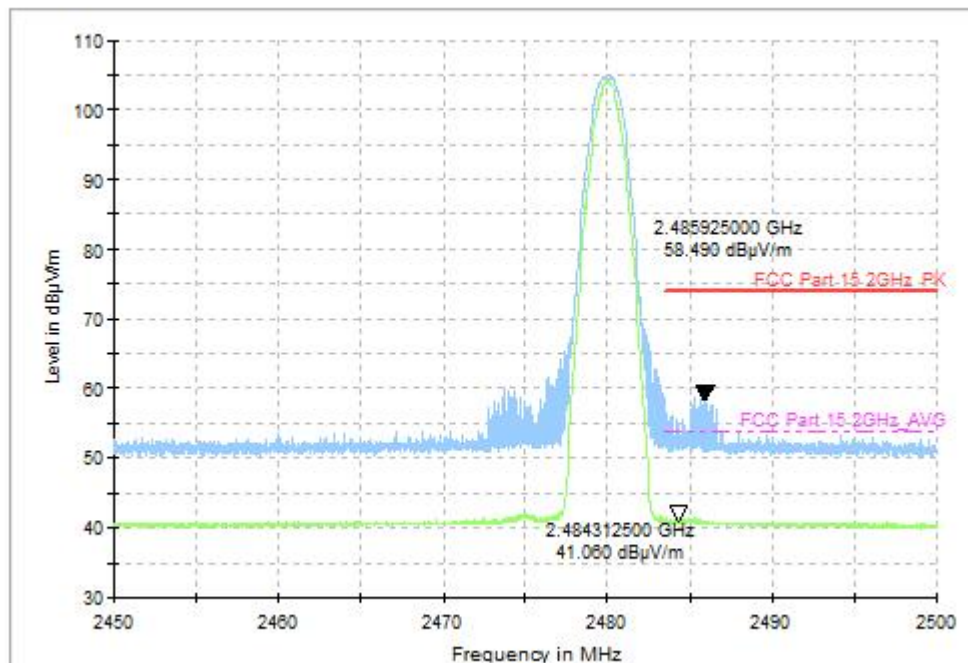
Fig.28 Radiated Band Edges (CH39, 2.45GHz~2.50GHz), LE 1M
