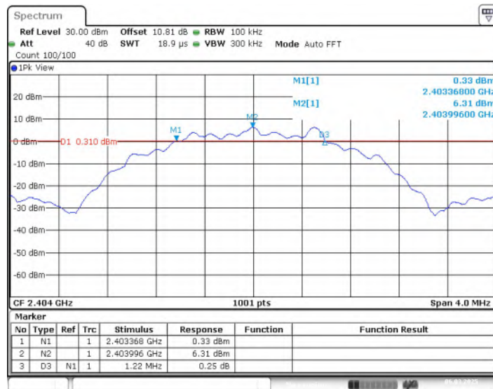
Fig.10 6dB Bandwidth (CH1), LE 2M
