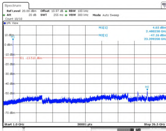
Fig.19 Conducted Spurious Emission (CH39, 1GHz-26.5GHz), LE 1M
