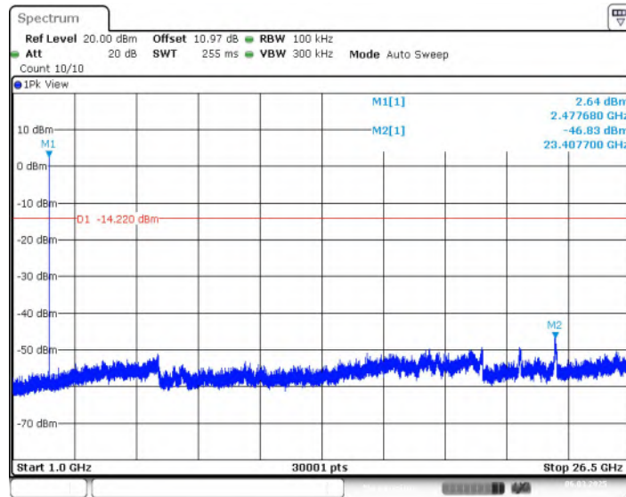
Fig.22 Conducted Spurious Emission (CH38, 1GHz-26.5GHz), LE 2M
