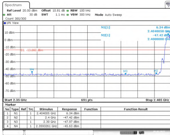
Fig.15 Band Edges (CH1), LE 2M
