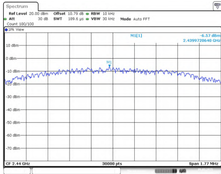
Fig.5 Power Spectral Density (CH19), LE 2M
