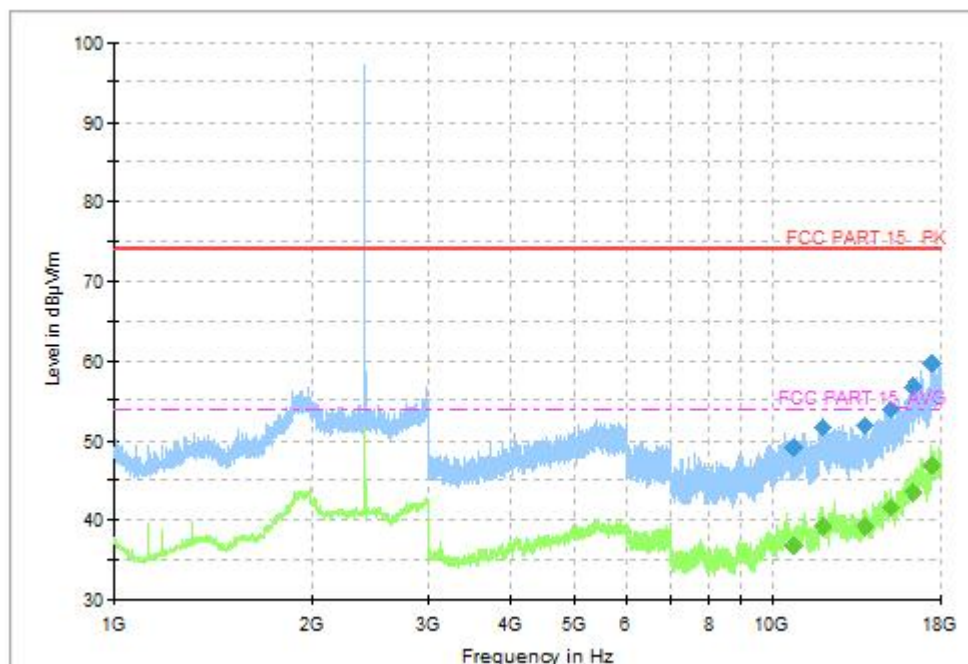
Fig.29 Radiated Spurious Emission (CH1, 1GHz ~18GHz), LE 2M
