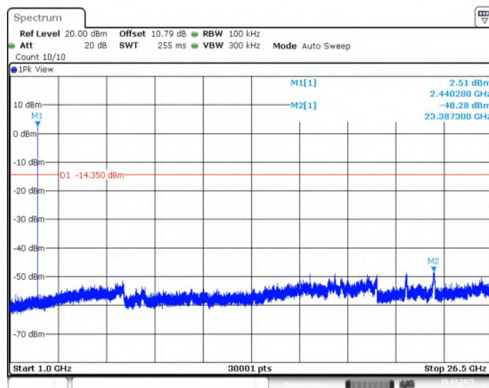
Fig.21 Conducted Spurious Emission (CH19, 1GHz-26.5GHz), LE 2M
