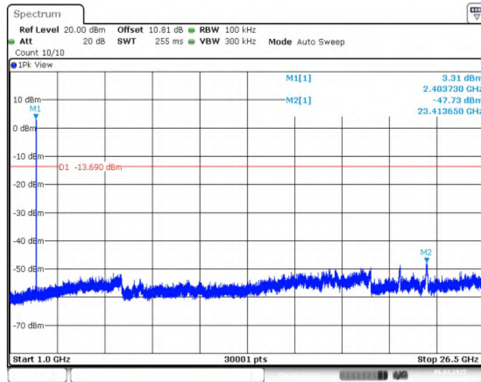
Fig.20 Conducted Spurious Emission (CH1, 1GHz-26.5GHz), LE 2M
