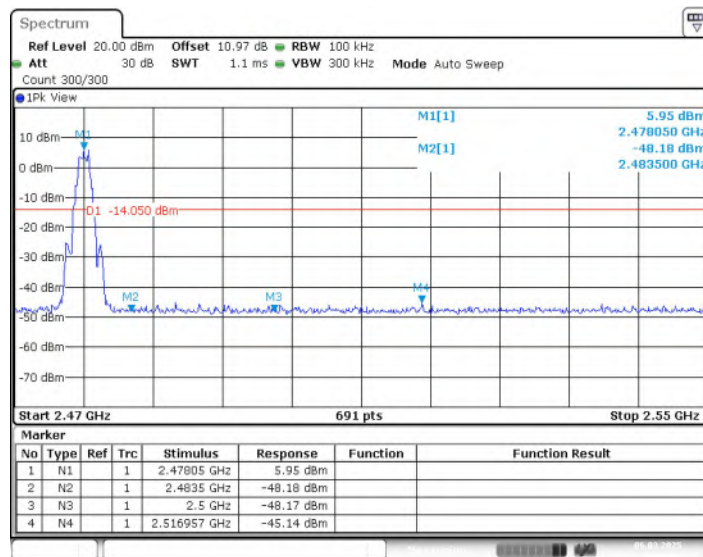
Fig.16 Band Edges (CH38), LE 2M
