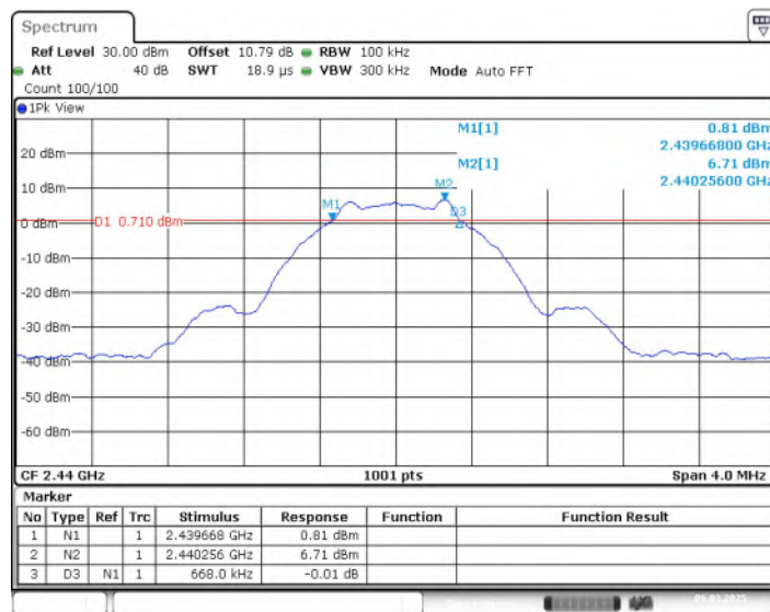
Fig.8 6dB Bandwidth (CH19), LE 1M
