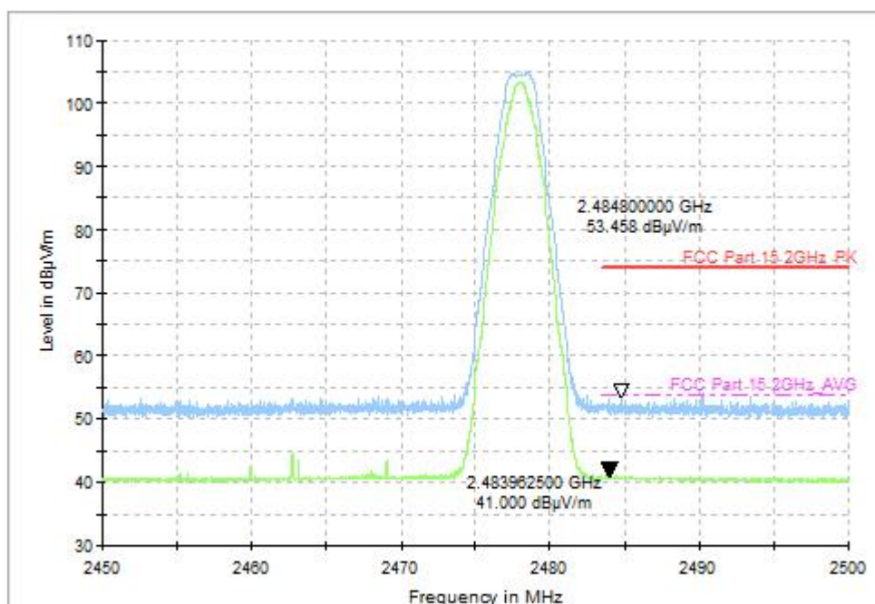
Fig.33 Radiated Band Edges (CH38, 2.45GHz~2.50GHz), LE 2M
