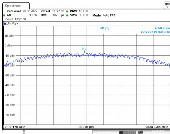
Fig.6 Power Spectral Density (CH38), LE 2M
