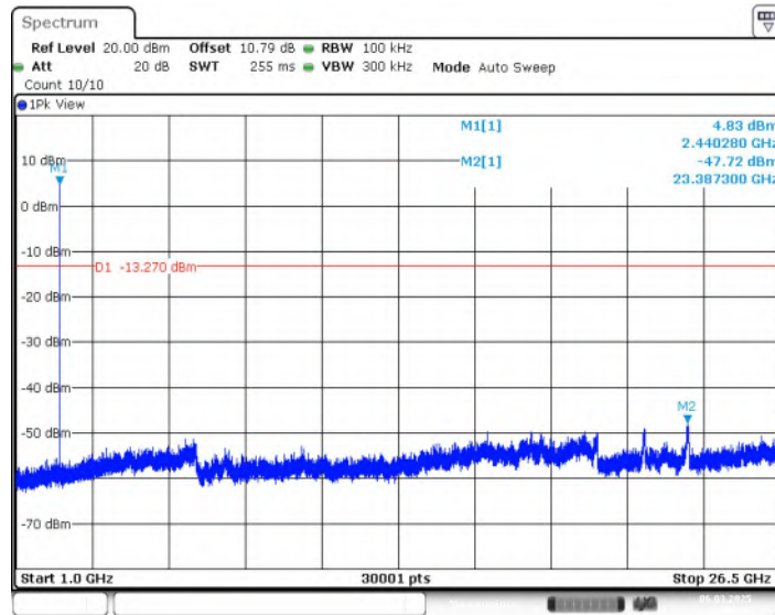
Fig.18 Conducted Spurious Emission (CH19, 1GHz-26.5GHz), LE 1M
