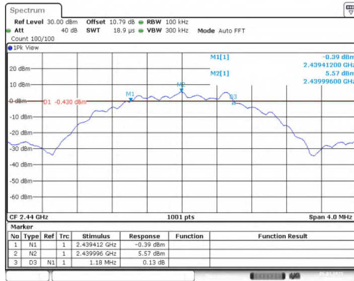
Fig.11 6dB Bandwidth (CH19), LE 2M
