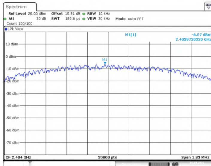
Fig.4 Power Spectral Density (CH1), LE 2M
