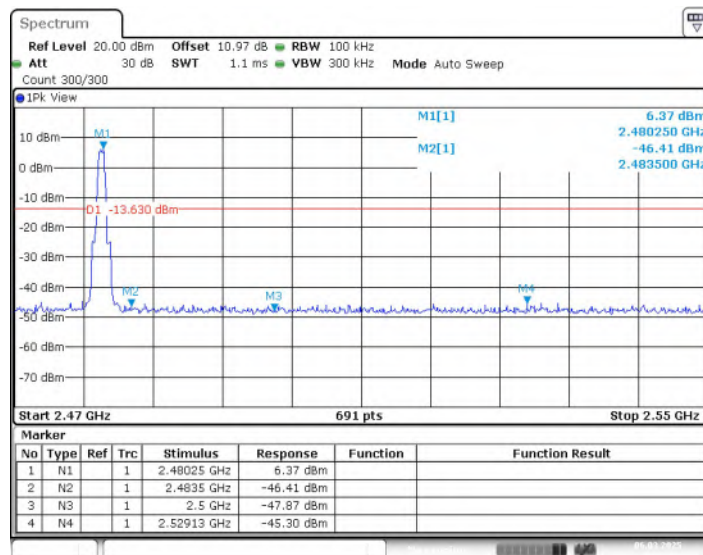
Fig.14 Band Edges (CH39), LE 1M
