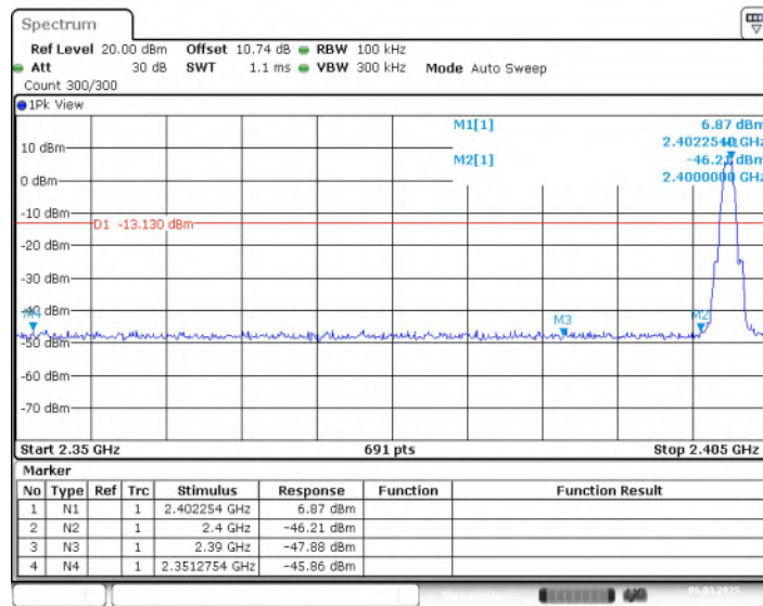
Fig.13 Band Edges (CH0), LE 1M
