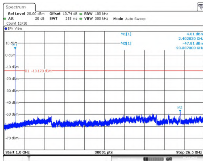
Fig.17 Conducted Spurious Emission (CH0, 1GHz-26.5GHz), LE 1M
