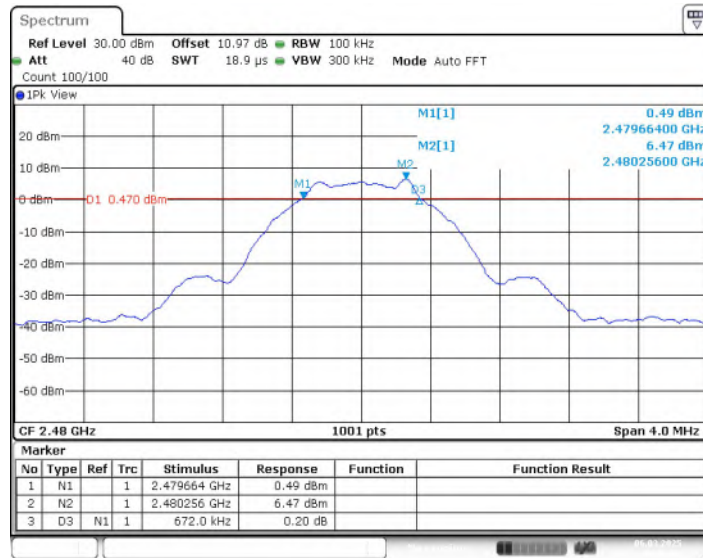
Fig.9 6dB Bandwidth (CH39), LE 1M
