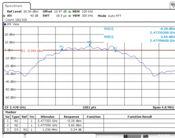
Fig.12 6dB Bandwidth (CH38), LE 2M
