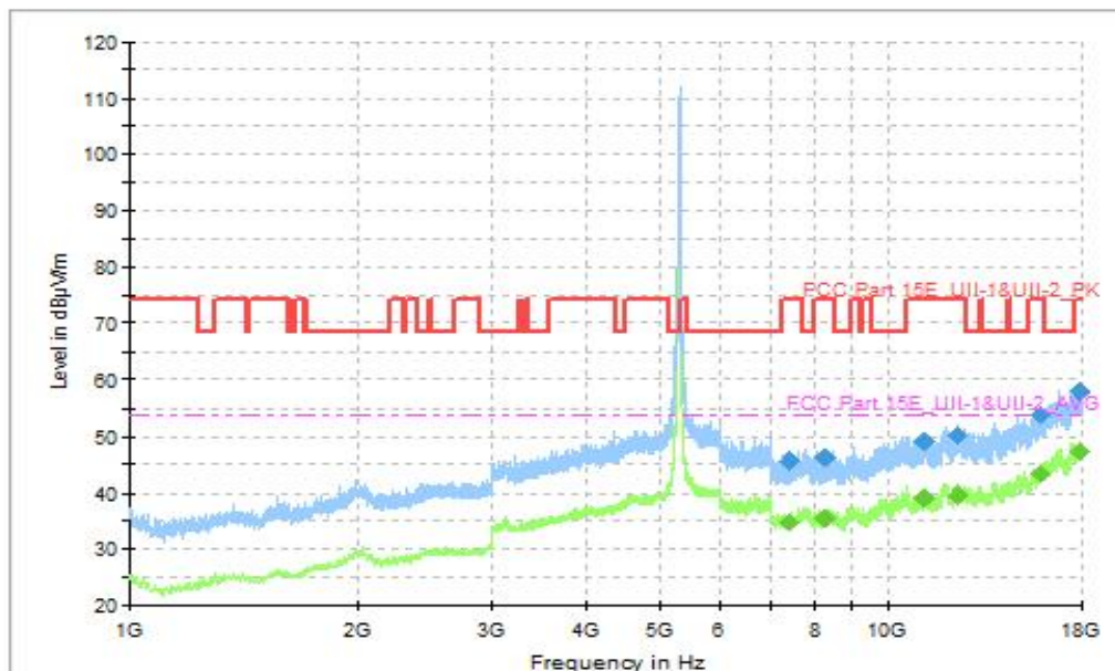
Fig. 61 Transmitter Spurious Emission (802.11be-EHT40, CH62 5310MHz, 1GHz-18GHz), MIMO
