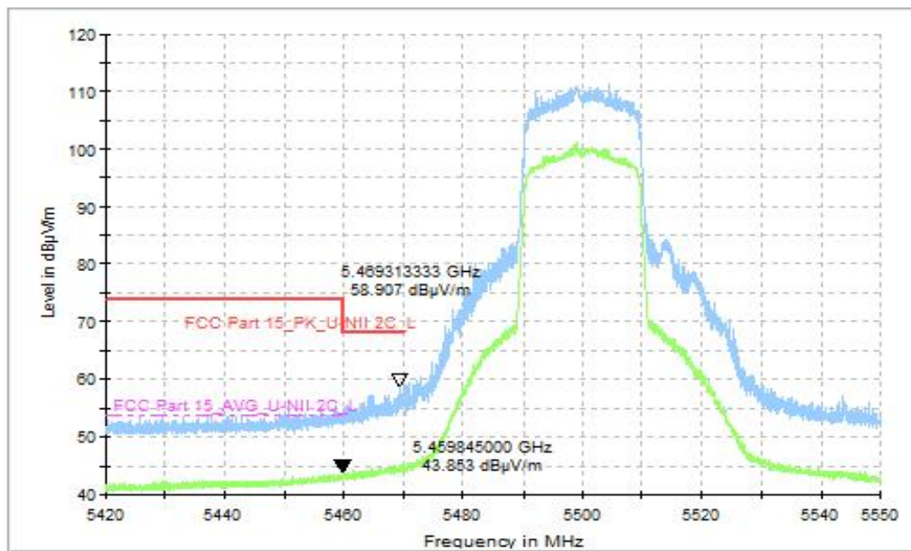
Fig. 29 Band Edges, CH100 5500MHz, MIMO
