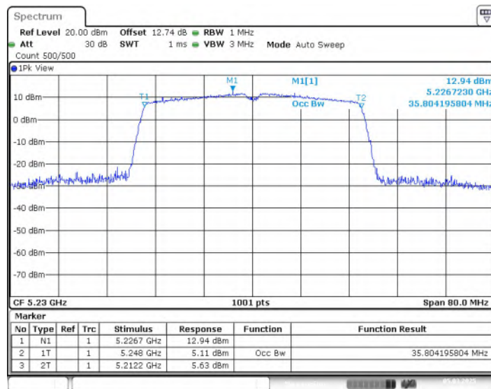
Fig. 18 99% Occupied Bandwidth (802.11n-HT40, 5230MHz)
