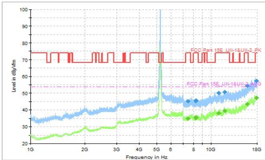
Fig. 59 Transmitter Spurious Emission (802.11be-EHT40, CH46 5230MHz, 1GHz-18GHz), MIMO
