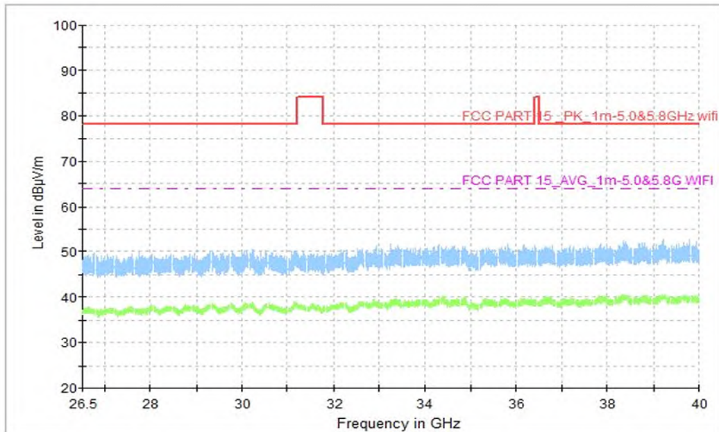
Fig. 76 Transmitter Spurious Emission (All channel, 26.5GHz~40GHz), MIMO
