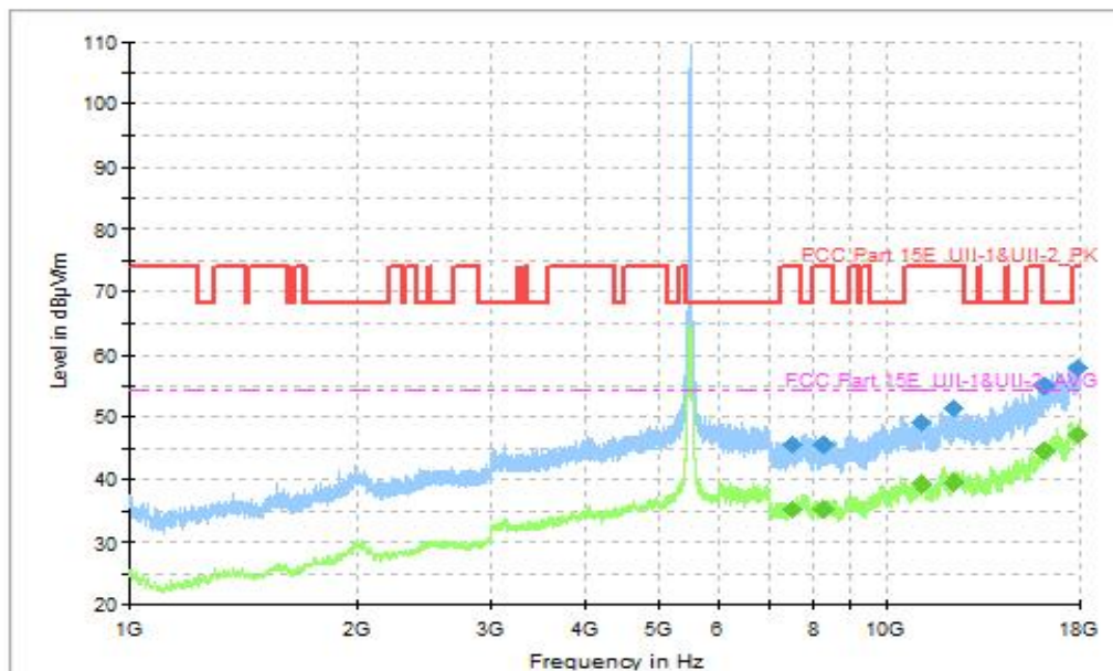
Fig. 62 Transmitter Spurious Emission (802.11be-EHT40, CH102 5510MHz, 1GHz-18GHz), MIMO
