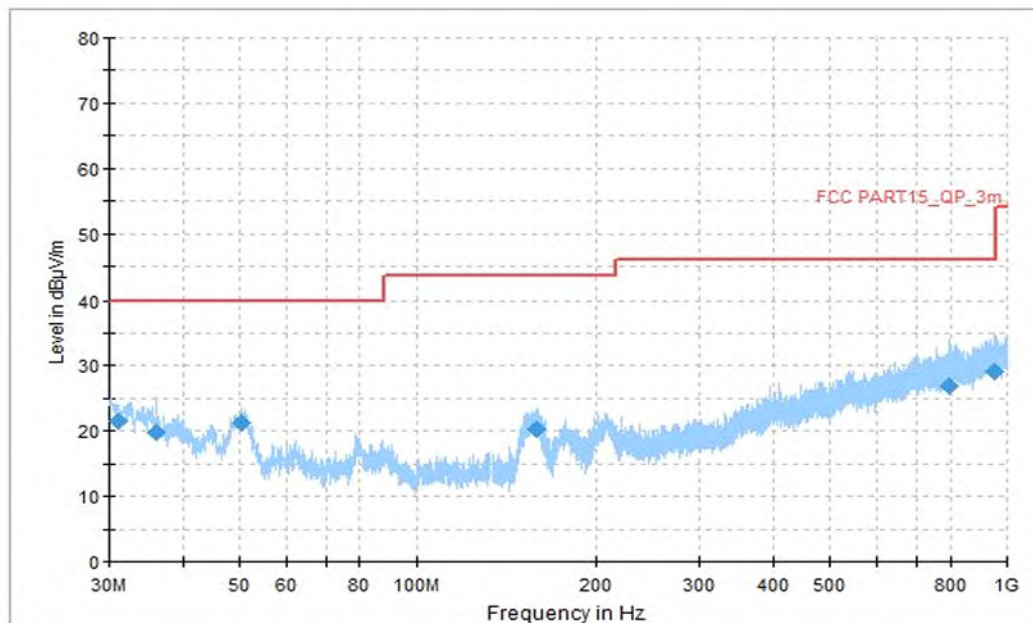
Fig. 74 Transmitter Spurious Emission (All channel, 30MHz~1GHz), MIMO
