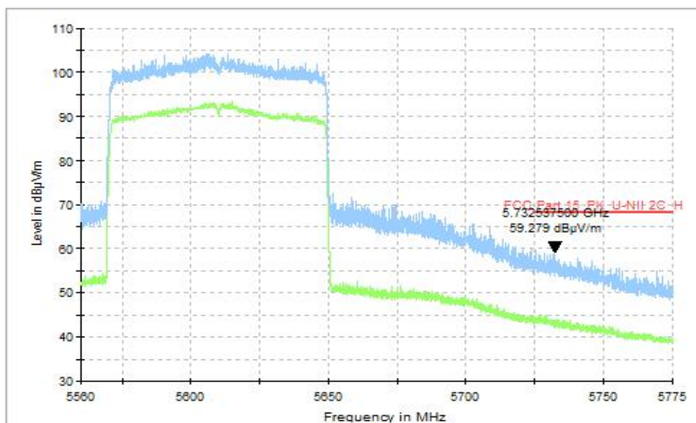
Fig. 42 Band Edges, CH122 5610MHz, MIMO
