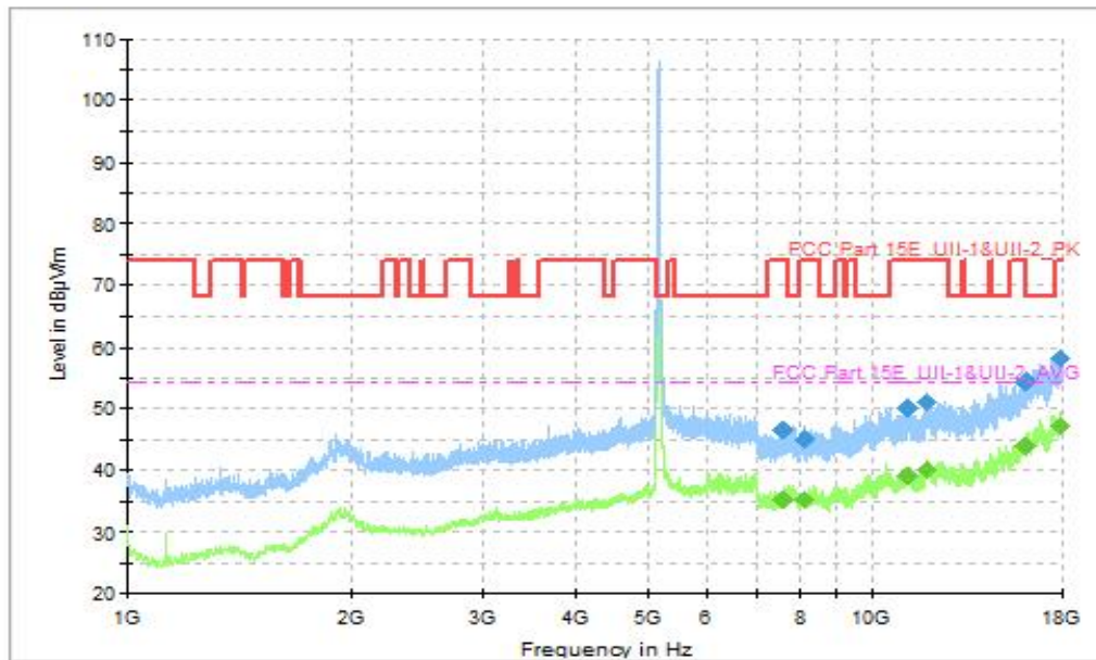
Fig. 46 Transmitter Spurious Emission (802.11be-EHT20, CH36 5180MHz, 1GHz-18GHz), MIMO
