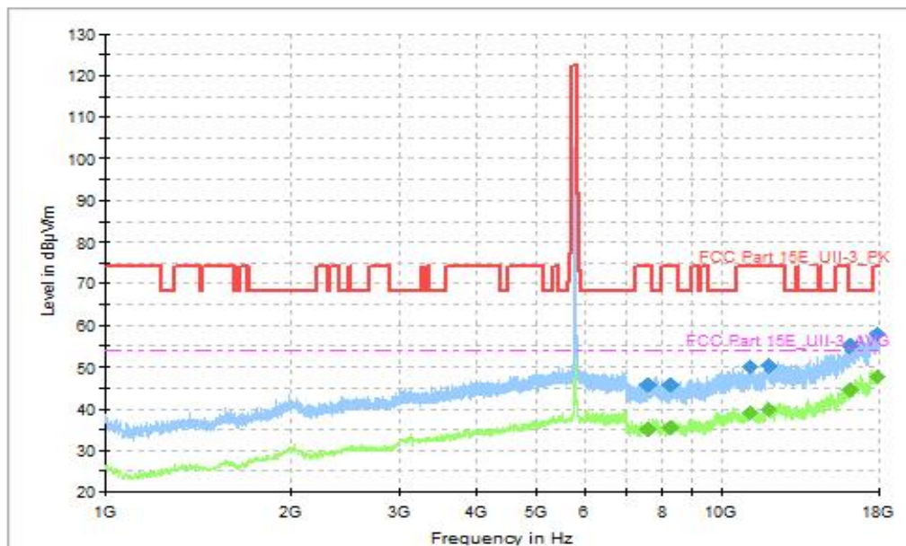
Fig. 66 Transmitter Spurious Emission (802.11be-EHT40, CH159 5795MHz, 1GHz-18GHz), MIMO
