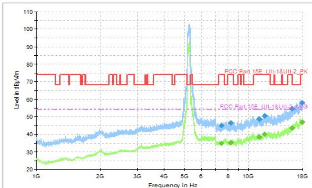
Fig. 72 Transmitter Spurious Emission (802.11be-EHT160, CH50 5250MHz, 1GHz-18GHz), MIMO
