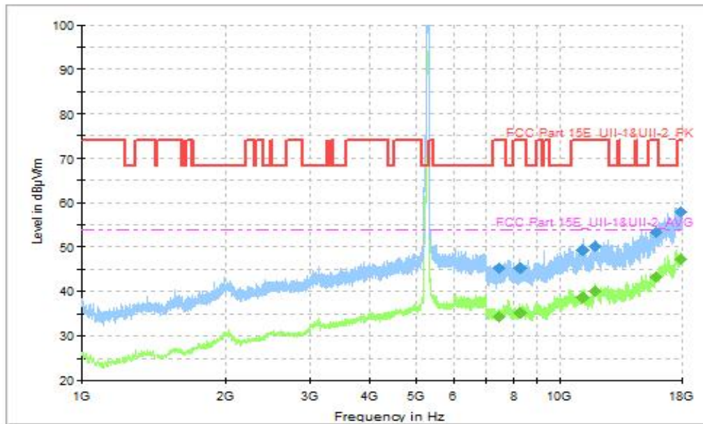
Fig. 68 Transmitter Spurious Emission (802.11be-EHT80, CH58 5290MHz, 1GHz-18GHz), MIMO
