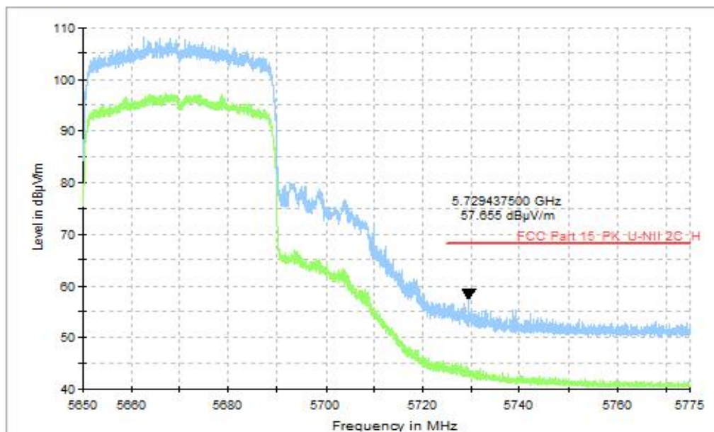
Fig. 36 Band Edges, CH134 5670MHz, MIMO
