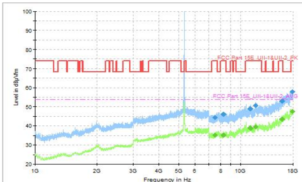
Fig. 51 Transmitter Spurious Emission (802.11be-EHT20, CH64 5320MHz, 1GHz-18GHz), MIMO
