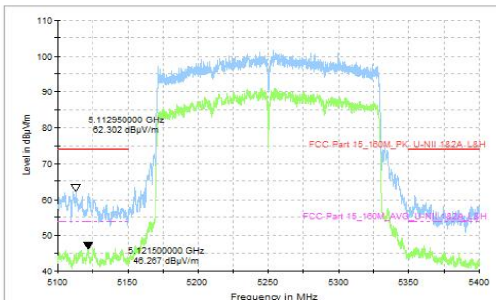
Fig. 44 Band Edges, CH50 5250MHz, MIMO
