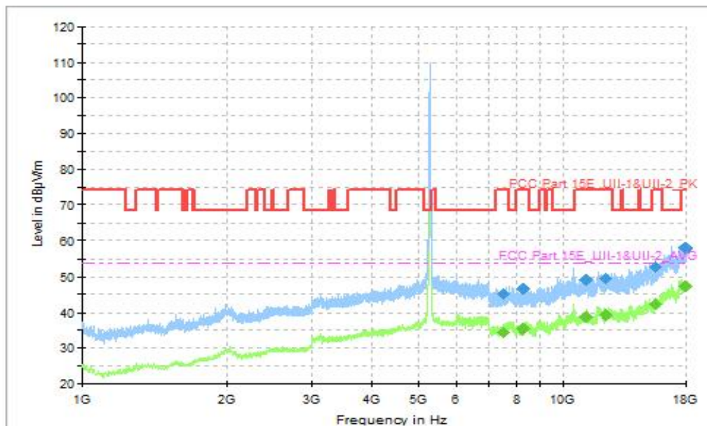
Fig. 50 Transmitter Spurious Emission (802.11be-EHT20, CH56 5280MHz, 1GHz-18GHz), MIMO
