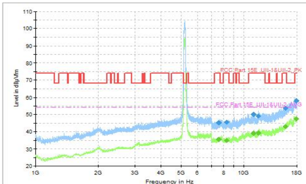
Fig. 67 Transmitter Spurious Emission (802.11be-EHT80, CH42 5210MHz, 1GHz-18GHz), MIMO
