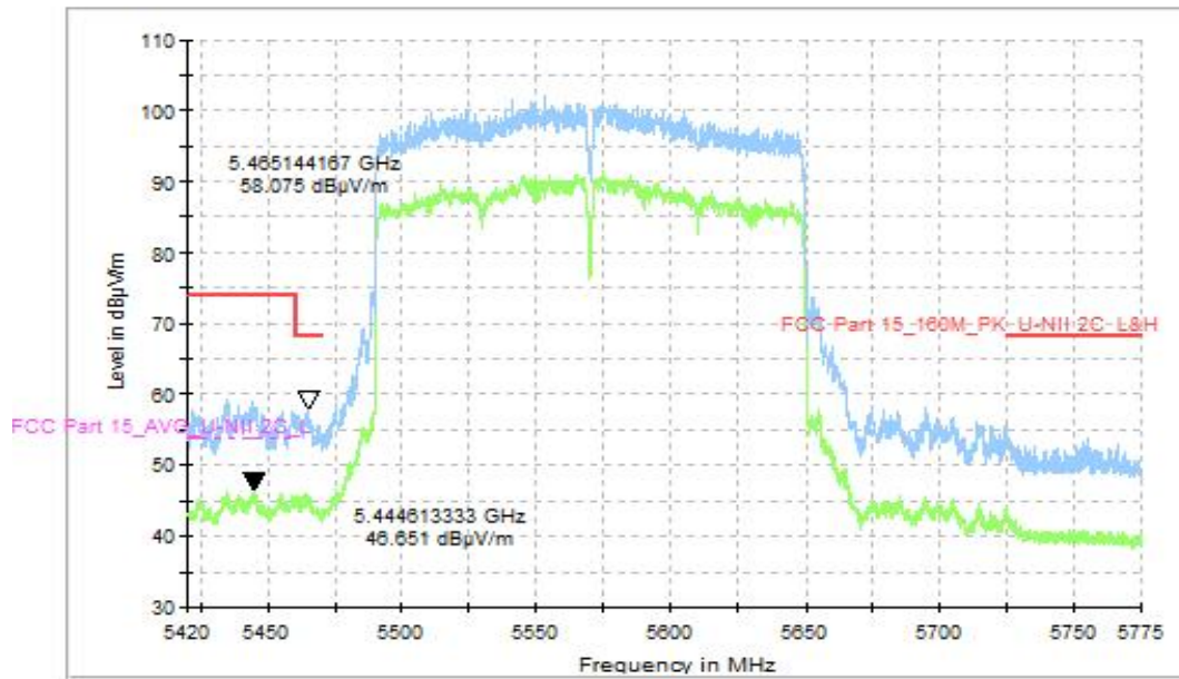
Fig. 45 Band Edges, CH114 5570MHz, MIMO
