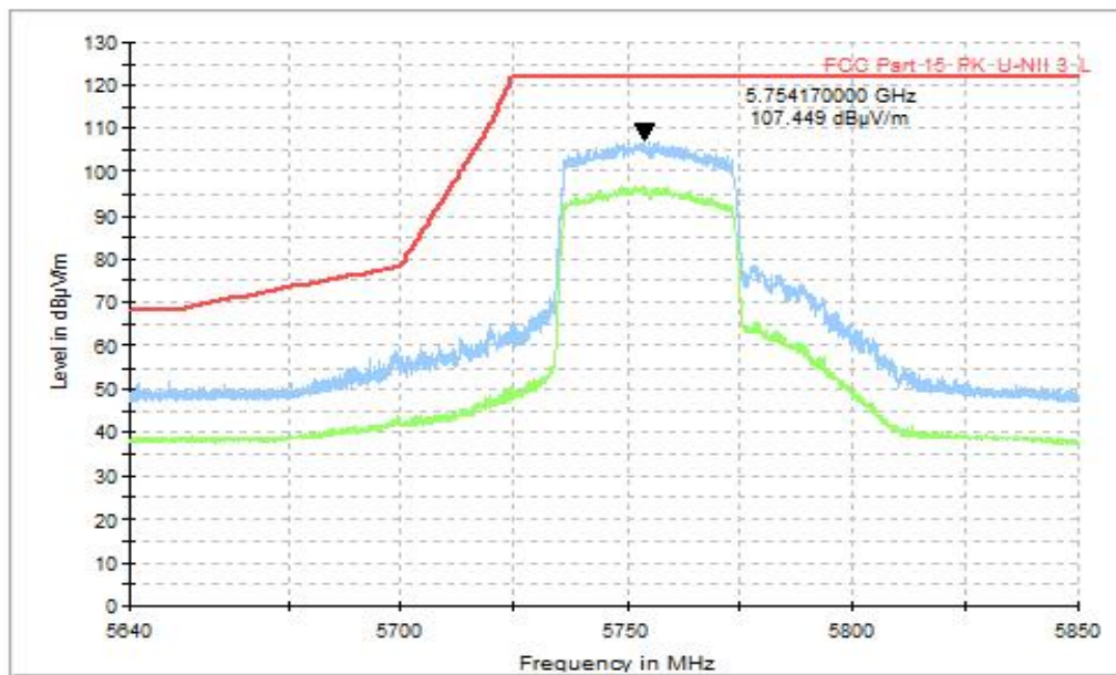
Fig. 37 Band Edges, CH151 5755MHz, MIMO
