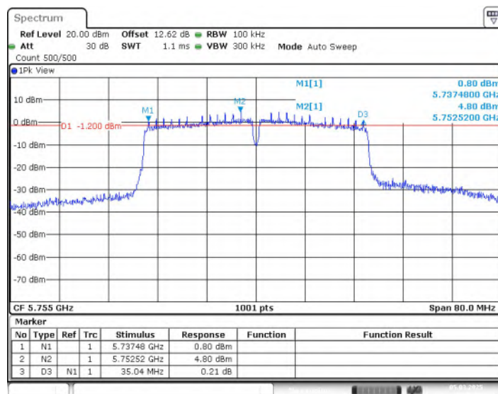
Fig. 12 Occupied 6dB Bandwidth (802.11n-HT40, 5755MHz)
