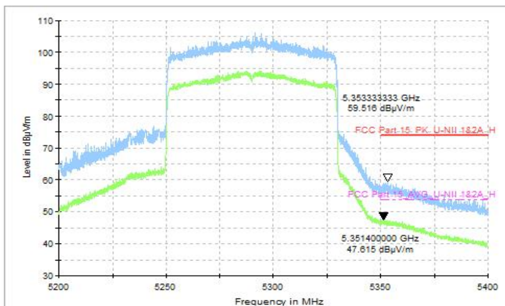
Fig. 40 Band Edges, CH58 5290MHz, MIMO
