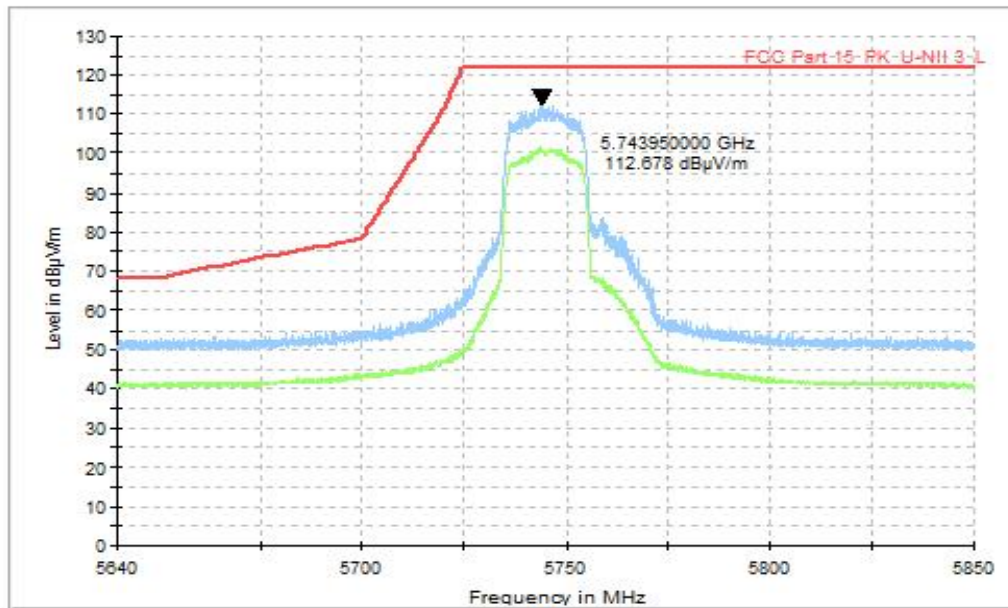
Fig. 31 Band Edges, CH149 5745MHz, MIMO
