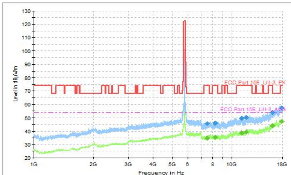
Fig. 71 Transmitter Spurious Emission (802.11be-EHT80, CH155 5775MHz, 1GHz-18GHz), MIMO
