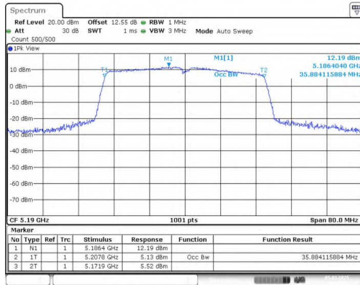
Fig. 17 99% Occupied Bandwidth (802.11n-HT40, 5190MHz)
