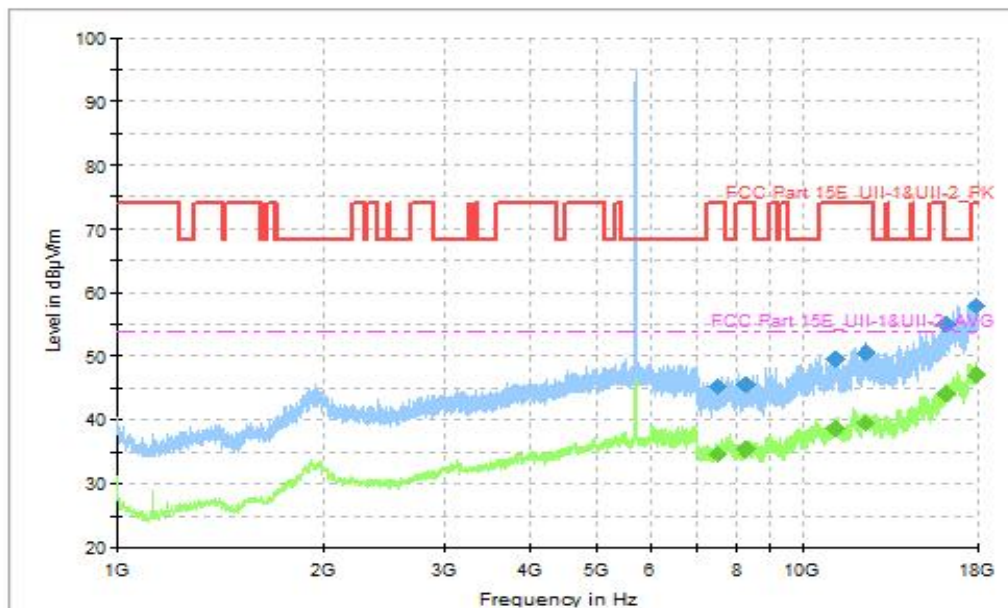
Fig. 54 Transmitter Spurious Emission (802.11be-EHT20, CH140 5700MHz, 1GHz-18GHz), MIMO
