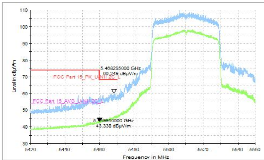
Fig. 35 Band Edges, CH102 5510MHz, MIMO
