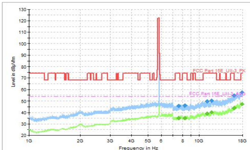
Fig. 57 Transmitter Spurious Emission (802.11be-EHT20, CH165 5825MHz, 1GHz-18GHz), MIMO
