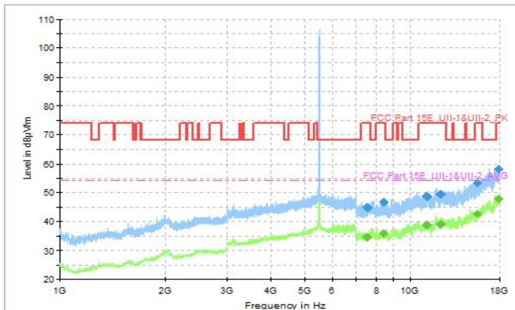
Fig. 52 Transmitter Spurious Emission (802.11be-EHT20, CH100 5500MHz, 1GHz-18GHz), MIMO
