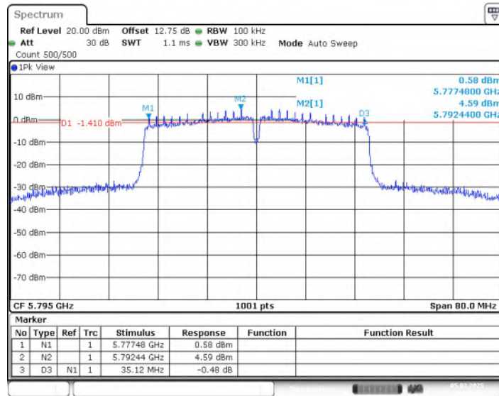
Fig. 13 Occupied 6dB Bandwidth (802.11n-HT40, 5795MHz)
