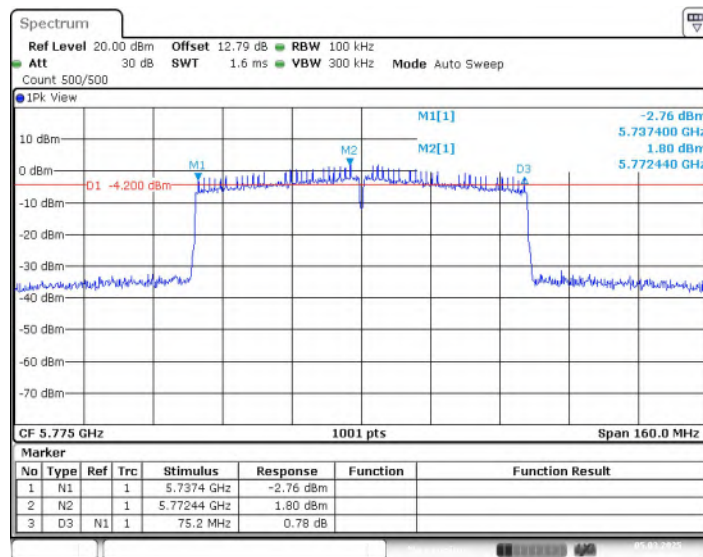
Fig. 14 Occupied 6dB Bandwidth (802.11ac-VHT80, 5775MHz)
