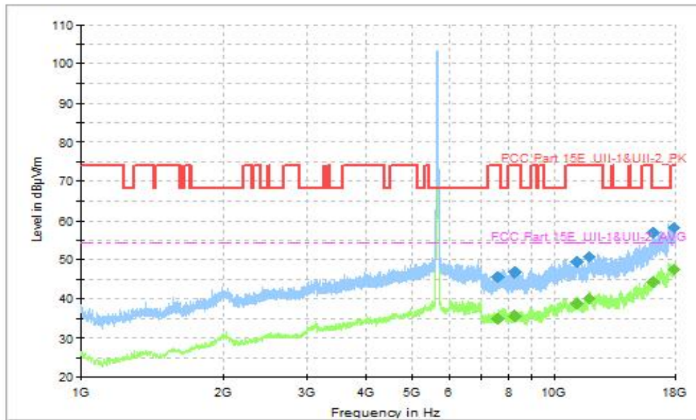
Fig. 64 Transmitter Spurious Emission (802.11be-EHT40, CH134 5670MHz, 1GHz-18GHz), MIMO
