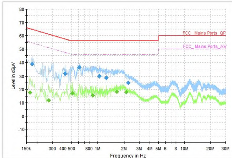
Fig. 78 AC Power line Conducted Emission (Traffic)
