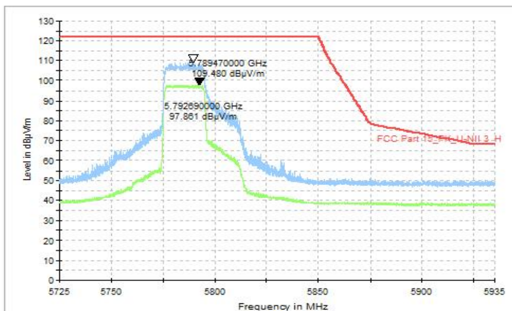
Fig. 38 Band Edges, CH159 5795MHz, MIMO
