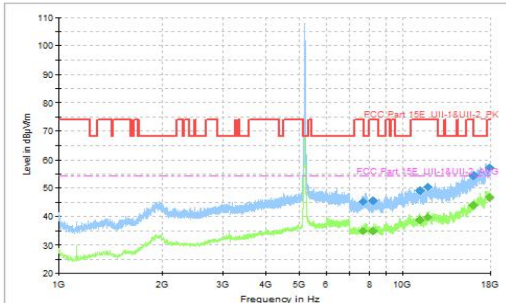
Fig. 47 Transmitter Spurious Emission (802.11be-EHT20, CH40 5200MHz, 1GHz-18GHz), MIMO
