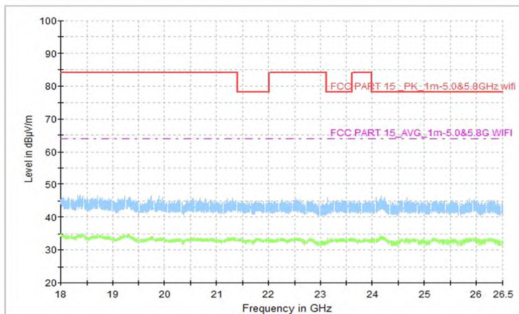
Fig. 75 Transmitter Spurious Emission (All channel, 18GHz~26.5GHz), MIMO
