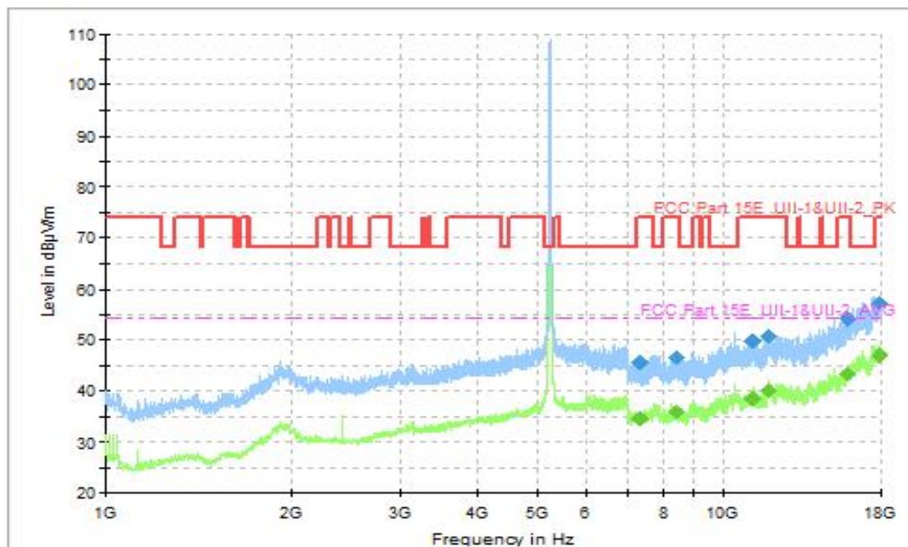
Fig. 48 Transmitter Spurious Emission (802.11be-EHT20, CH48 5240MHz, 1GHz-18GHz), MIMO
