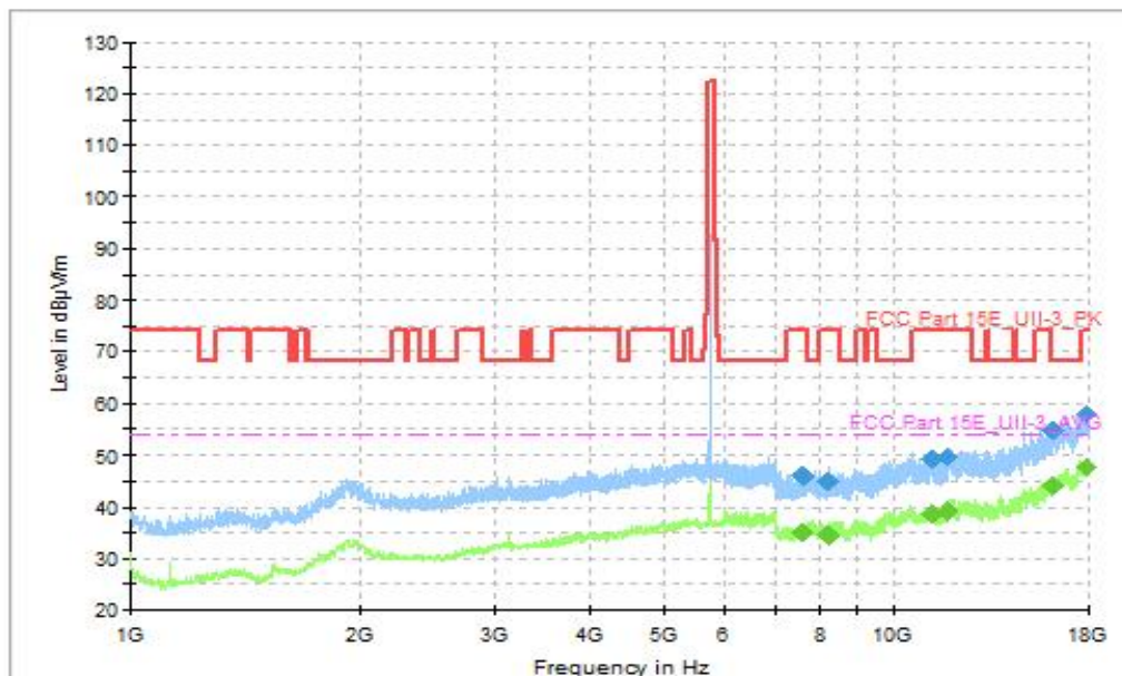
Fig. 55 Transmitter Spurious Emission (802.11be-EHT20, CH149 5745MHz, 1GHz-18GHz), MIMO
