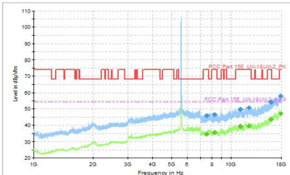
Fig. 53 Transmitter Spurious Emission (802.11be-EHT20, CH120 5600MHz, 1GHz-18GHz), MIMO
