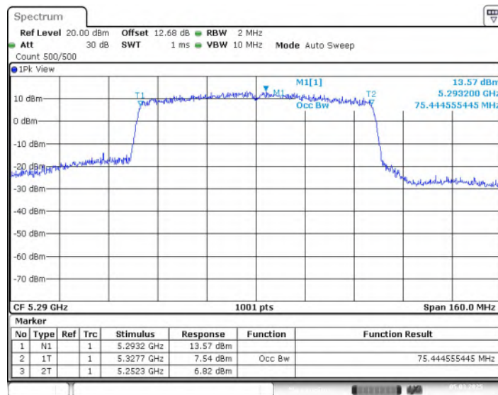
Fig. 20 99% Occupied Bandwidth (802.11ac-VHT80, 5290MHz)
