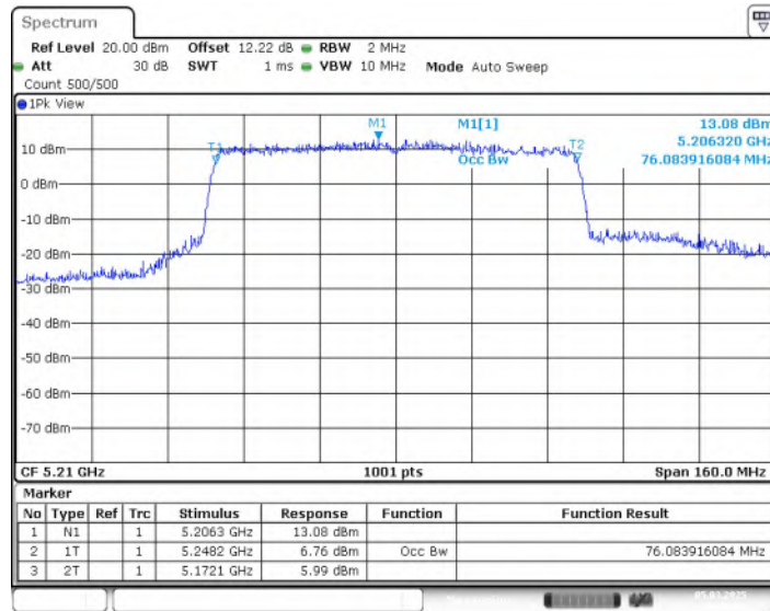
Fig. 19 99% Occupied Bandwidth (802.11ac-VHT80, 5210MHz)
