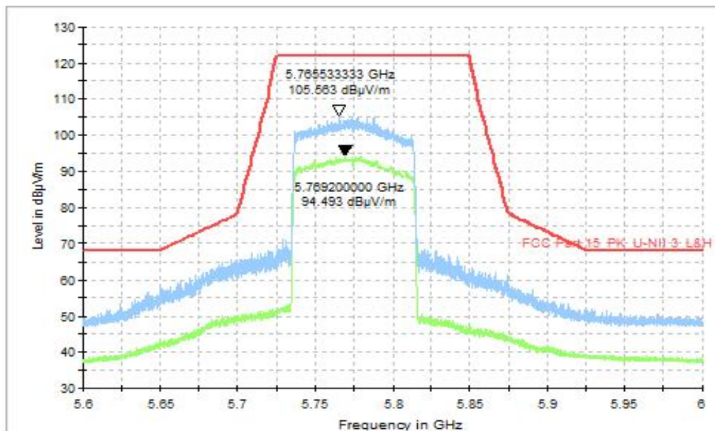
Fig. 43 Band Edges, CH155 5775MHz, MIMO
