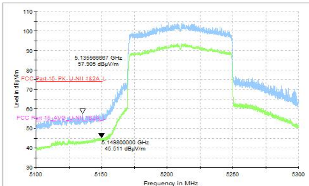
Fig. 39 Band Edges, CH42 5210MHz, MIMO
