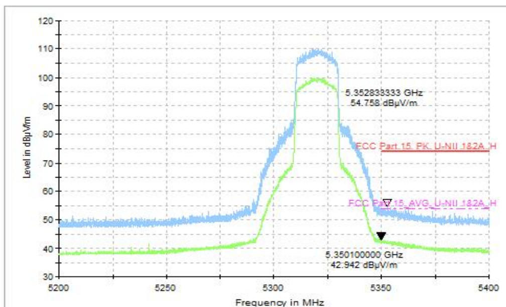
Fig. 28 Band Edges CH64 5320MHz, MIMO
