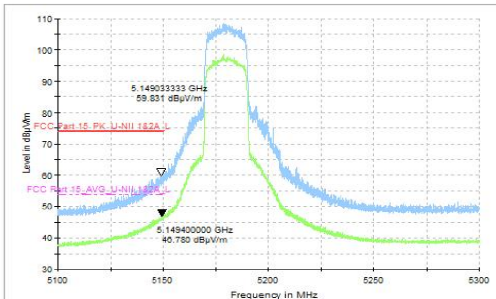
Fig. 27 Band Edges, CH36 5180MHz, MIMO
