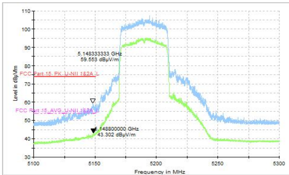
Fig. 33 Band Edges, CH38 5190MHz, MIMO
