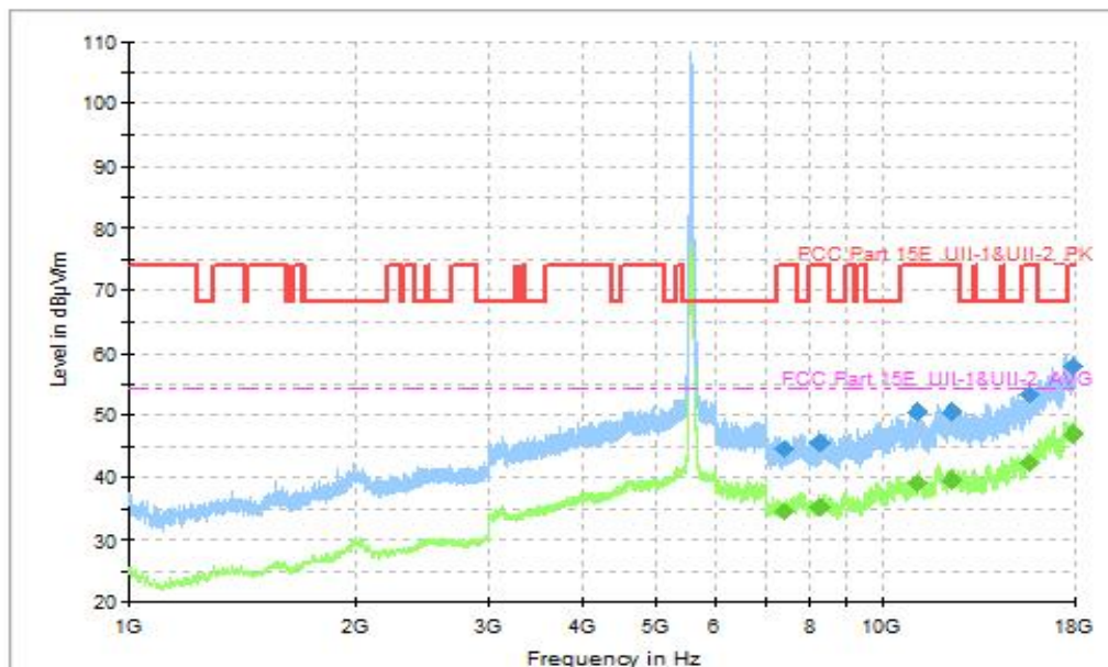
Fig. 63 Transmitter Spurious Emission (802.11be-EHT40, CH118 5580MHz, 1GHz-18GHz), MIMO
