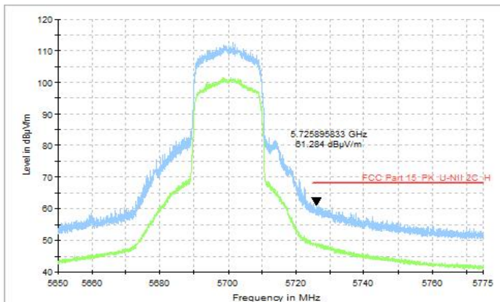
Fig. 30 Band Edges, CH140 5700MHz, MIMO
