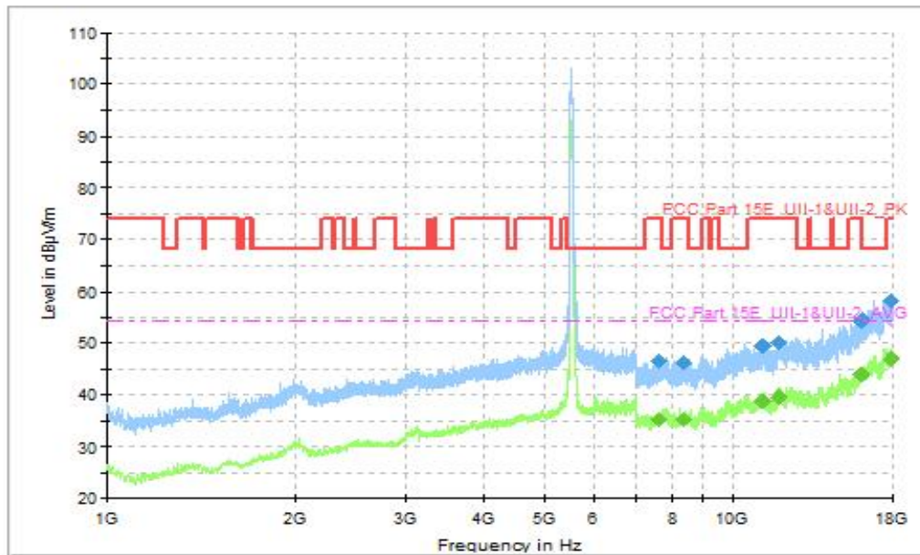
Fig. 69 Transmitter Spurious Emission (802.11be-EHT80, CH106 5530MHz, 1GHz-18GHz), MIMO
