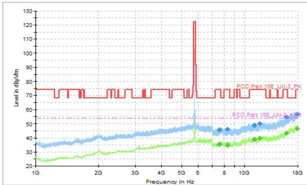
Fig. 65 Transmitter Spurious Emission (802.11be-EHT40, CH151 5755MHz, 1GHz-18GHz), MIMO
