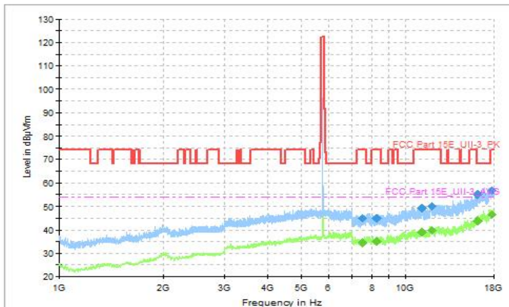
Fig. 56 Transmitter Spurious Emission (802.11be-EHT20, CH157 5785MHz, 1GHz-18GHz), MIMO
