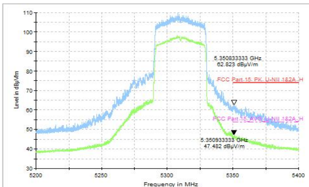
Fig. 34 Band Edges, CH62 5310MHz, MIMO
