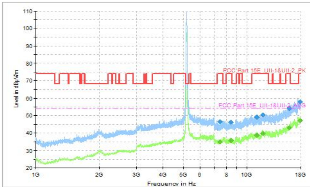
Fig. 58 Transmitter Spurious Emission (802.11be-EHT40, CH38 5190MHz, 1GHz-18GHz), MIMO
