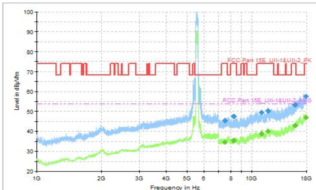
Fig. 73 Transmitter Spurious Emission (802.11be-EHT160, CH114 5570MHz, 1GHz-18GHz), MIMO
