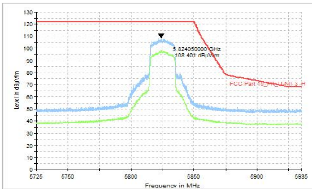
Fig. 32 Band Edges, CH165 5825MHz, MIMO
