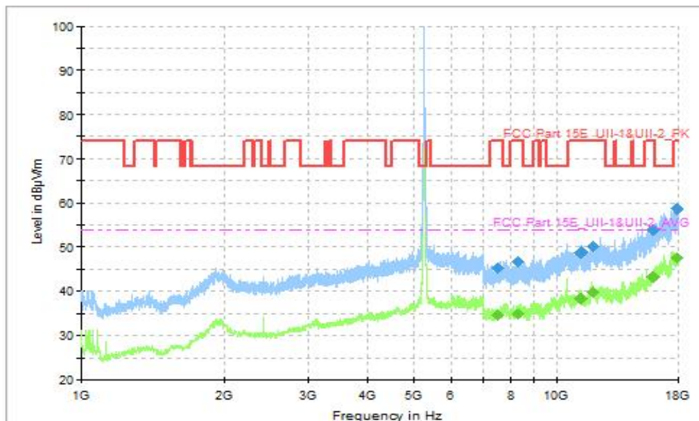
Fig. 49 Transmitter Spurious Emission (802.11be-EHT20, CH52 5260MHz, 1GHz-18GHz), MIMO
