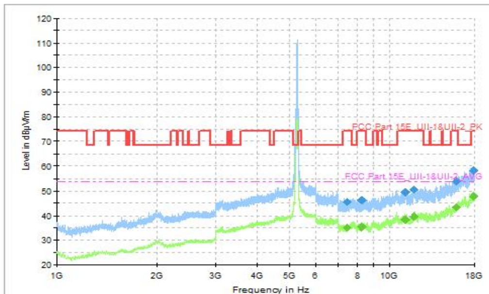
Fig. 60 Transmitter Spurious Emission (802.11be-EHT40, CH54 5270MHz, 1GHz-18GHz), MIMO
