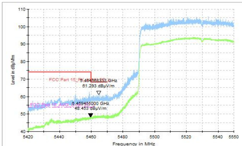
Fig. 41 Band Edges, CH106 5530MHz, MIMO
