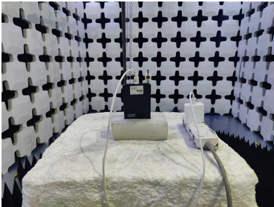
18. Radiated Emissions (Par22/24/27, 26.5GHz-40GHz)
