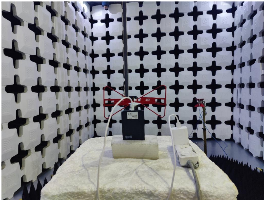
16. Radiated Emissions (Part 22/24/27, 30MHz-18GHz)
