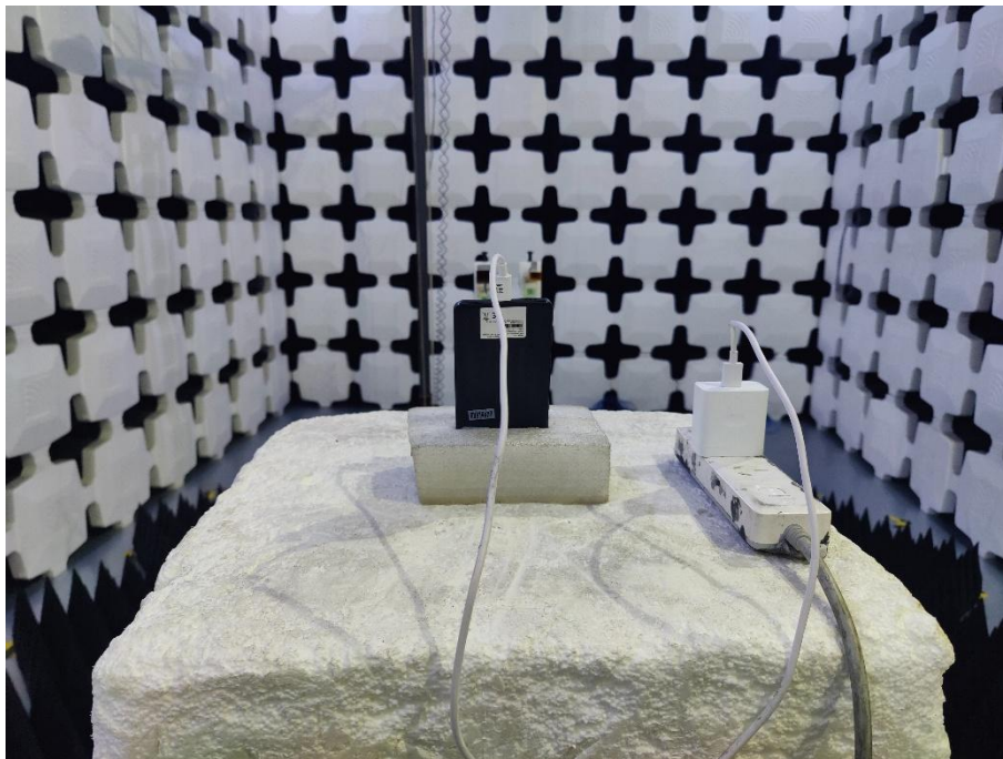
14. Radiated Emissions (Part 15C&Part 15E, 18GHz -26.5GHz)
