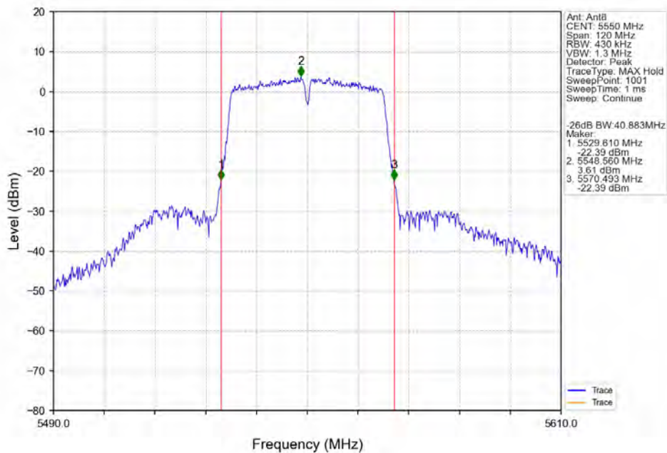
802.11n(HT40)_MCH_5550MHz_Ant8_NTNV
