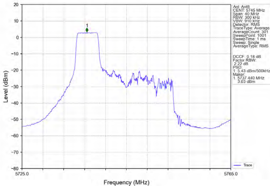
802.11ax(HEW20)_LCH_5745MHz_RU106_Left_Ant8_NTNV
