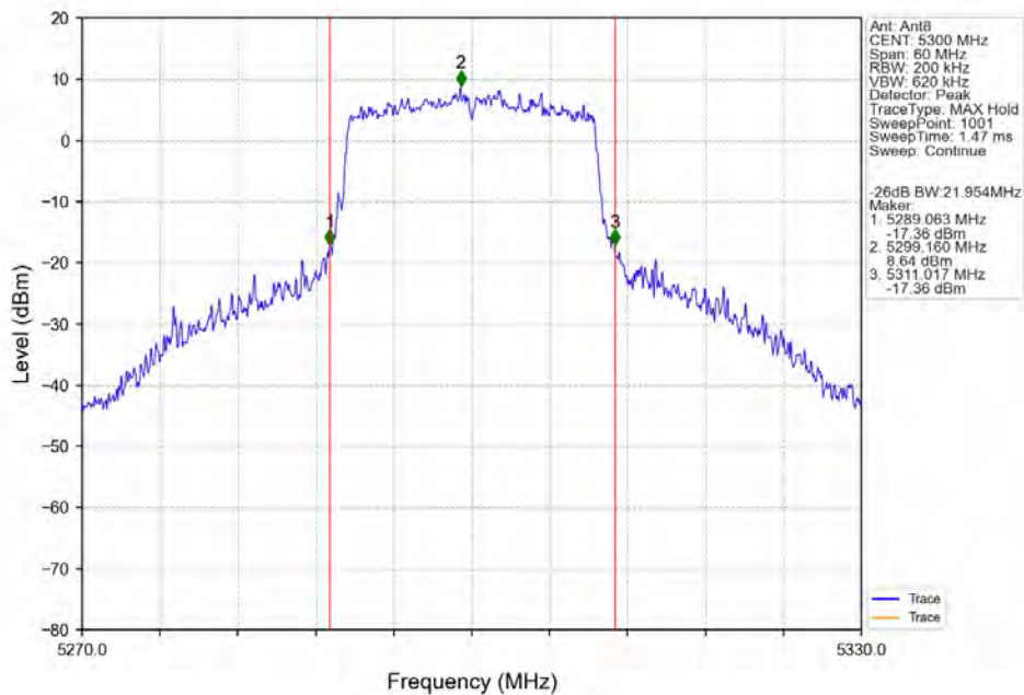
802.11ax(HEW20)_MCH_5300MHz_RU242_Left_Ant8_NTNV
