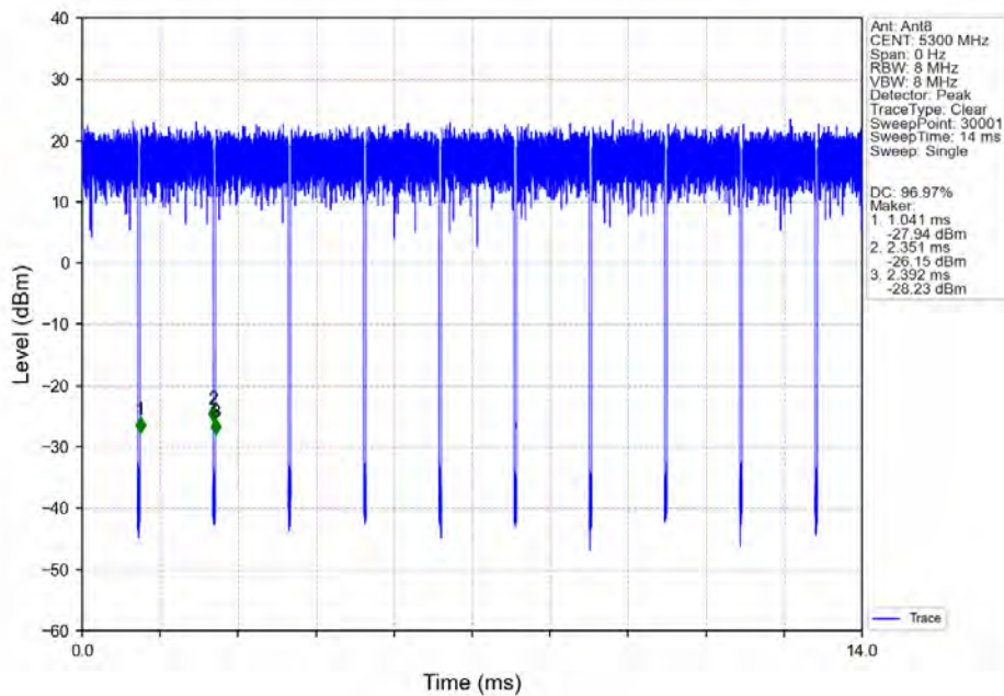
802.11ac(VHT20)_MCH_5300MHz_Ant8_NTNV
