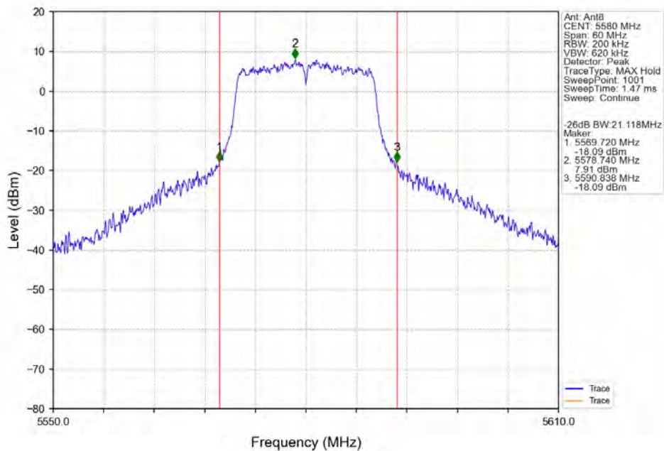
802.11a_MCH_5580MHz_Ant8_NTNV
