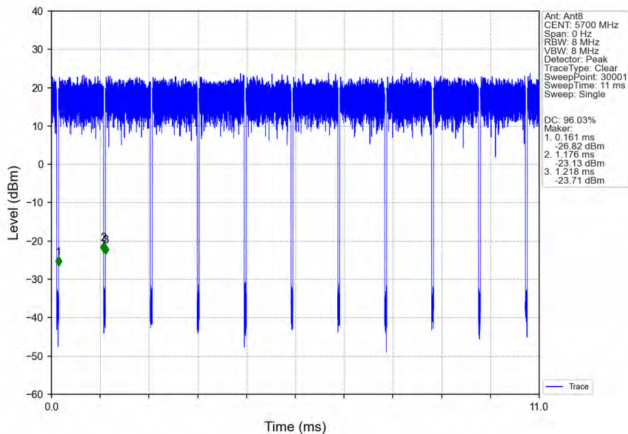
802.11ax(HEW20)_HCH_5700MHz_RU242_Left_Ant8_NTNV
