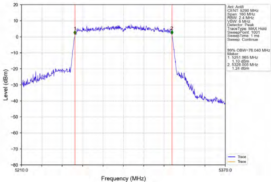
802.11ac(VHT80)_MCH_5290MHz_Ant8_NTNV
