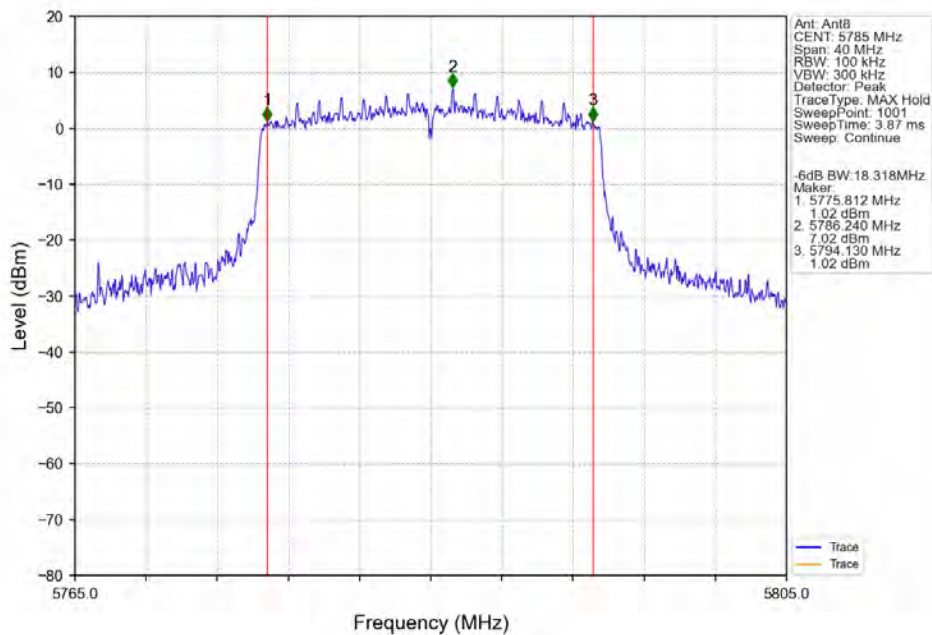
802.11ax(HEW20)_MCH_5785MHz_RU242_Left_Ant8_NTNV
