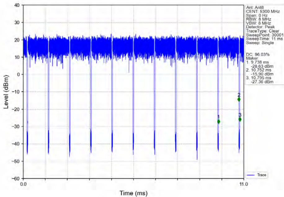
802.11ax(HEW20)_MCH_5300MHz_RU242_Left_Ant8_NTNV
