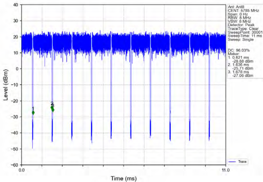
802.11ax(HEW20)_MCH_5785MHz_RU242_Left_Ant8_NTNV
