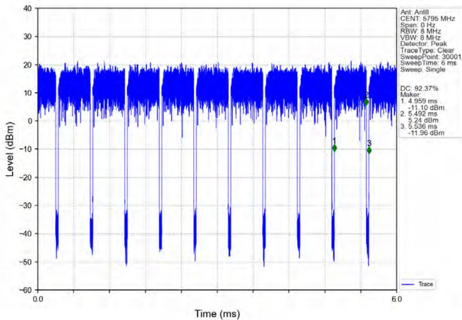
802.11ax(HEW40)_HCH_5795MHz_RU484_Left_Ant8_NTNV
