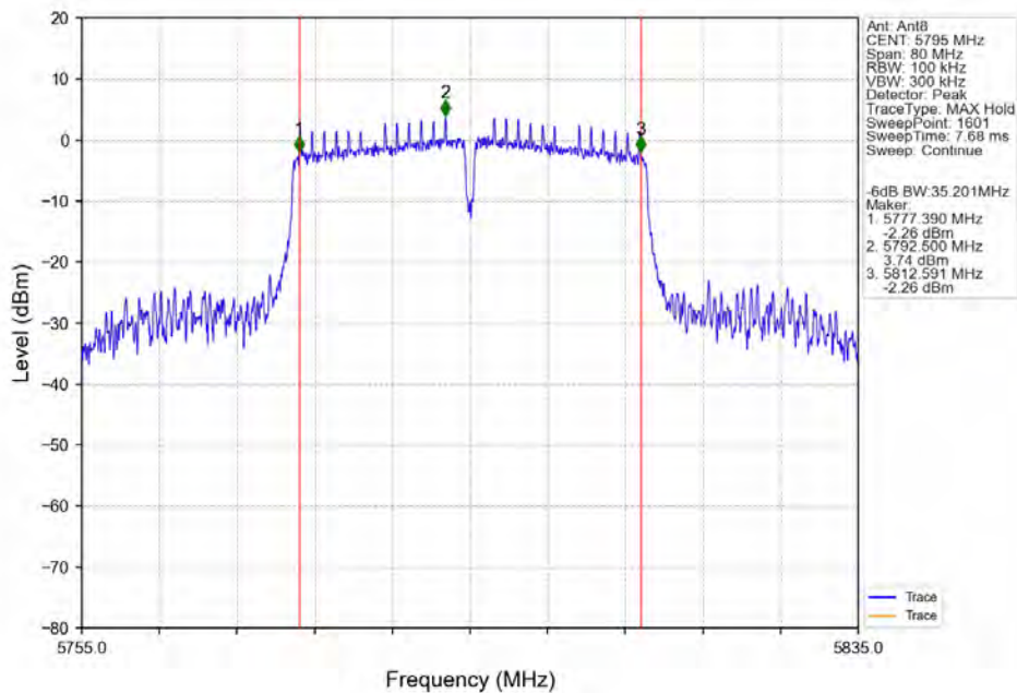
802.11n(HT40)_HCH_5795MHz_Ant8_NTNV
