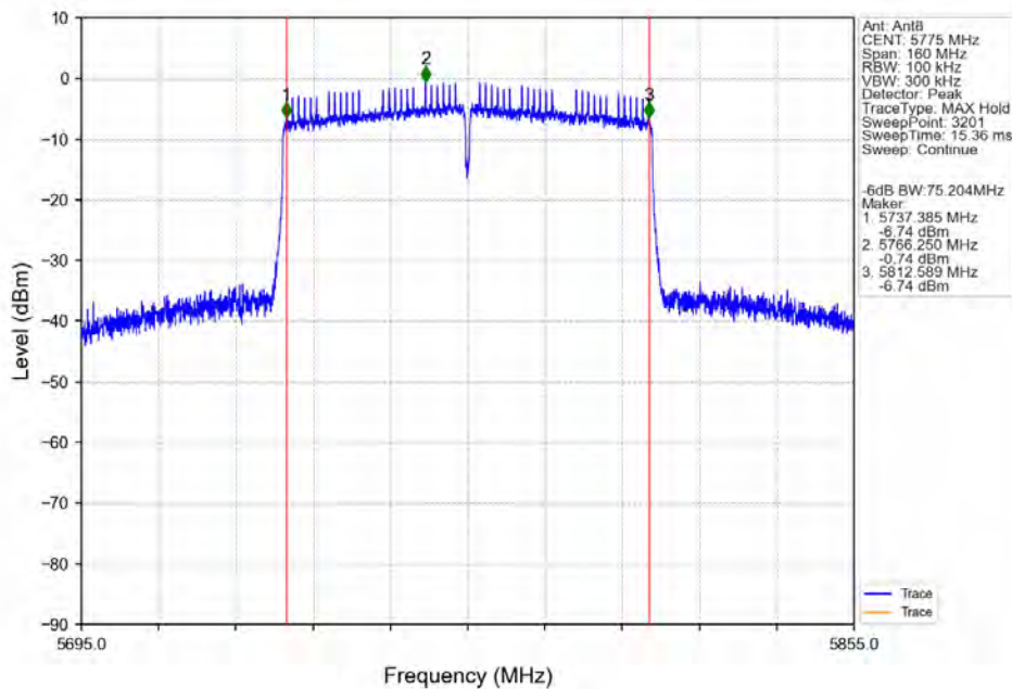
802.11ac(VHT80)_MCH_5775MHz_Ant8_NTNV
