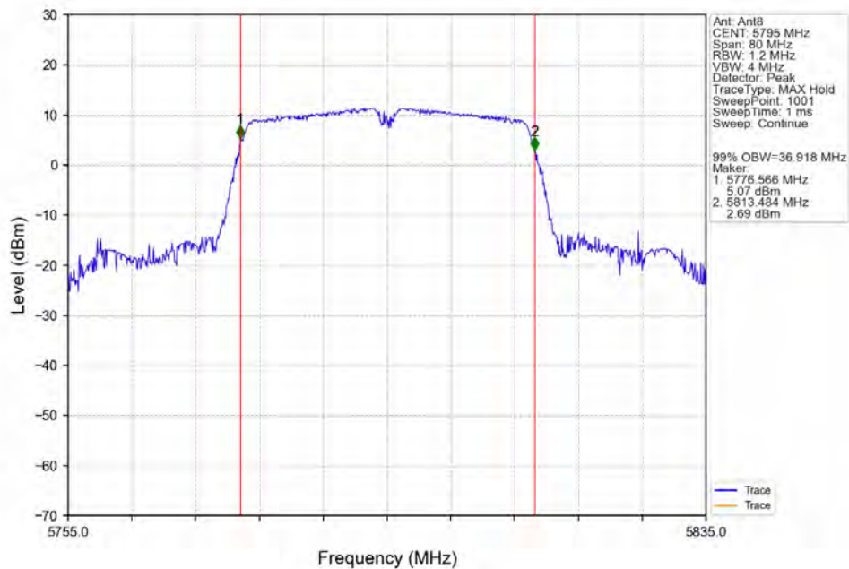
802.11ac(VHT40)_HCH_5795MHz_Ant8_NTNV
