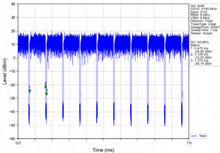
802.11ac(VHT40)_LCH_5190MHz_Ant8_NTNV
