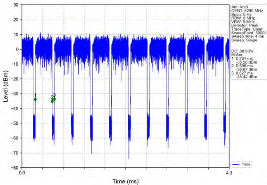
802.11ac(VHT80)_MCH_5290MHz_Ant8_NTNV
