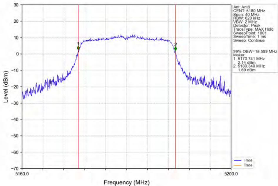
802.11ac(VHT20)_LCH_5180MHz_Ant8_NTNV
