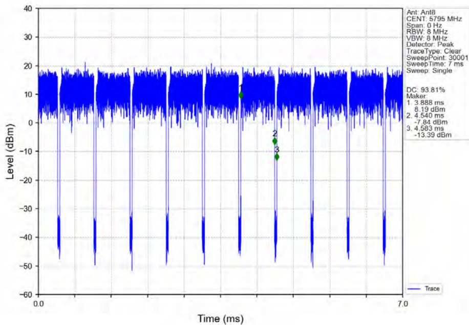
802.11ac(VHT40)_HCH_5795MHz_Ant8_NTNV
