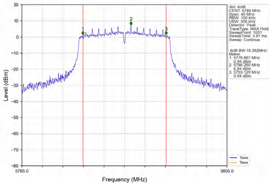
802.11ac(VHT20)_MCH_5785MHz_Ant8_NTNV
