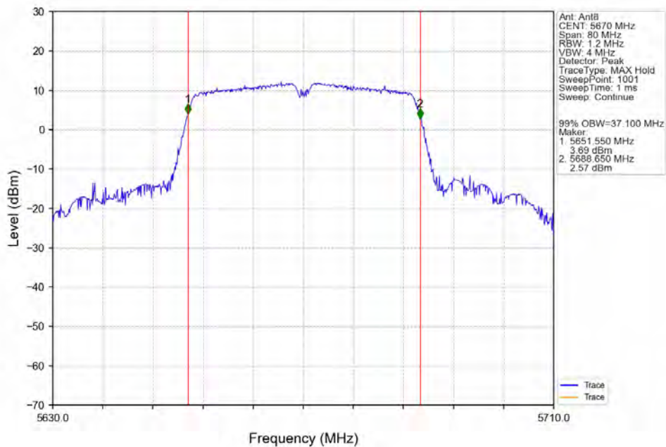
802.11ac(VHT40)_HCH_5670MHz_Ant8_NTNV
