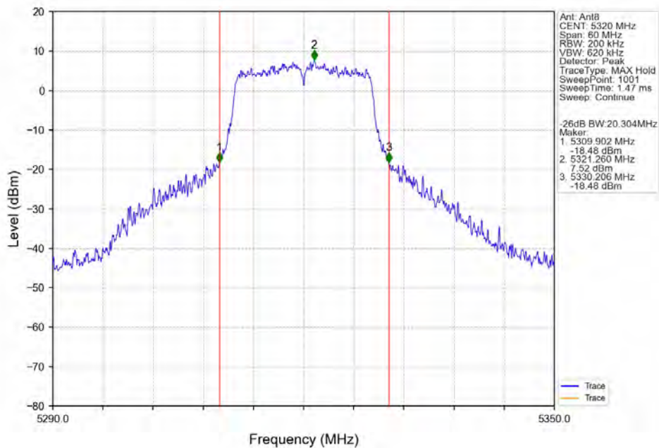
802.11a_HCH_5320MHz_Ant8_NTNV
