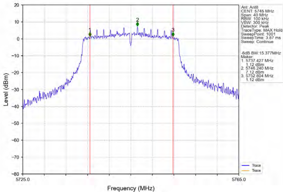
802.11n(HT20)_LCH_5745MHz_Ant8_NTNV
