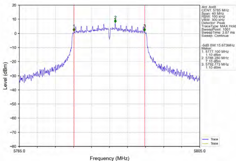
802.11a_MCH_5785MHz_Ant8_NTNV
