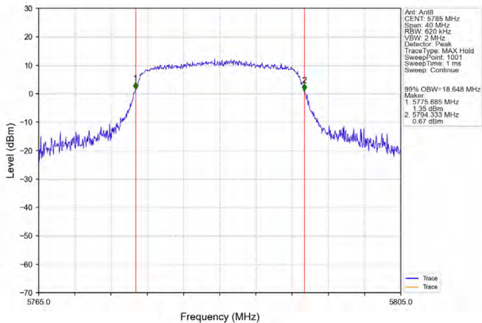
802.11ac(VHT20)_MCH_5785MHz_Ant8_NTNV
