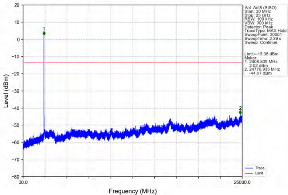
802.11ax(HEW20)_LCH_2412MHz_RU106_Left_Ant8 (SISO)_NTNV
