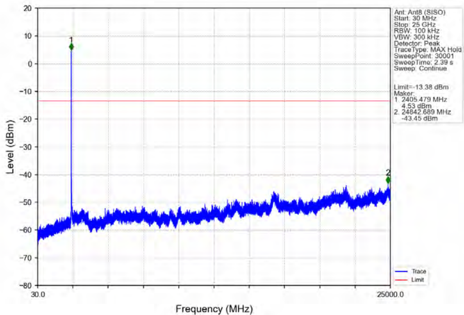
802.11ax(HEW20)_LCH_2412MHz_RU52_Left_Ant8 (SISO)_NTNV
