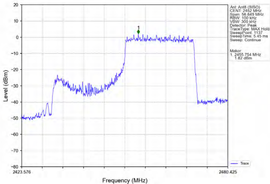
802.11ax(HEW40)_HCH_2452MHz_RU242_Right_Ant8 (SISO)_NTNV
