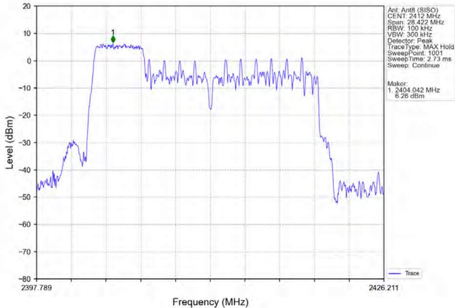
802.11ax(HEW20)_LCH_2412MHz_RU106_Left_Ant8 (SISO)_NTNV
