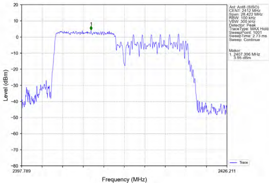
802.11ax(HEW20)_LCH_2412MHz_RU106_Left_Ant8 (SISO)_NTNV
