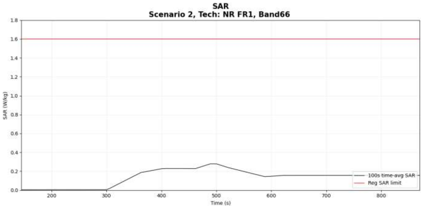
Figure 5- 11 Time-averaged SAR for case 7 (sub6 NR n66)
