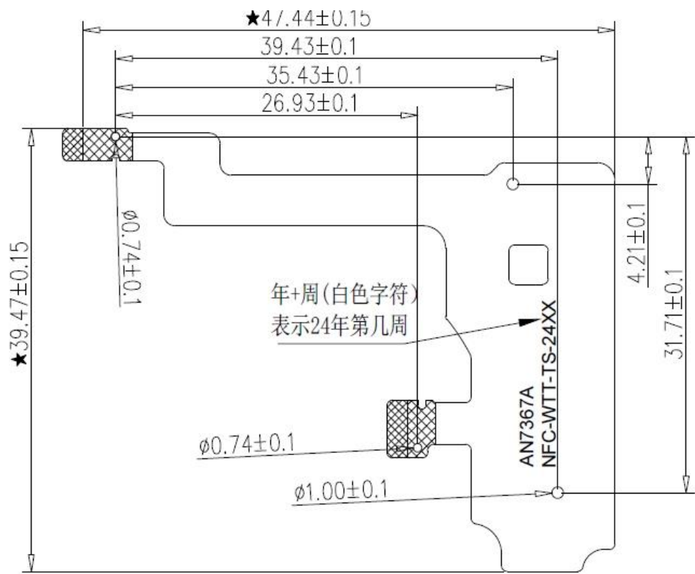
Fig 2 NFC antenna information
