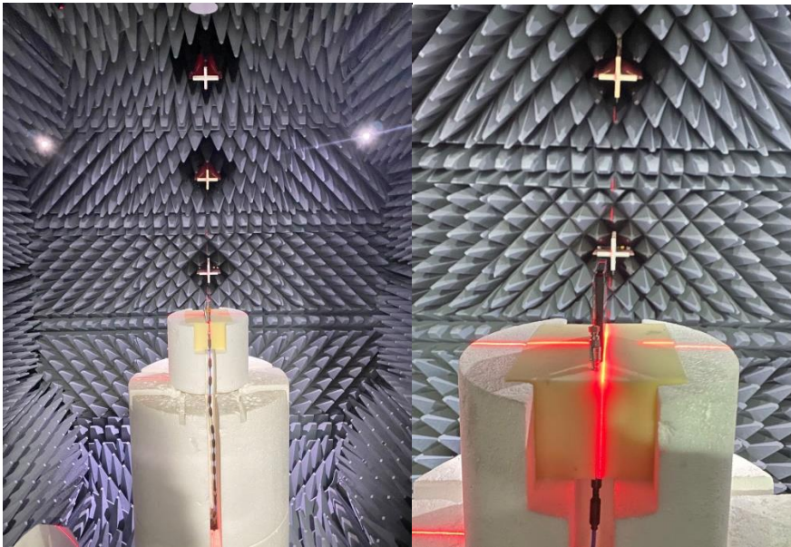
Fig.6. The DUT in the fully anechoic chamber
