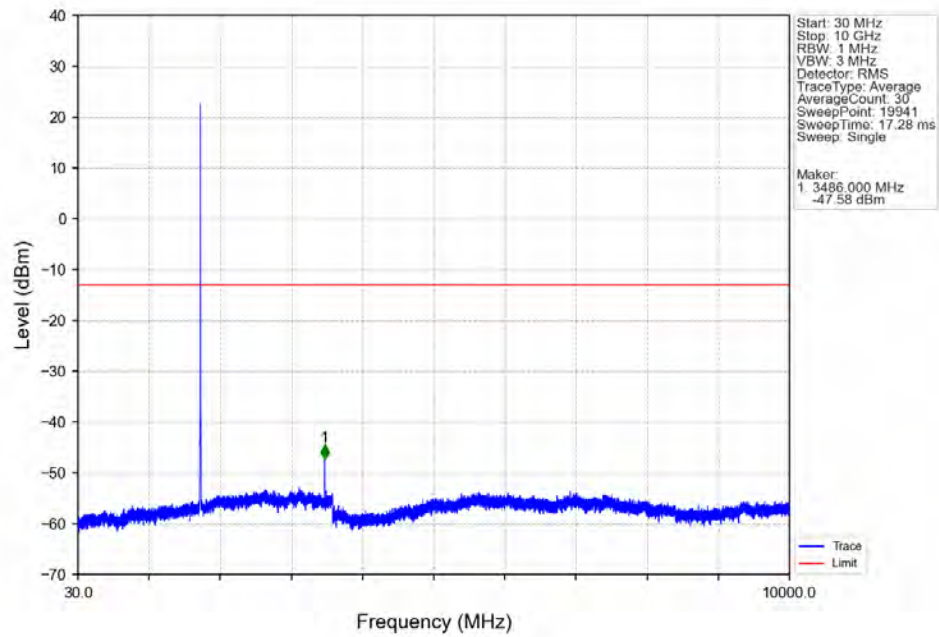
Band66_5MHz_16QAM_MCH_1745MHz_RB_1_0_NTV
