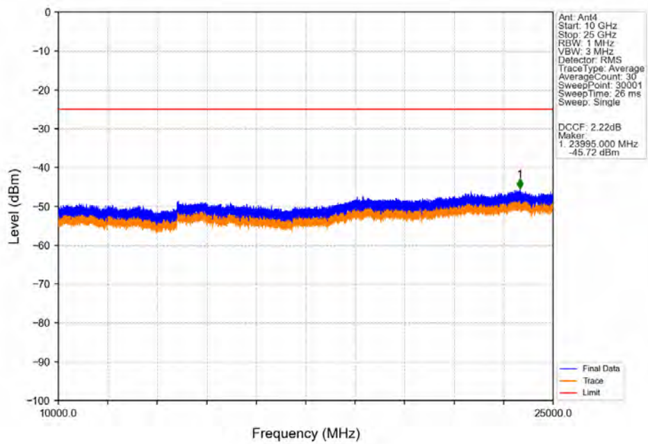
Band41_10MHz_64QAM_LCH_2501MHz_RB_1_0_NTNV
