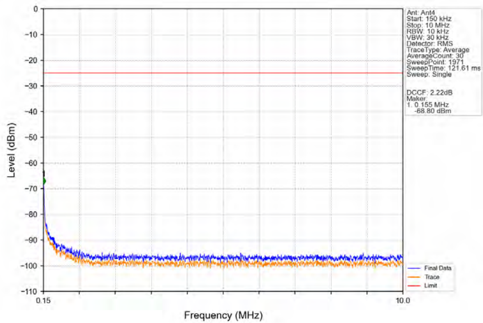
Band41_10MHz_64QAM_HCH_2685MHz_RB_1_0_NTNV
