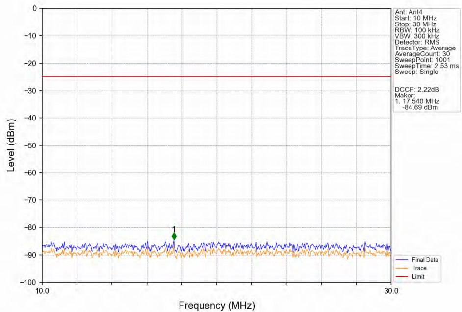
Band41_10MHz_64QAM_LCH_2501MHz_RB_1_0_NTNV
