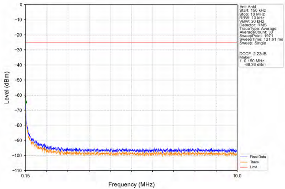
Band41_20MHz_16QAM_LCH_2506MHz_RB_1_0_NTNV
