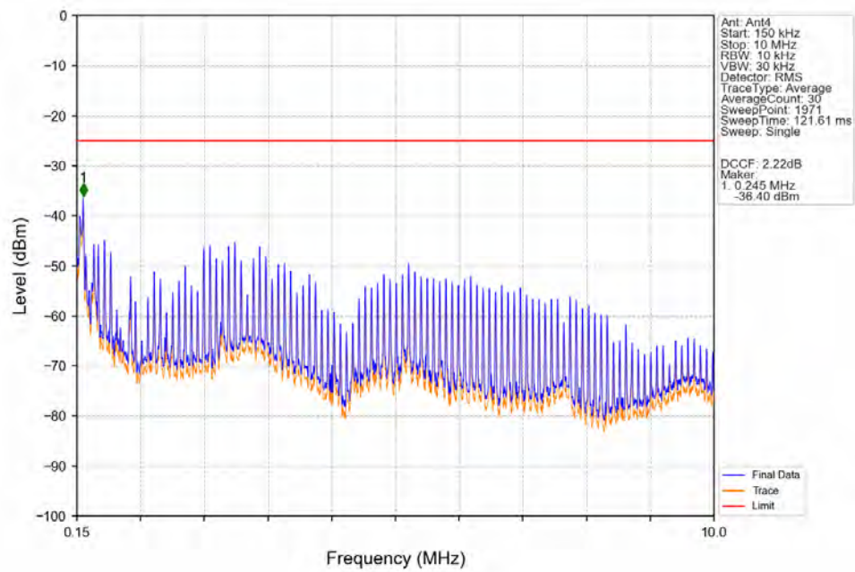
Band41_20MHz_64QAM_MCH_2593MHz_RB_1_0_NTNV
