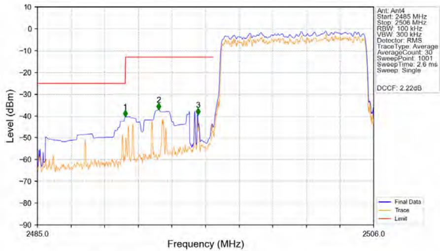
Band41_10MHz_64QAM_LCH_2501MHz_RB_50_0_NTNV
