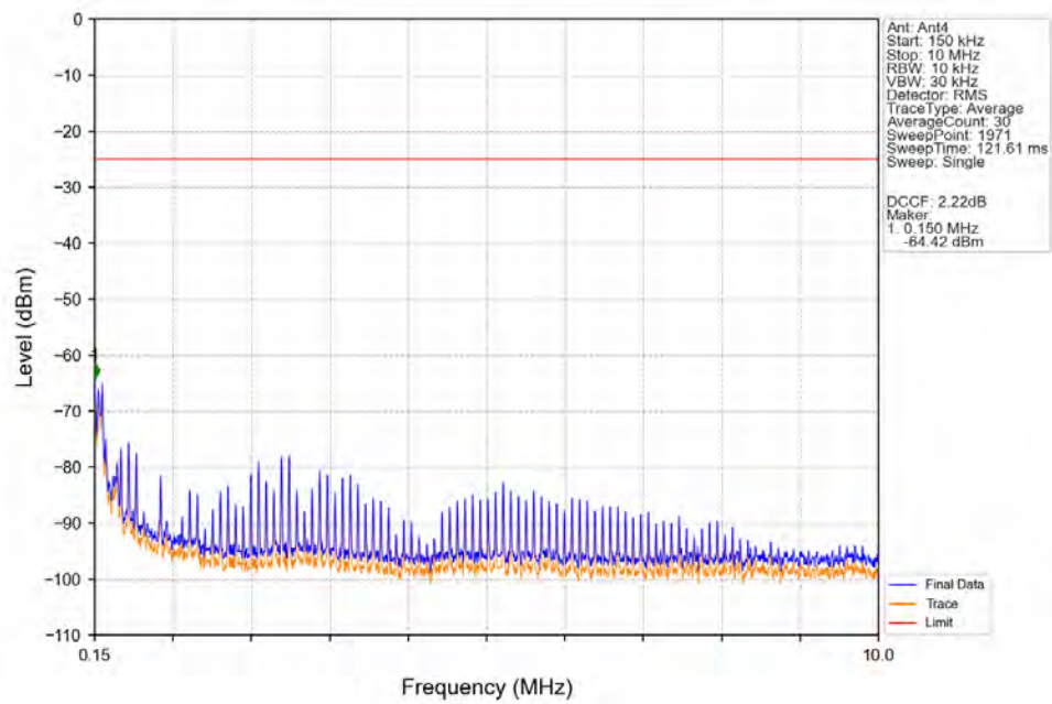
Band41_20MHz_64QAM_HCH_2680MHz_RB_1_0_NTNV
