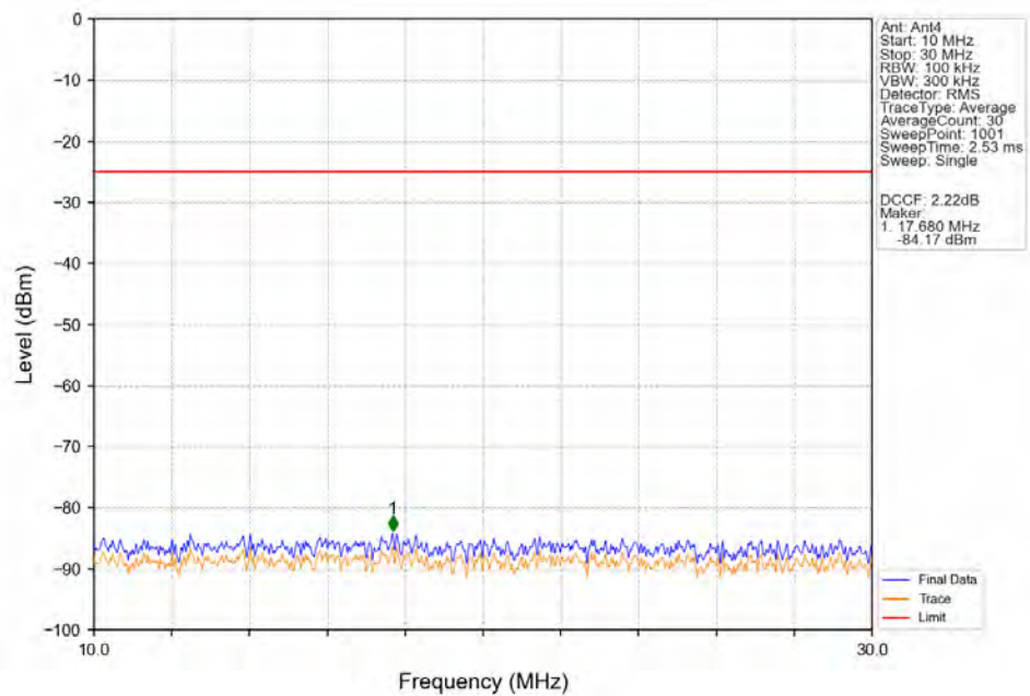
Band41_20MHz_64QAM_LCH_2506MHz_RB_1_0_NTNV
