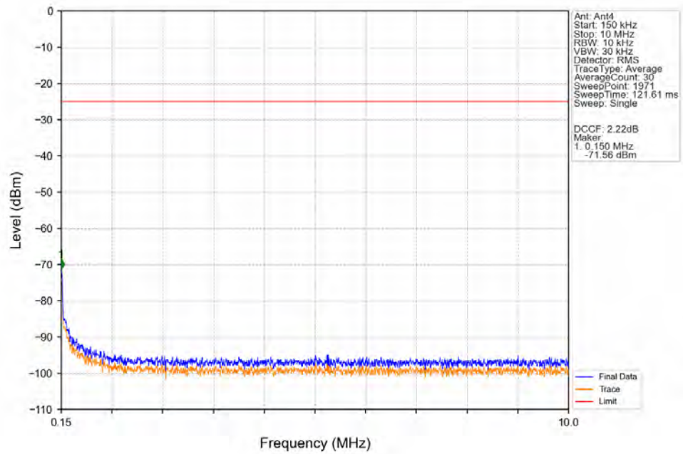
Band41_10MHz_64QAM_LCH_2501MHz_RB_1_0_NTNV
