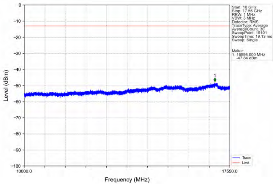
Band4 10MHz 64QAM HCH 1750MHz RB 1 0 NTV
