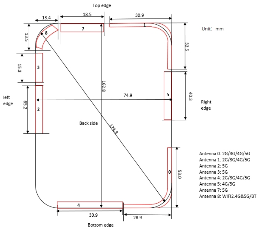
Photograph 11. Antenna position of EUT
