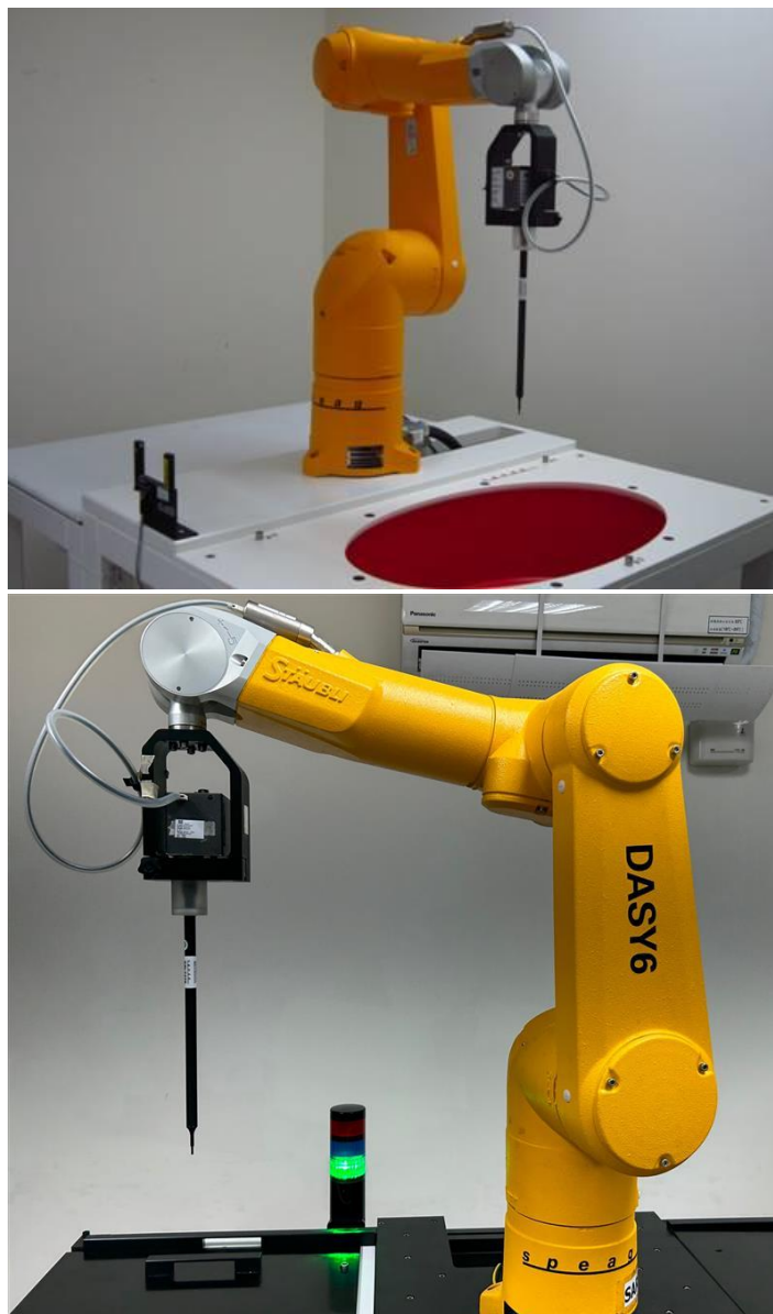
Fig.1 Photograph of the SAR measurement system
