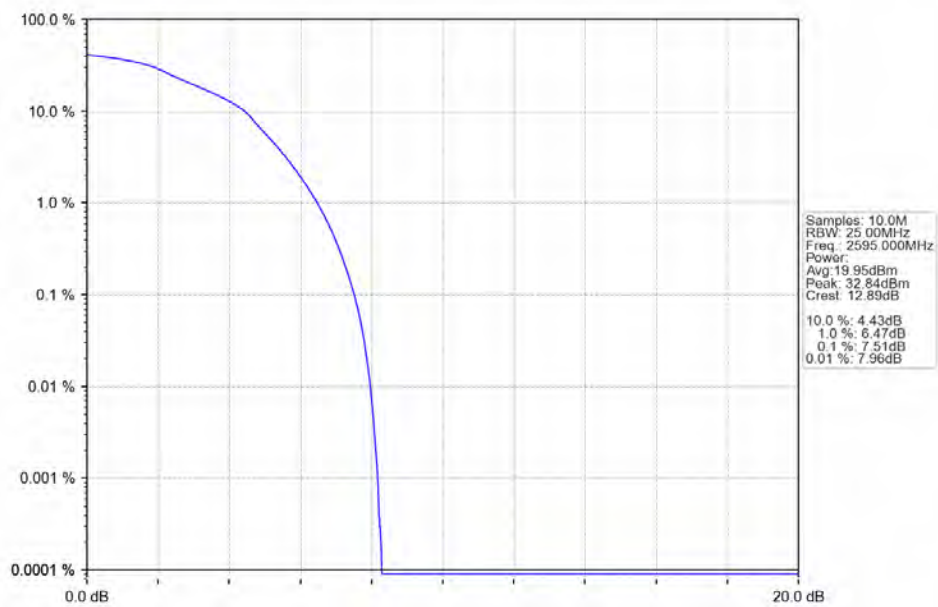
Band38_20MHz_64QAM_MCH_2595MHz_RB_100_0_NTN
