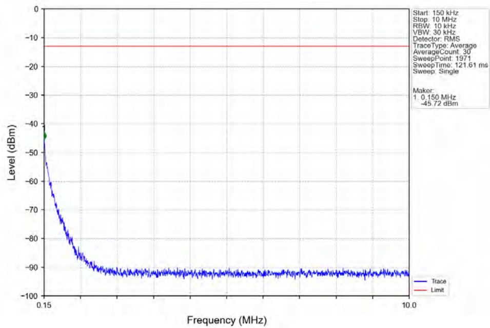
Band26a 5MHz 64QAM MCH 819MHz RB 1 0 NTNV
