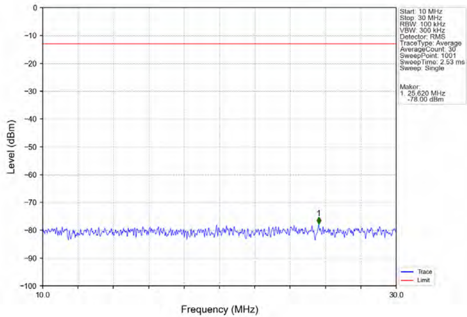
Band12_5MHz_64QAM_HCH_713.5MHz_RB_1_0_NTNV
