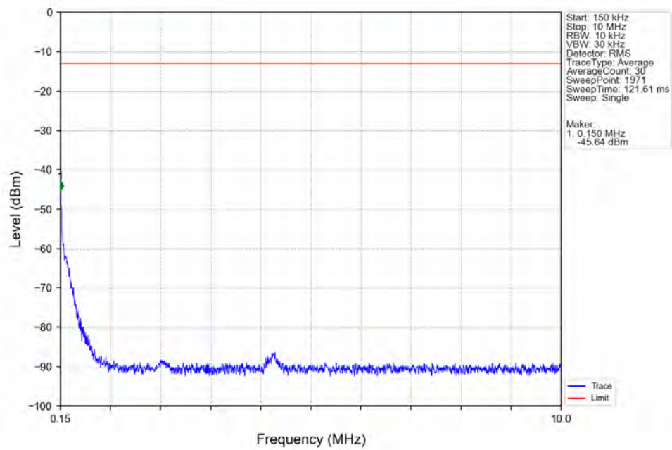
Band12_5MHz_64QAM_MCH_707.5MHz_RB_1_0_NTNV
