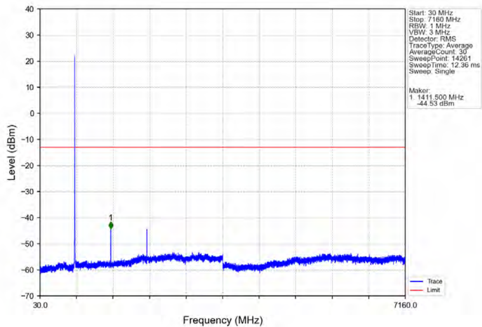
Band12_5MHz_64QAM_MCH_707.5MHz_RB_1_0_NTNV
