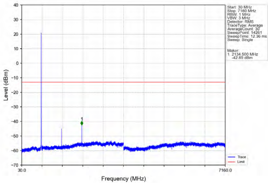
Band12_5MHz_64QAM_HCH_713.5MHz_RB_1_0_NTNV
