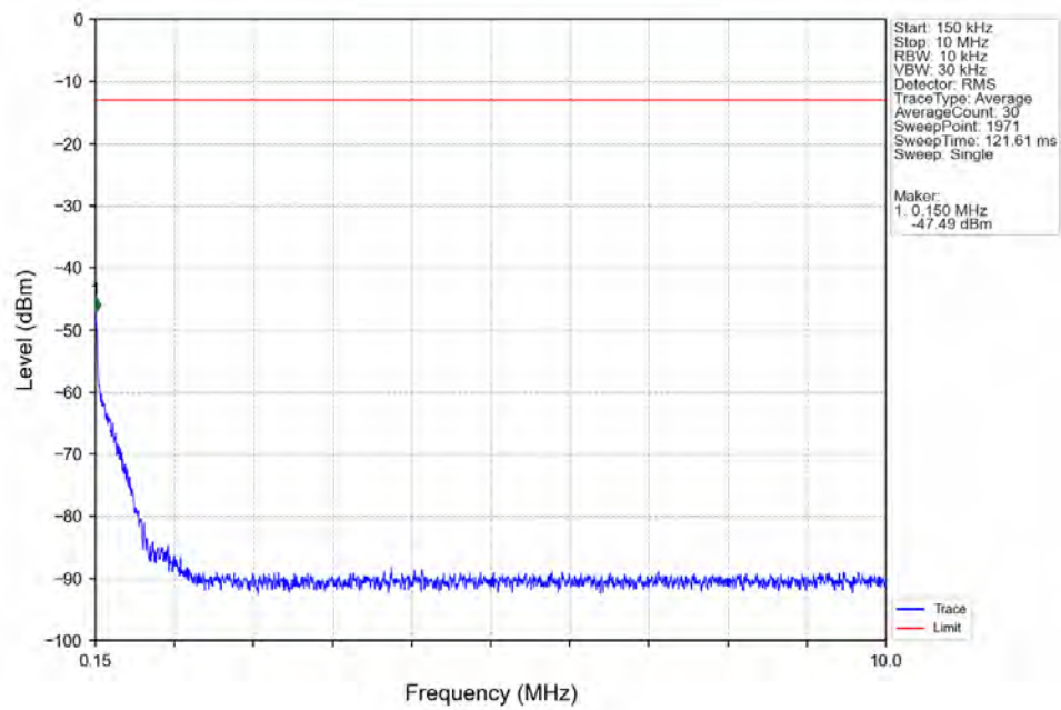
Band12_10MHz_64QAM_HCH_711MHz_RB_1_0_NTNV
