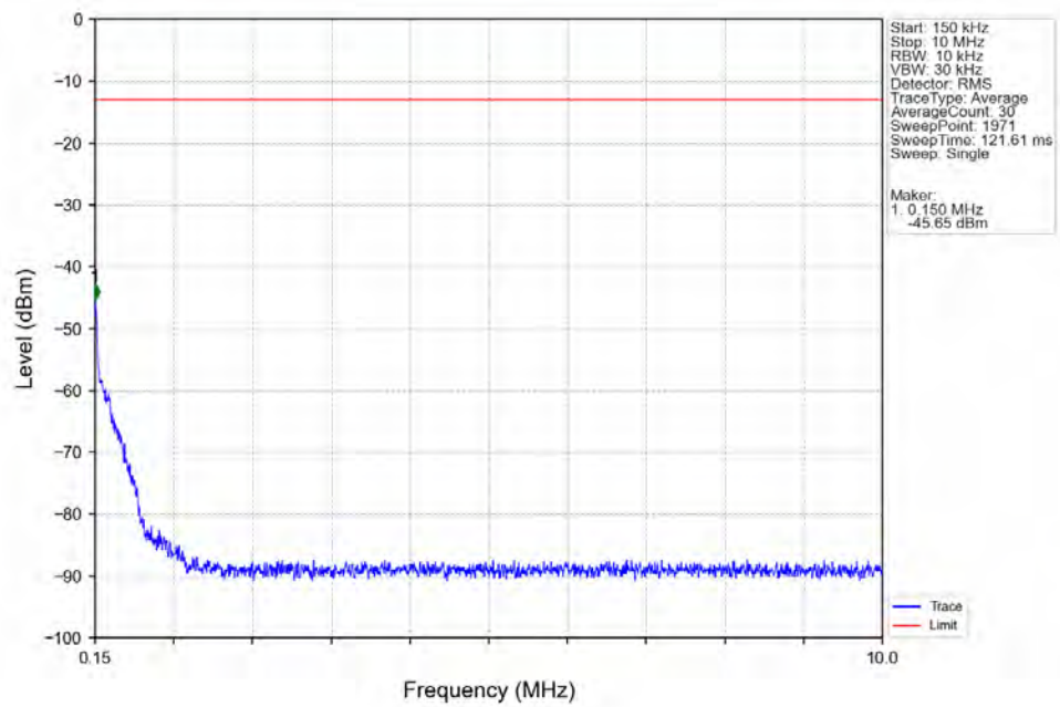
Band12_10MHz_QPSK_HCH_711MHz_RB_1_0_NTNV
